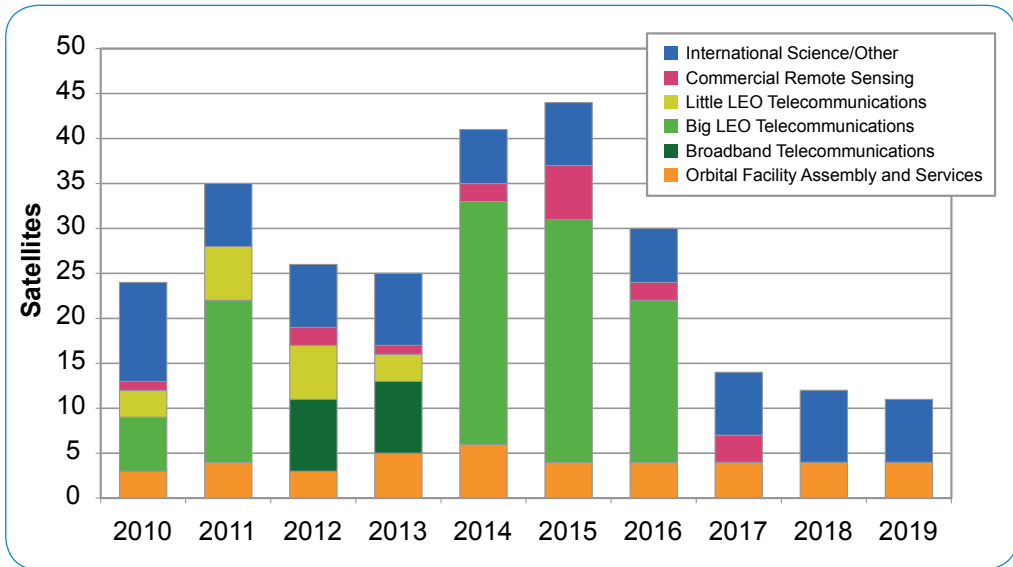
Figure 23. Satellite Forecast
