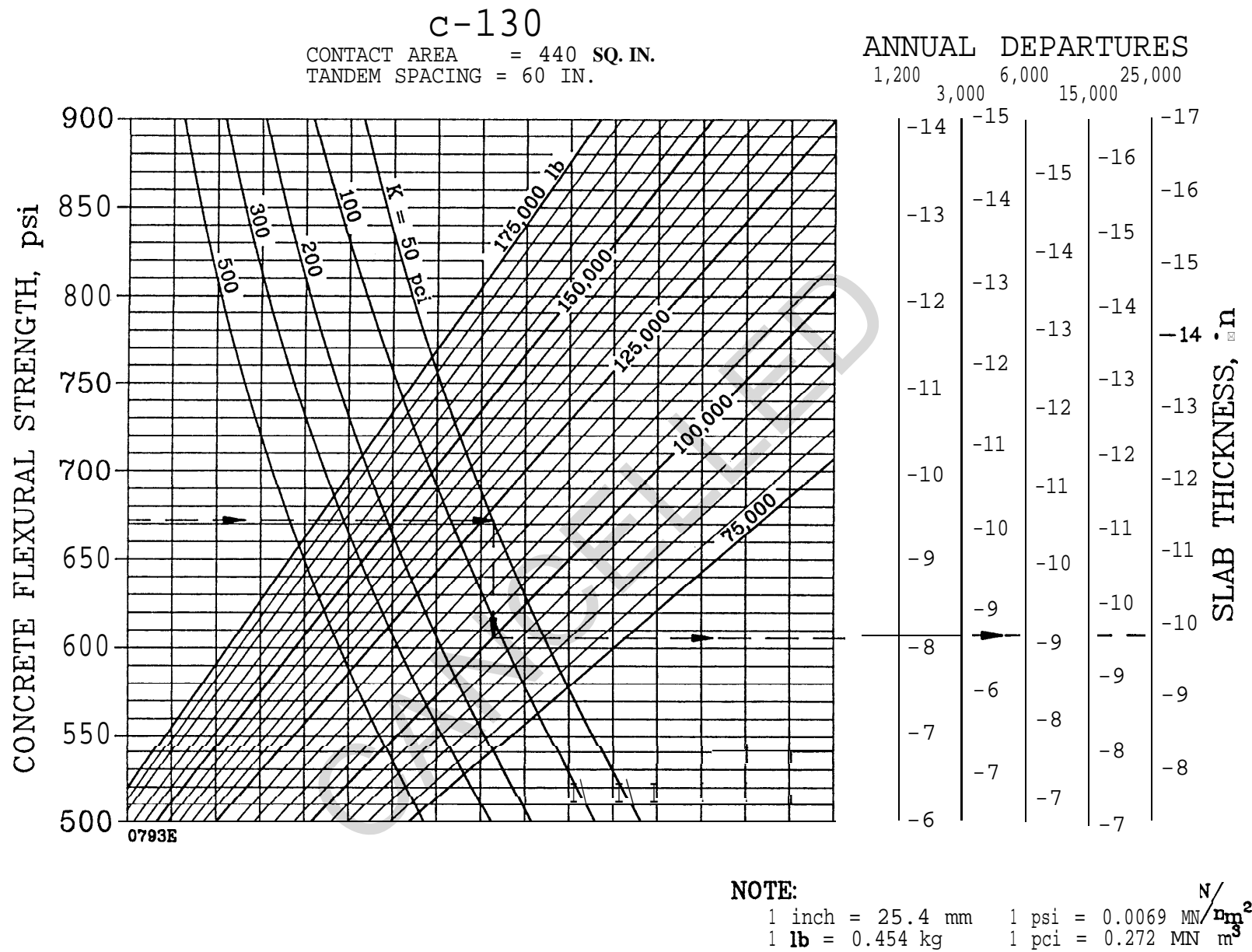
FIGURE 3-26. RIGID PAVEMENT DESIGN CURVES, C-130
