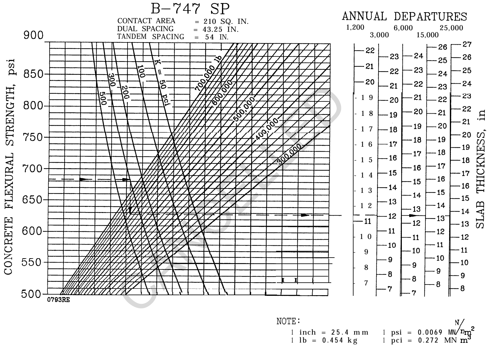
FIGURE 3-34. OPTIONAL RIGID PAVEMENT DESIGN CURVES, B-747-SP
