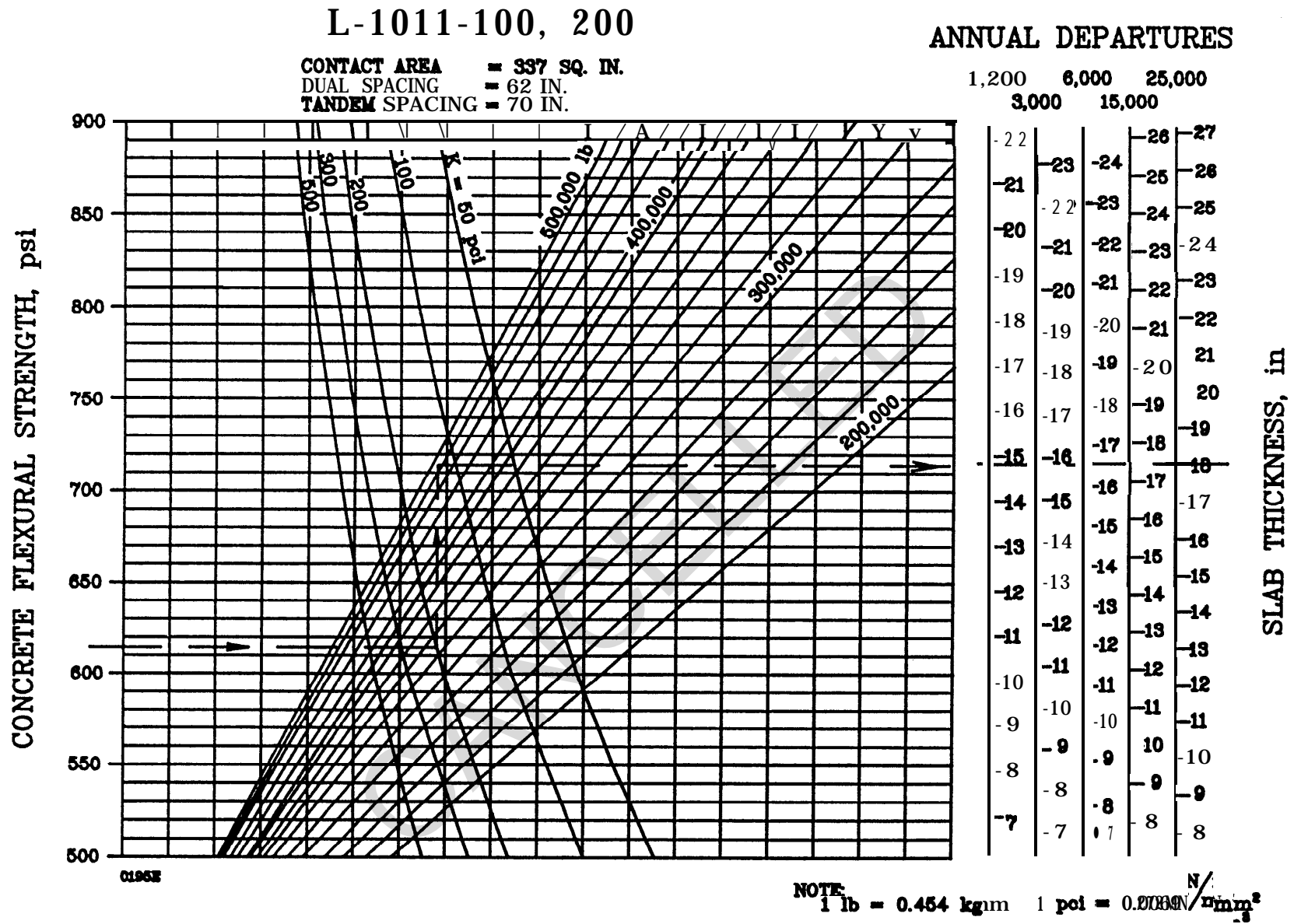
FIGURE 3-30. RIGID PAVEMENT DESIGN CURVES, L-1011-100,200
