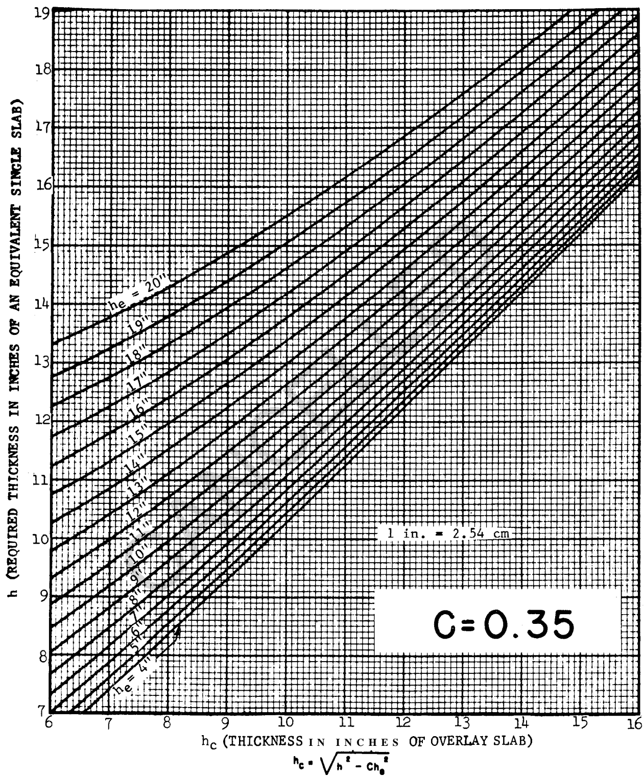
FIGURE 4-12. CONCRETE OVERLAY ON RIGID PAVEMENT
