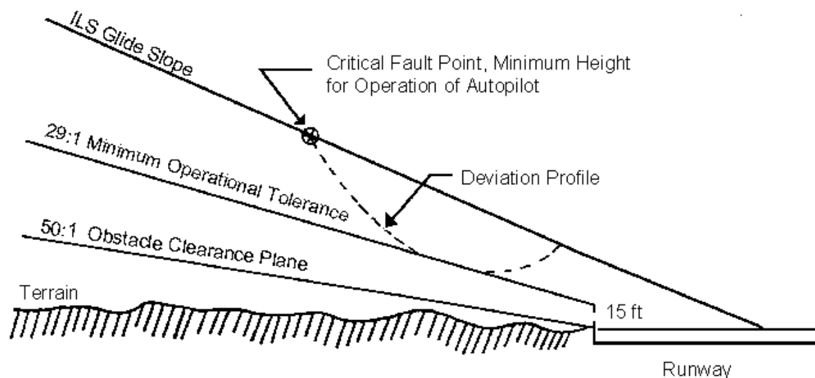
FIGURE AC 27.1329-2 OPERATIONAL LIMITATION
