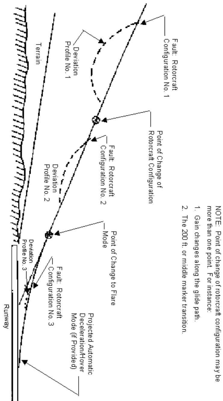
FIGURE AC 27.1329-1 DEVIATION PROFILE
