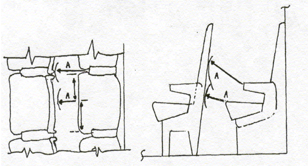
FIGURE AC 27.562-5
