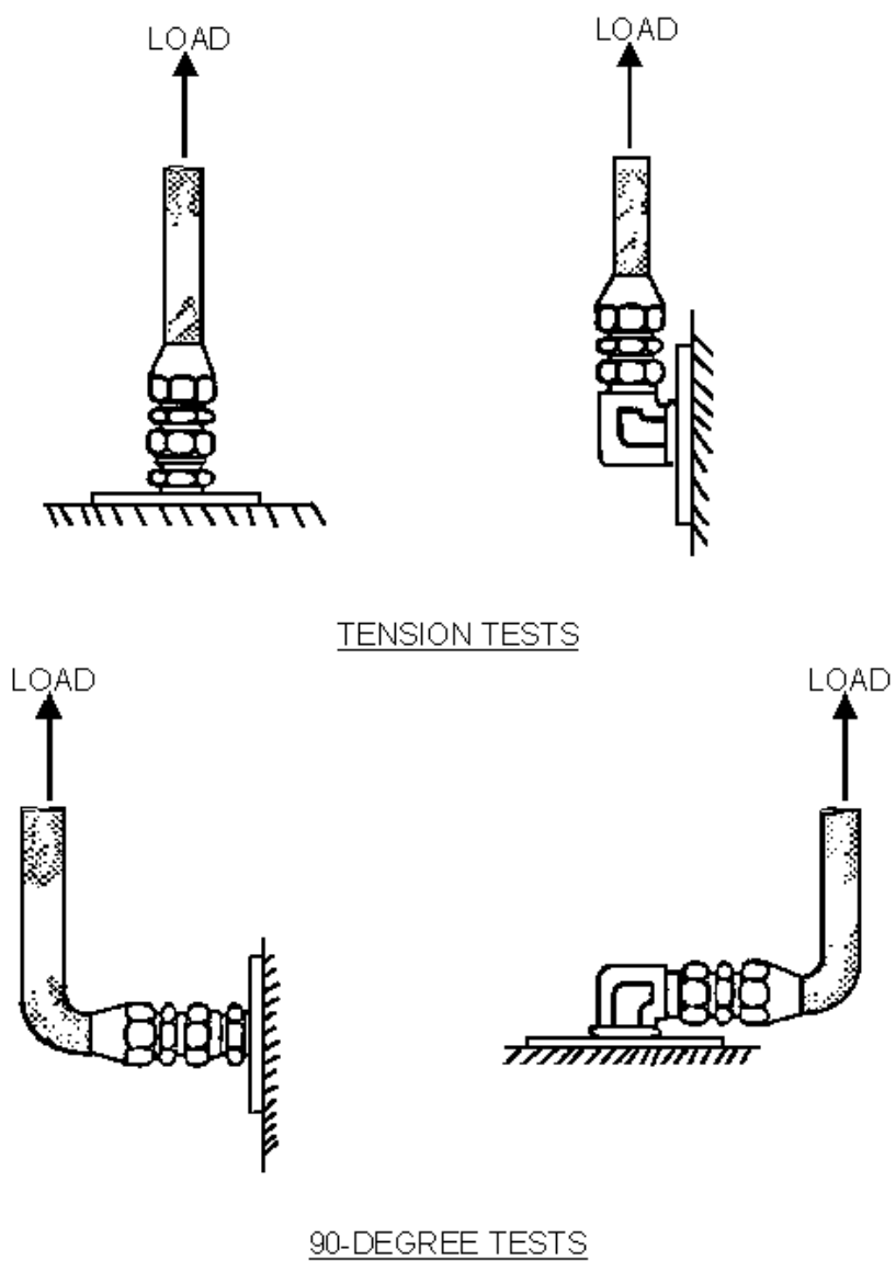
FIGURE AC 27.952-2 HOSE ASSEMBLY TESTS
