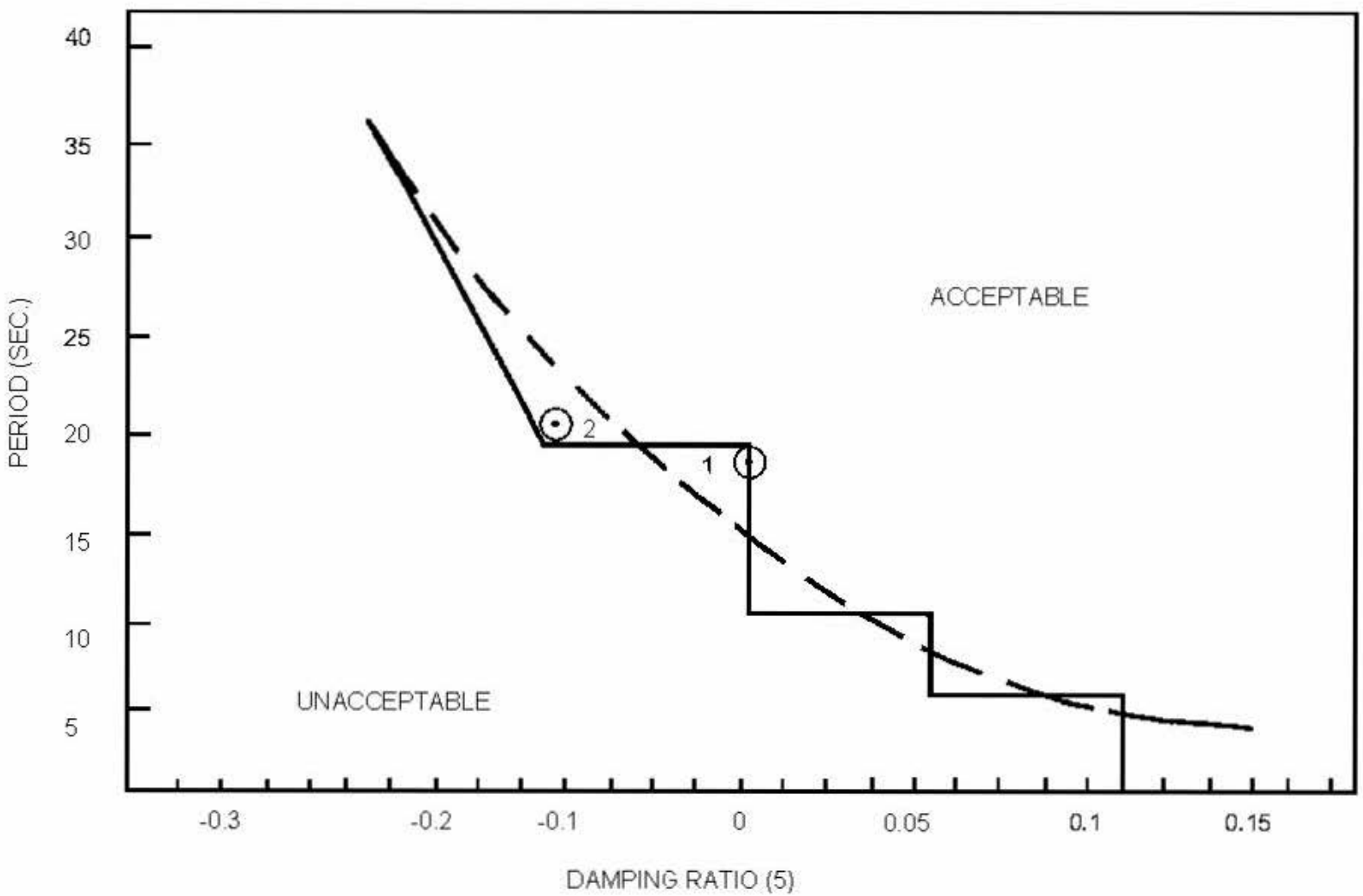
FIGURE AC 27-1B-1 ROTORCRAFT DYNAMIC STABILITY REQUIREMENTS FOR IFR
