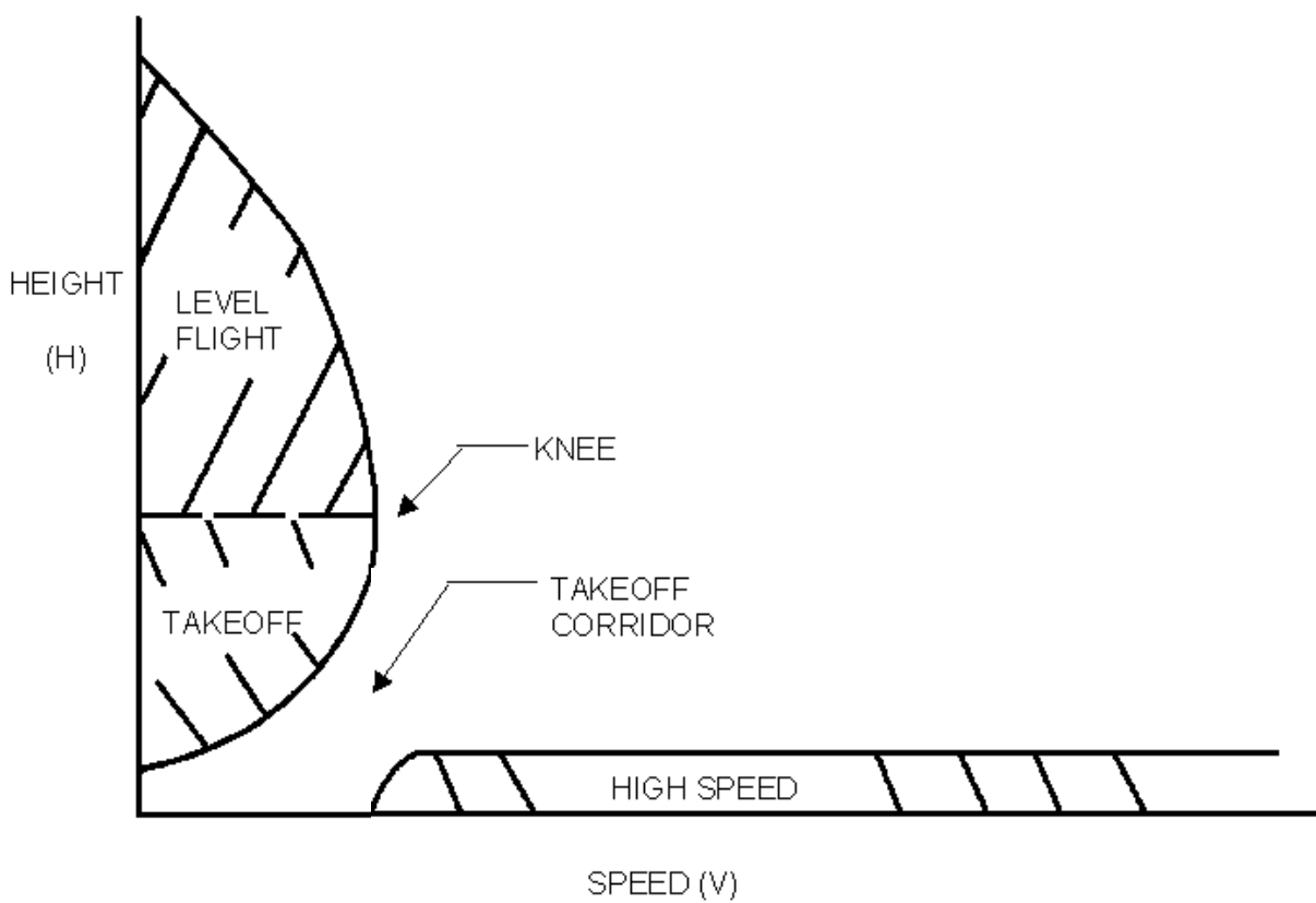
FIGURE AC 27.79-1 HEIGHT-VELOCITY (HV) DIAGRAM
