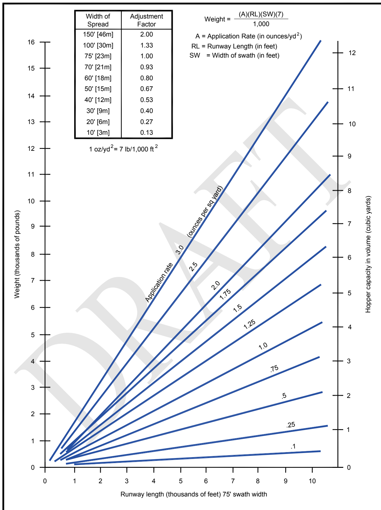
Figure 2—9. Hopper capacity – urea
