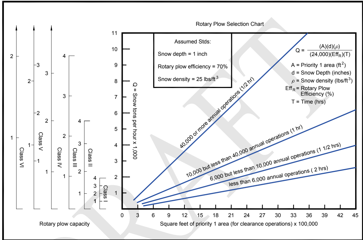
Figure 2—2. High-speed rotary plow calculations for airports with commercial service
