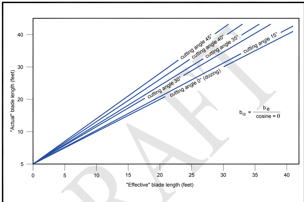
Figure 2—7 Effective versus actual snow plow blade length
