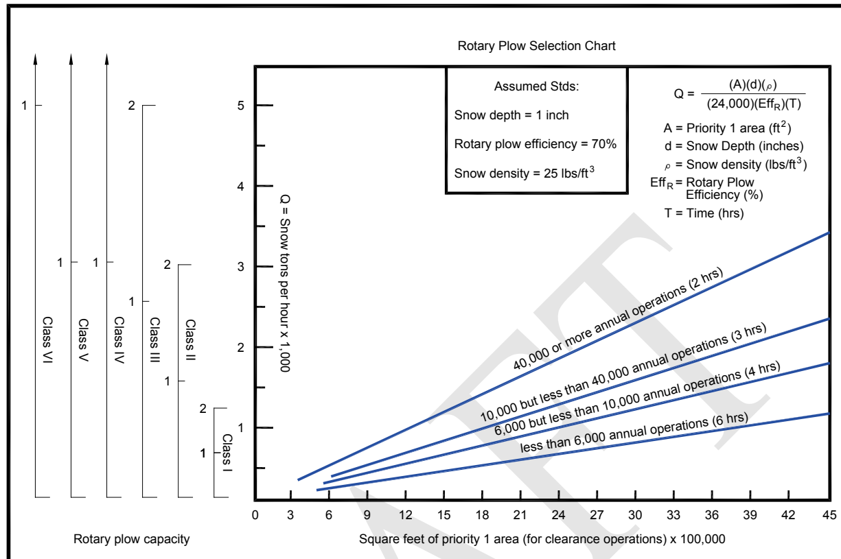
Figure 2—3. High-speed rotary plow calculations for airports with non-commercial service
