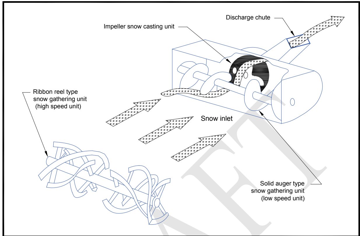
Figure 3—2. Two-stage rotary plow
