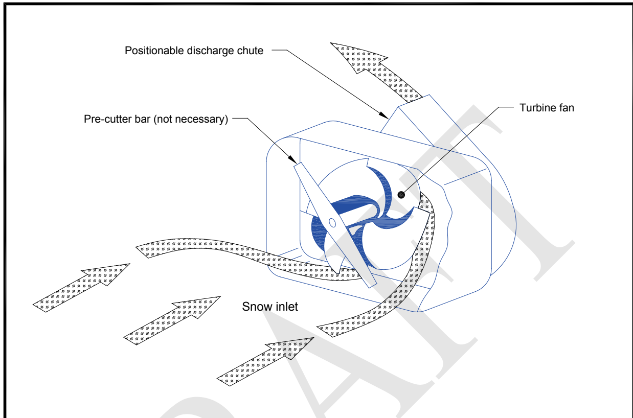
Figure 3—1. Single-stage rotary plow
