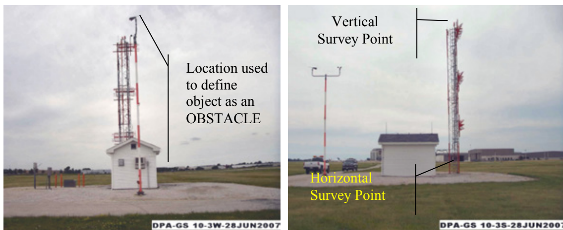
Figure 2-4. Illustrates the Documentation of a Glideslope Antenna from Different Perspectives
