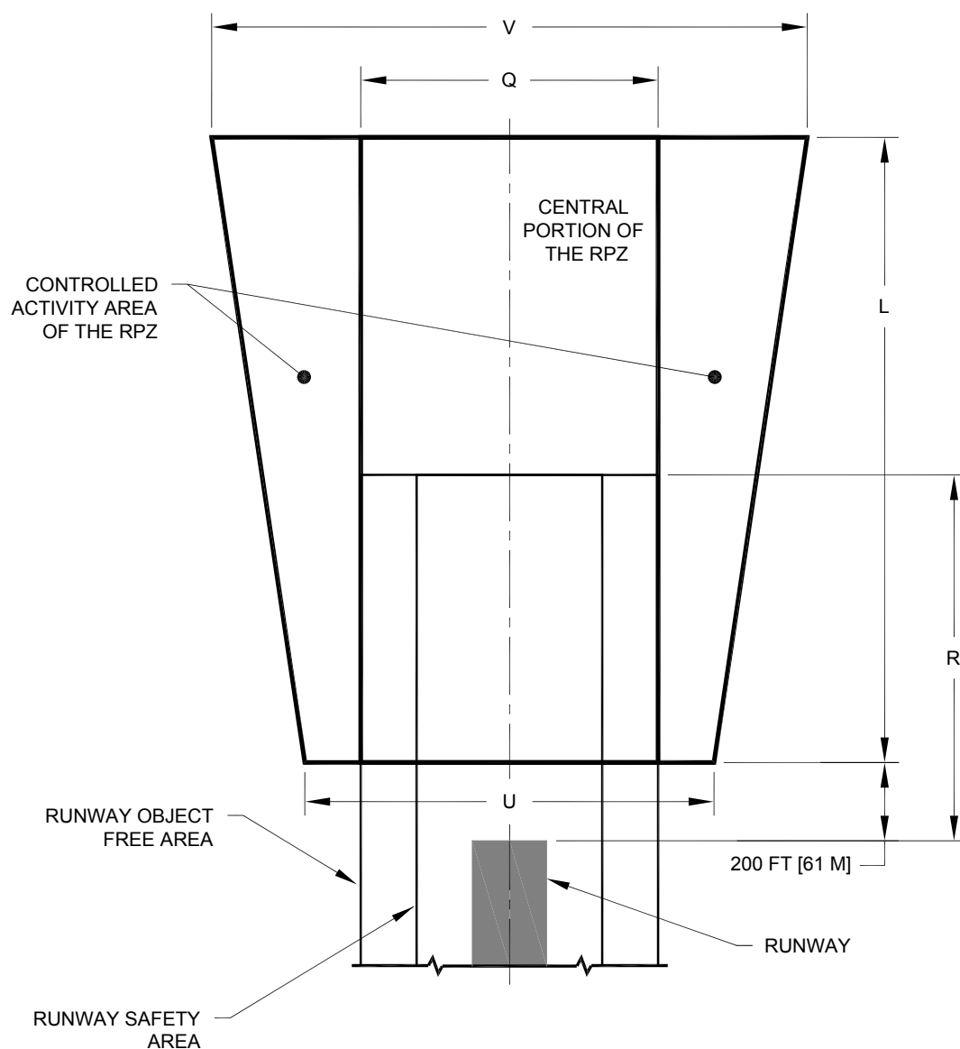
Figure 5-45. Runway Protection Zone (RPZ), Runway Object Free Area (ROFA) and Runway Safety Area (RSA)
