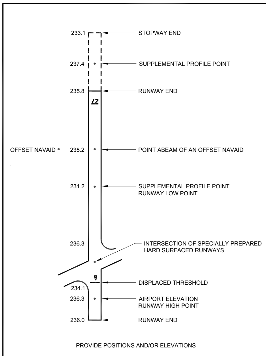
1524 Figure 2-6. Depicts Some of the Required Points and Elements of a Runway or Stopway
