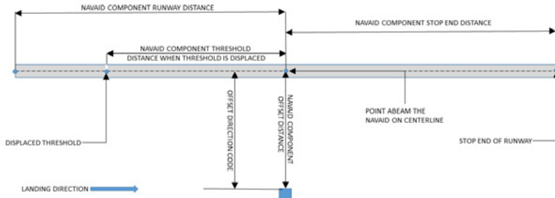
Figure 2-11. Shows the Required Measurements for a Navigational Aid
