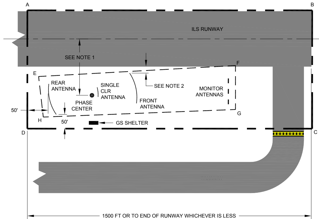
Figure 5-70. NAVAID Critical Area Example
