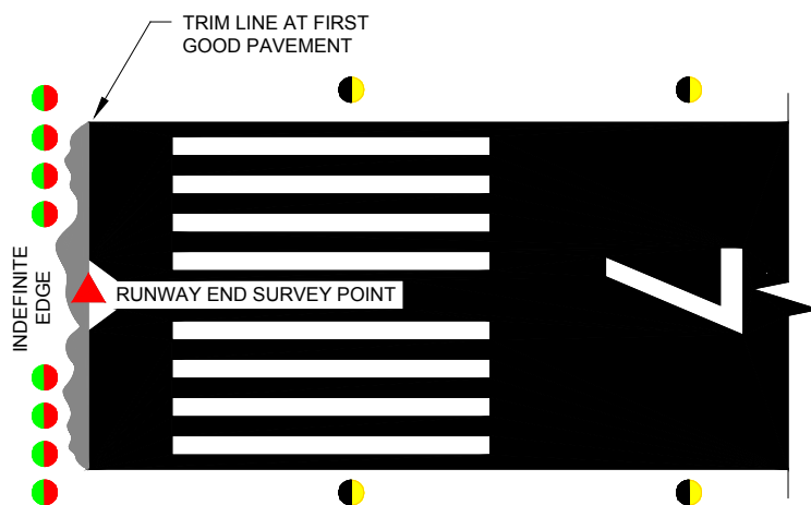
Figure 5-31. Runway End Survey Point
