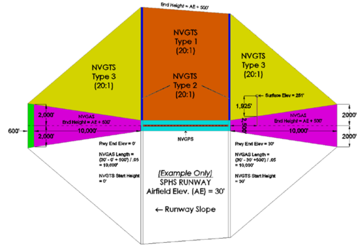
Figure 2-21. NVGPS, NVGAS, and NVGTS Types 1/2/3 for Non-Vertically Guided (NVG) Airport Surfaces
