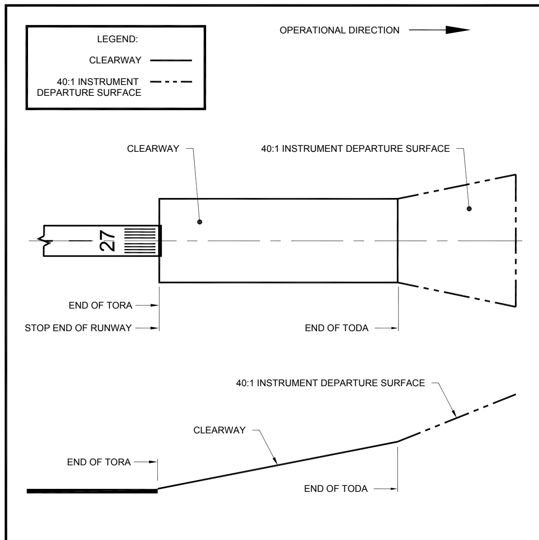
Figure 5-28. TODA extended by use of a clearway, normal TORA
