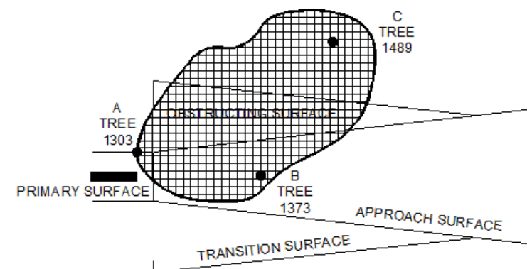
Figure 2-24. Reporting Highest Object(s) within Object Area Limits
