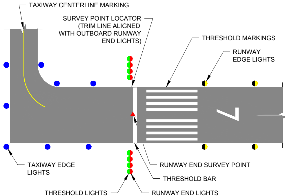
Figure 5-11. Paved Runway and Aligned Taxiway
