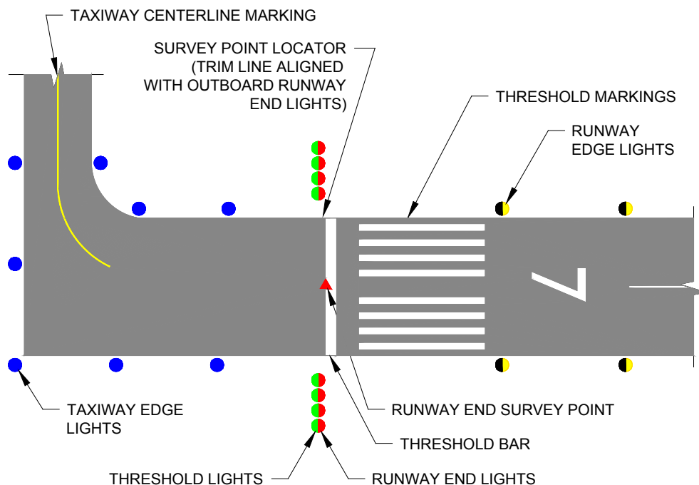
Figure 5-36. Paved Runway and Aligned Taxiway
