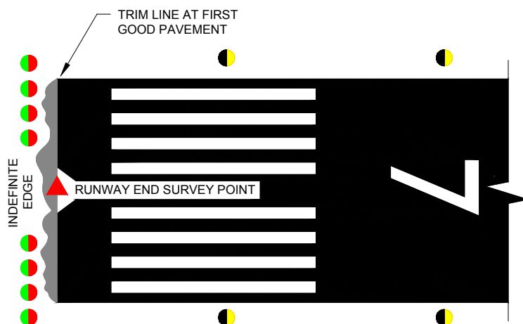
Figure 5-6. Runway End Survey Point
