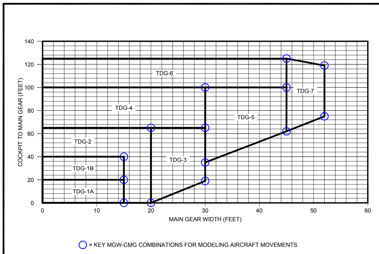
Figure 4-17. Key MGW-CMG combinations for modeling aircraft movements
