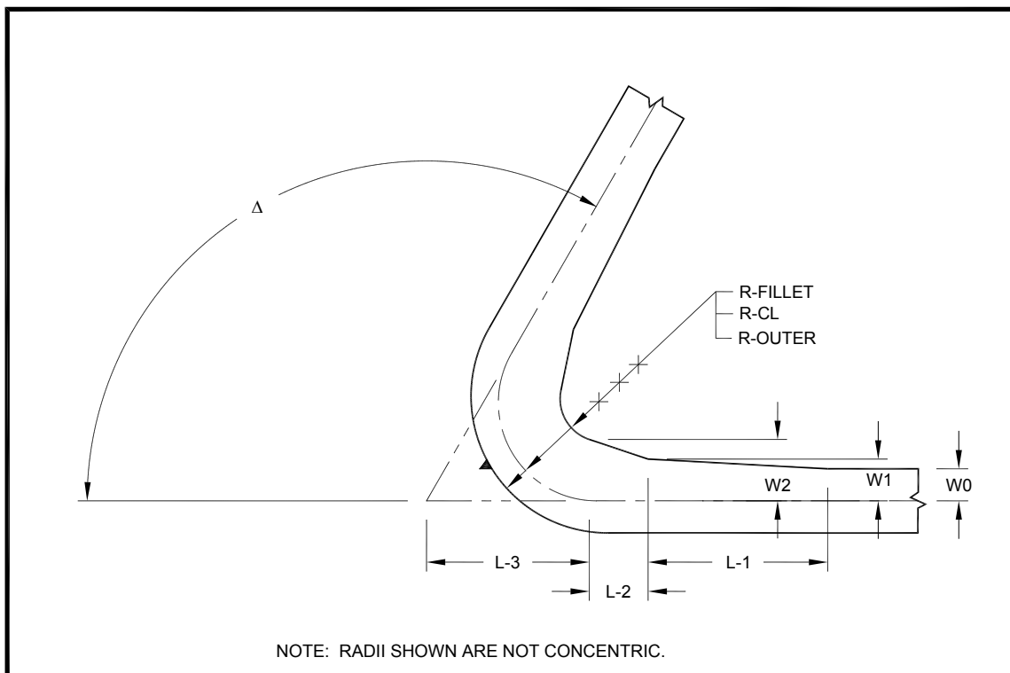
Figure 4-16. Greater than 90 degree delta
