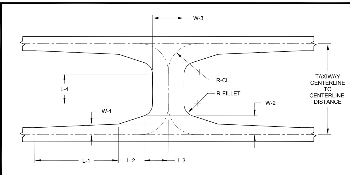
Figure 4-24. Crossover taxiway where direction reversal is needed based on TDG
