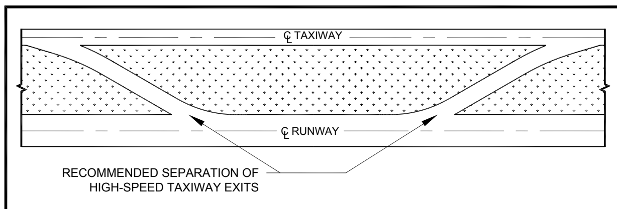
Figure 4-22. Proper design of high speed exits
