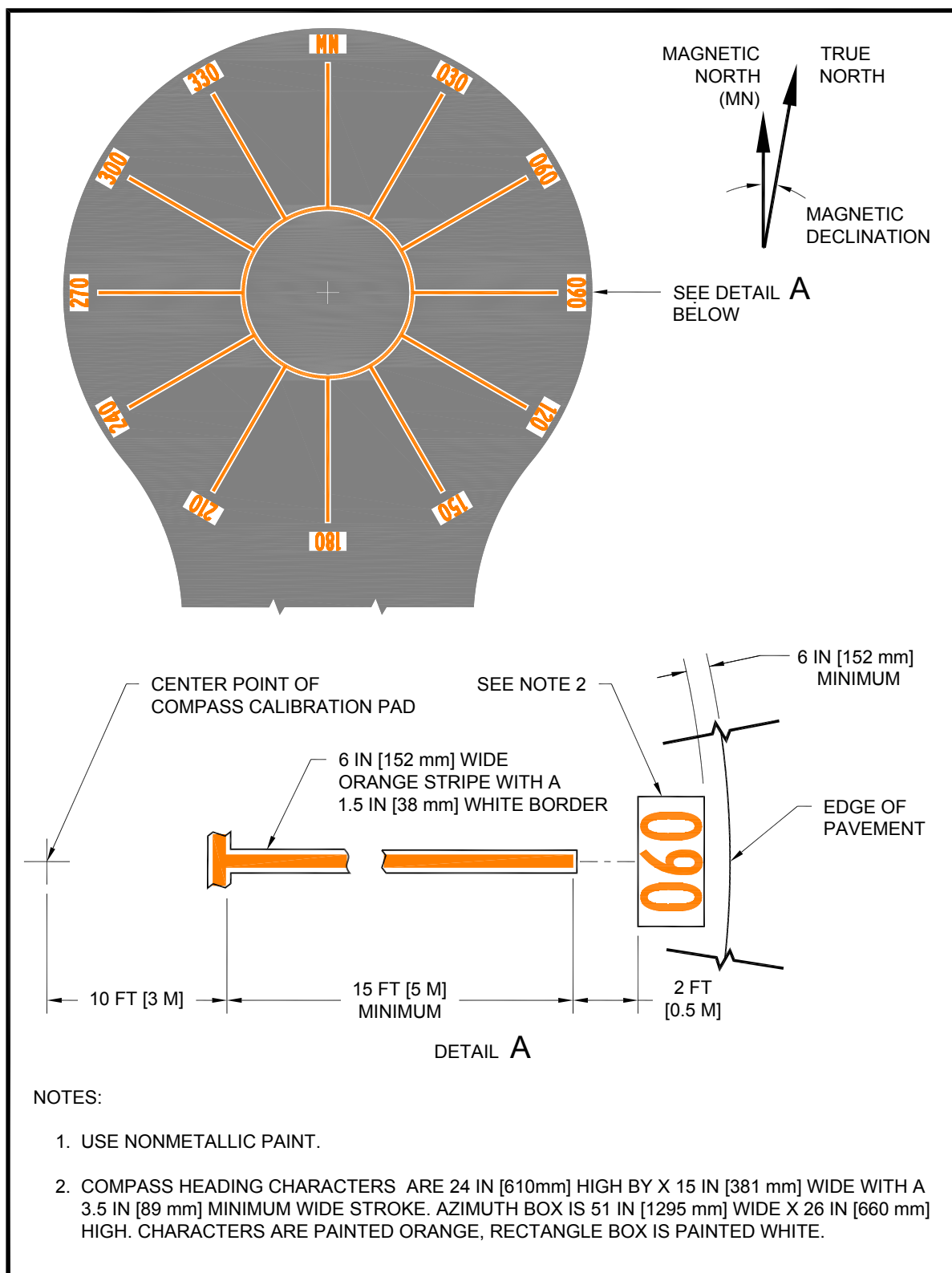
Figure A6-1. Compass calibration pad marking layout
