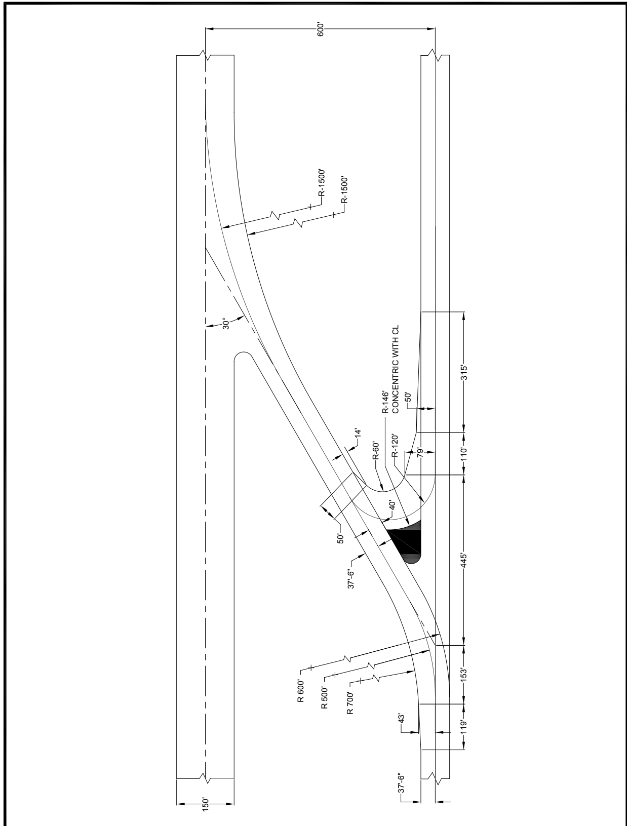
Figure 4-19. High speed exit for TDG-5
