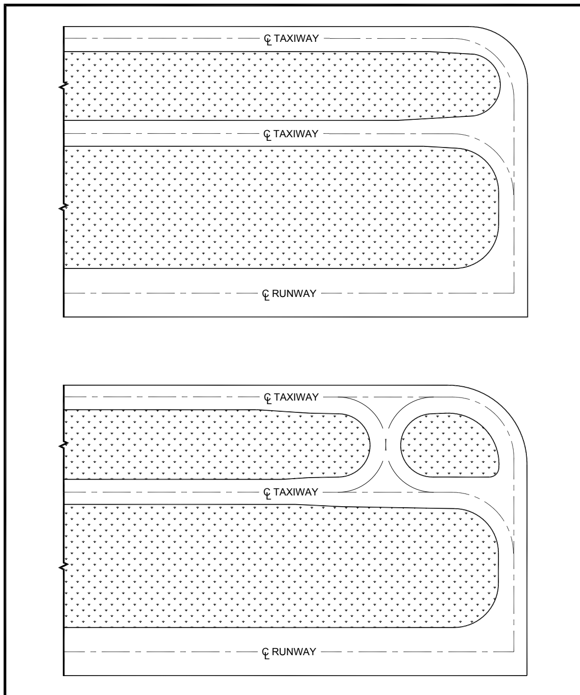
Figure 4-13. Parallel taxiways
