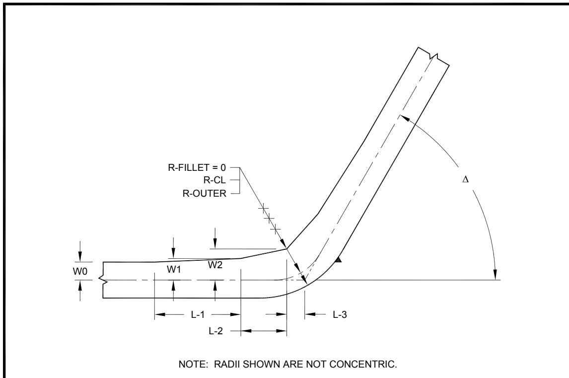
Figure 4-15. Less than 90 degree delta
