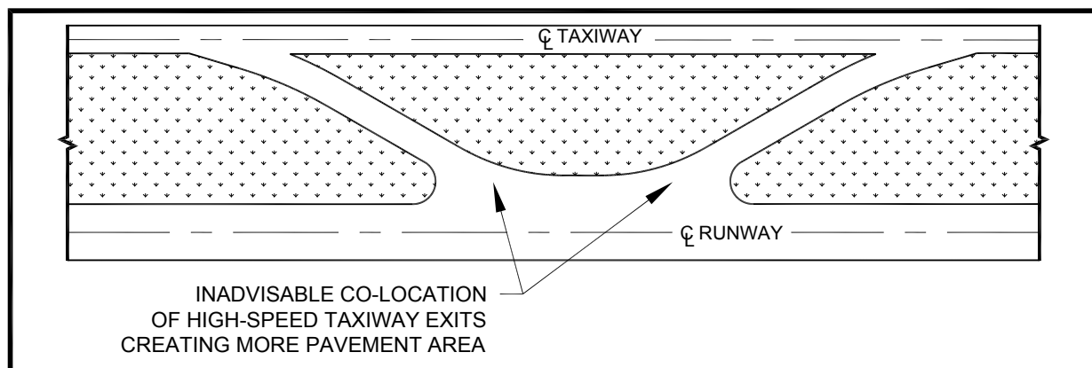
Figure 4-21. Poor design of high speed exits
