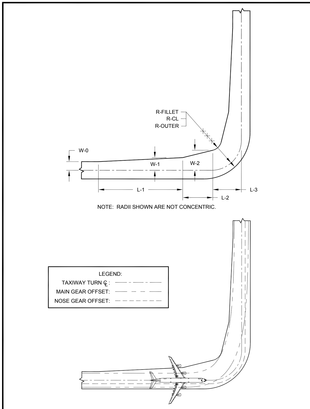
Figure 4-14. Taxiway turn
