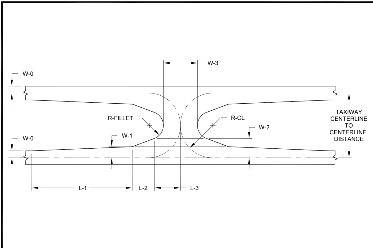
Figure 4-24. Crossover taxiway where direction reversal is needed based on TDG
