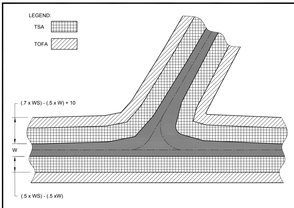
Figure 4-12. TSA and TOFA at taxiway intersections
