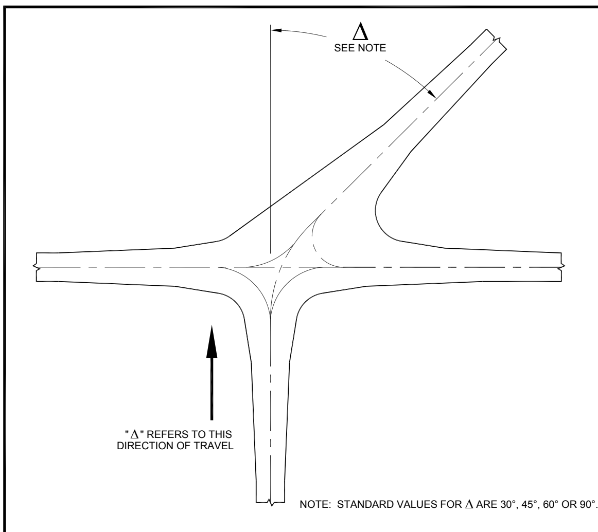
Figure 4-2. Three-node taxiway intersection
