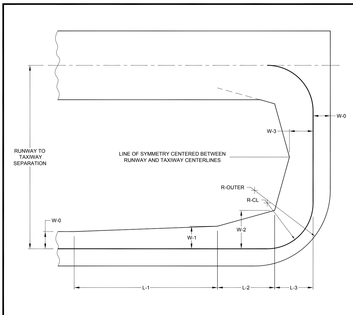
Figure 4-18. Entrance taxiway
