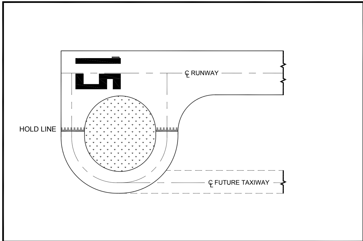
Figure 4-31. Taxiway turnaround
