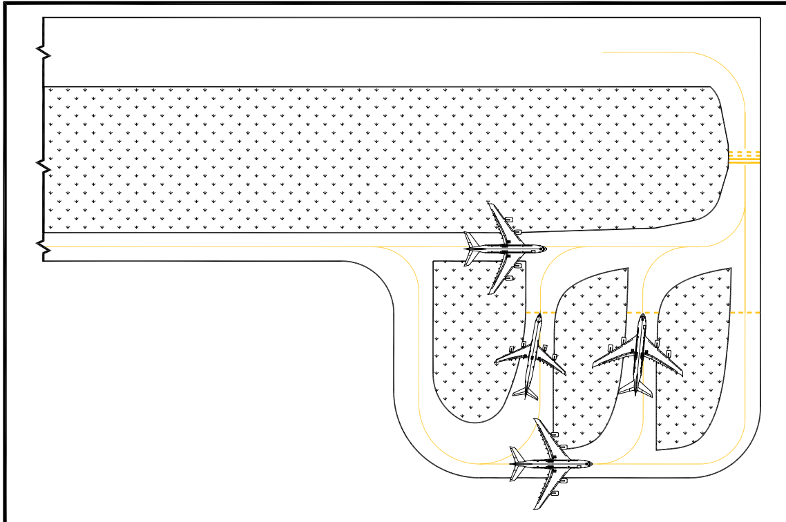
Figure 4-28. Typical holding bay configuration
