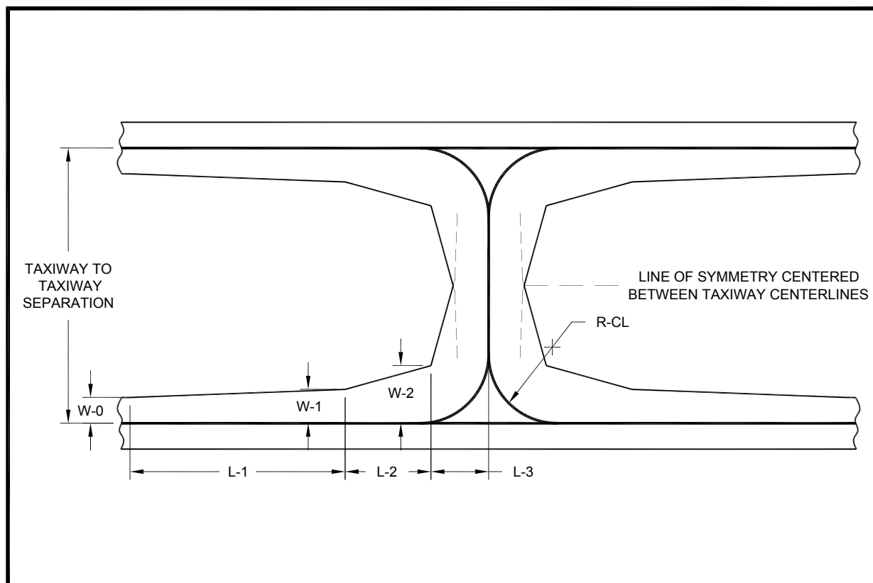
Figure 4-26. Crossover taxiway without direction reversal between taxiways
