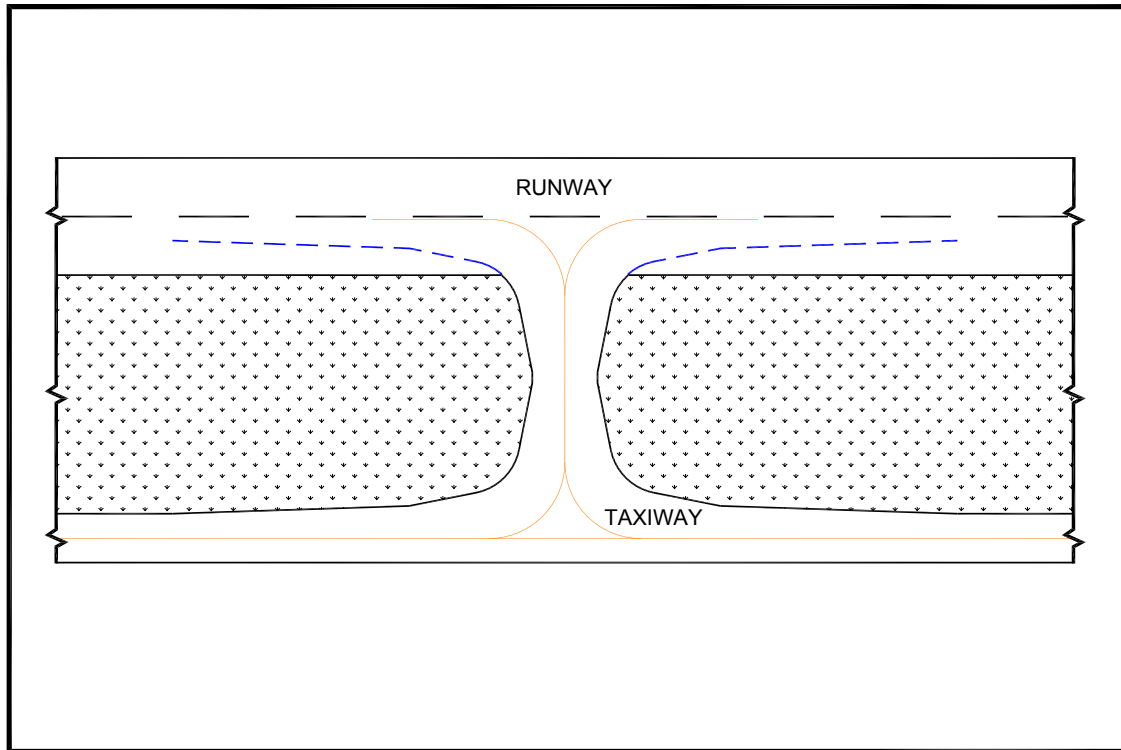
Figure 4-20. Right-angled exit taxiway
