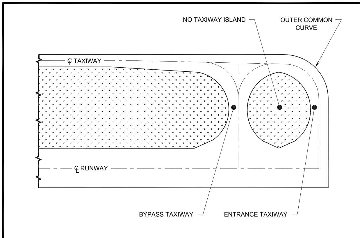
Figure 4-23. Bypass taxiway
