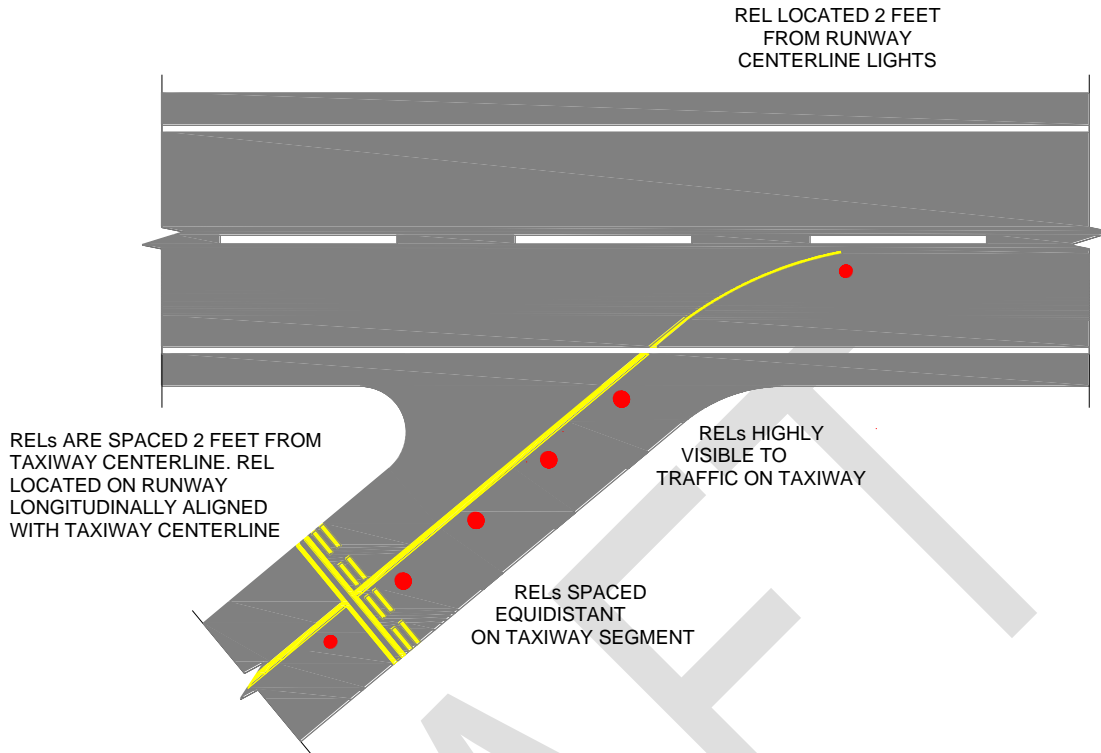
Figure 144. Angled Configuration
