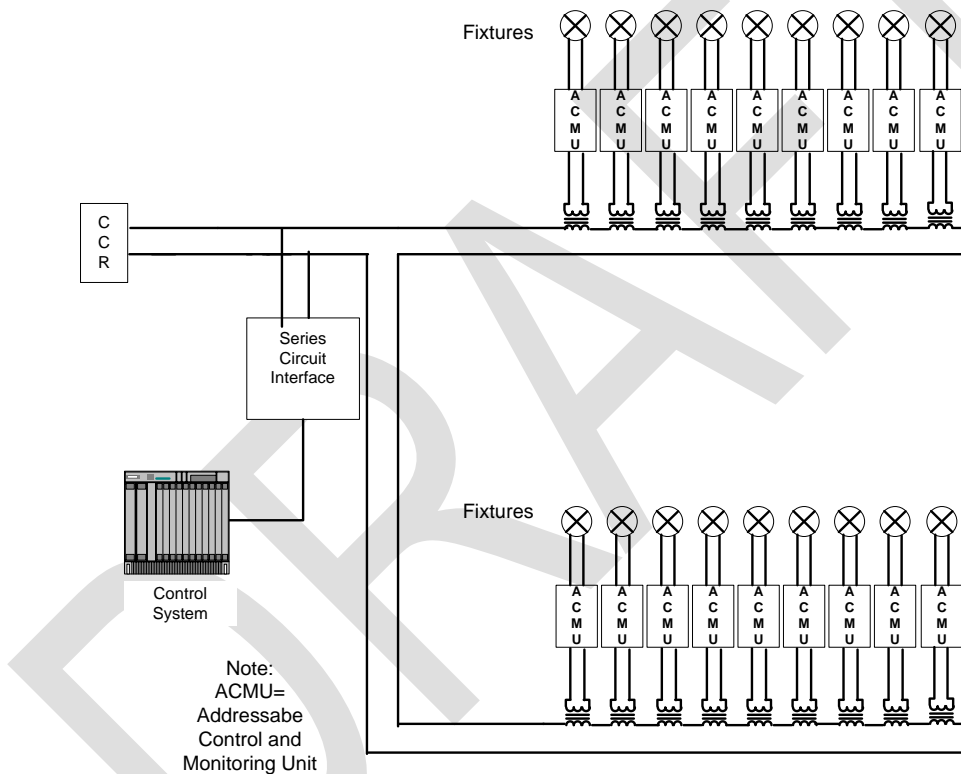
Figure 140. Typical Power Line Carrier System
