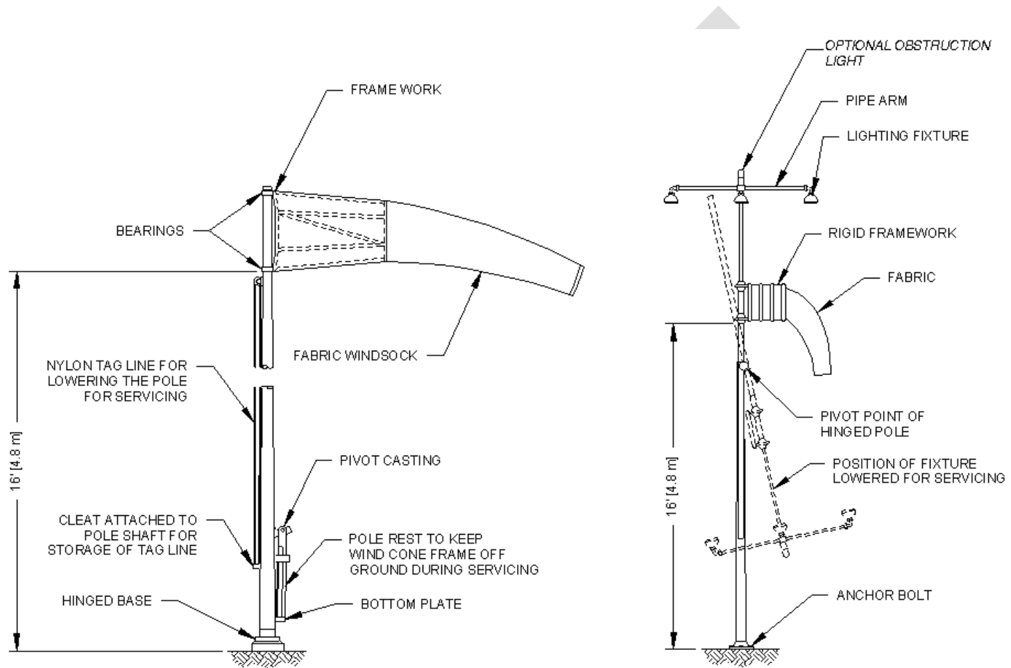
Figure 2. Typical Type L-807 supports
