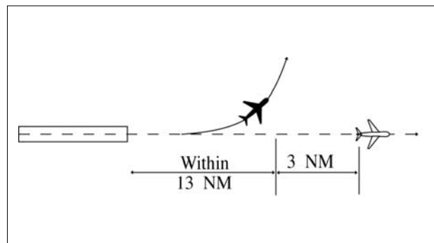
Minima on Diverging Courses
