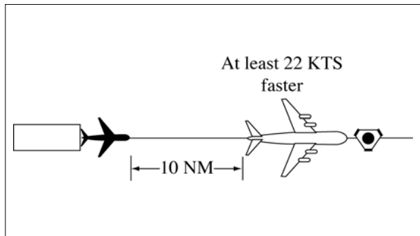
FIG 6-4-4 Minima on Same Course 22 Knots or More Separation
