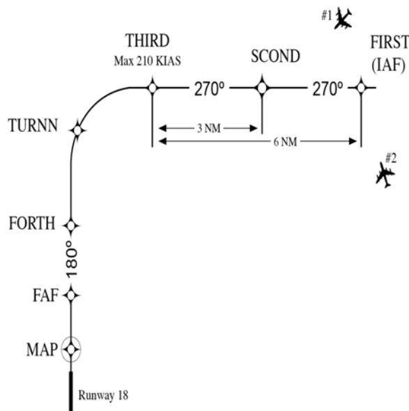
FIG 4-8-4 Radius to Fix (RF) and Track to Fix (TF)
