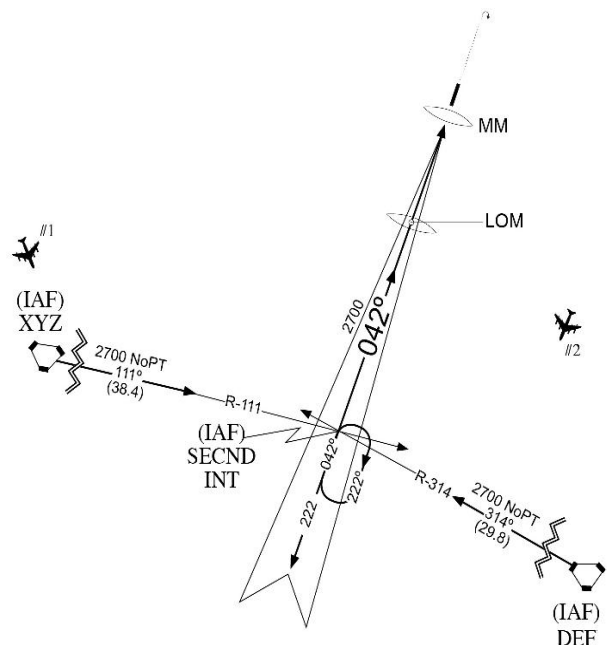
FIG 4-8-3 Approach Clearance Example for RNAV Aircraft On a Conventional Approach
