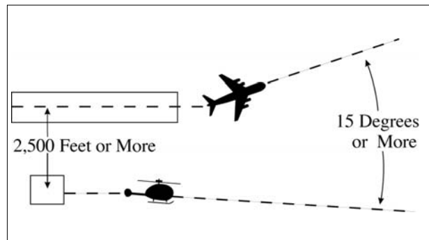
FIG 5-8-8 Parallel Helicopter Course Departures
