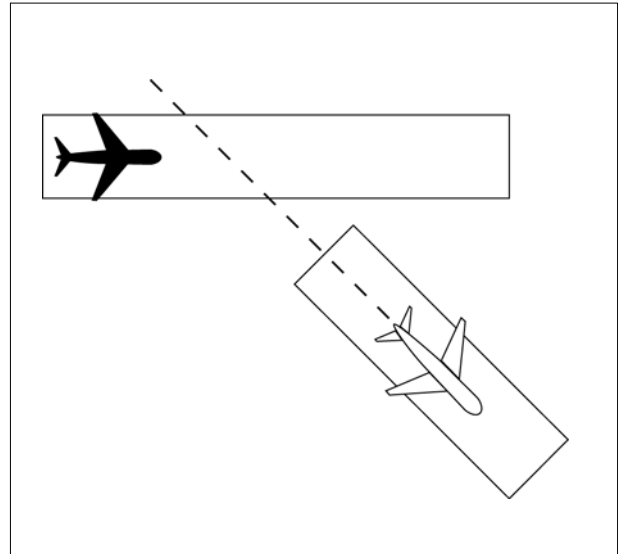
FIG 3-9-8 Intersecting Runway Separation
