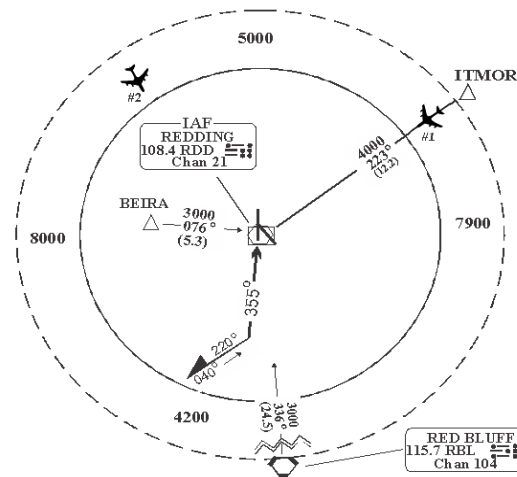
FIG 4–8–1 Approach Clearance Example
