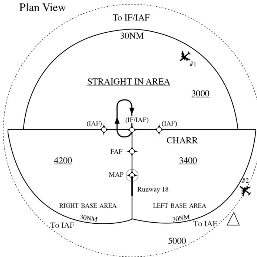
FIG 4-8-5 Basic "T" and TAA Design
