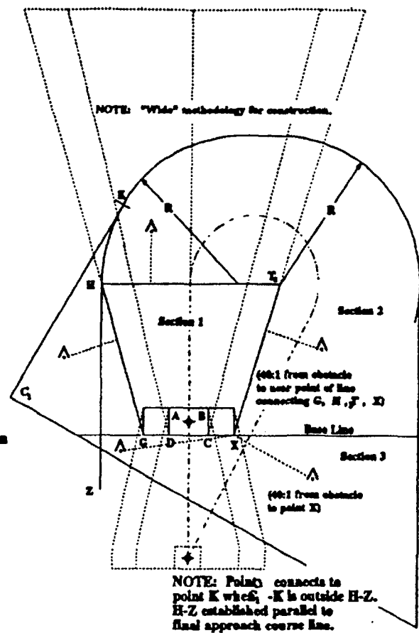
Figure 15-36. CLIMB TO ALTITUDE, STRAIGHT AND TURNING MISSED APPROACH > 180^\circ . Par 1535a(3).
