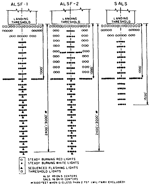
Figure 134 APPROACH LIGHTING SYSTEMS.
