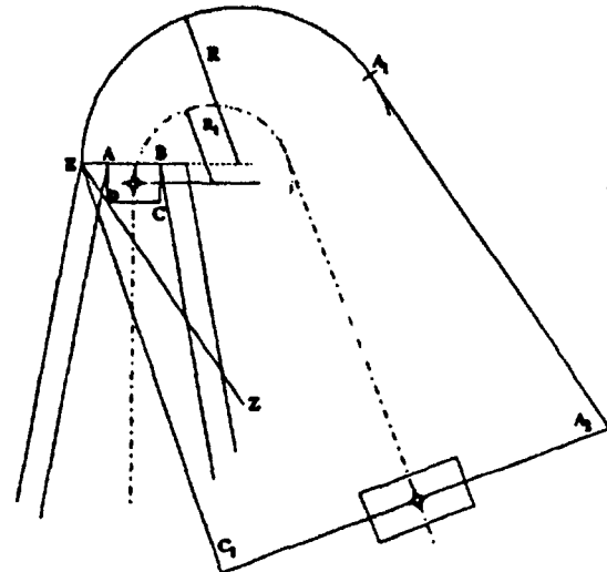
Figure 15-29. DIRECT TURNING MISSED APPROACH, > 90^\circ . Par 1534a(2)(b).
