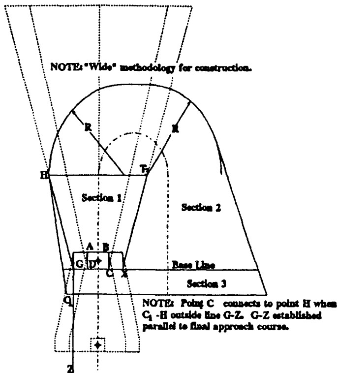
Figure 15-35. CLIMB TO ALTITUDE, STRAIGHT AND TURNING MISSED APPROACH > 90^\circ . Par 1535a(3).
