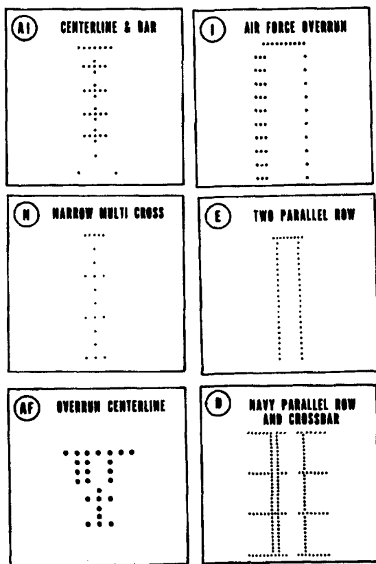
Figure 138. SYSTEMS EQUIVALENT TO SALS, SSALS, SSALF, MALS, AND MALSF.
