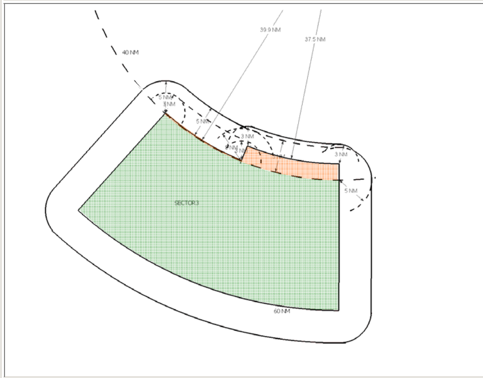
Figure 10-5a. Buffer Area, Contiguous Sector crossing 40 NM. (Single sensor,w/out reinforced MSSR)
