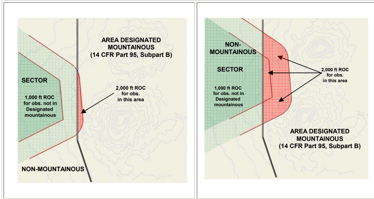
Figure 10-9. Sector/Buffer Overlaying Both Mountainous and Non-Mountainous Areas
