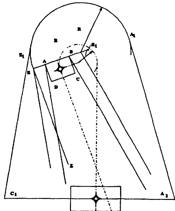
Figure 15-29. DIRECT TURNING MISSED APPROACH, > 90^\circ . Par 1534a(2)(b).
