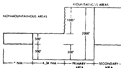
Figure 17-27 LF SEGMENT OBSTACLE CLEARANCE OVER 25 NM FROM ENROUTE FACILITY Par 1750 d
