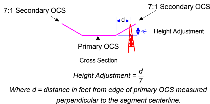
Figure 4-5. Secondary OCS Evaluation
