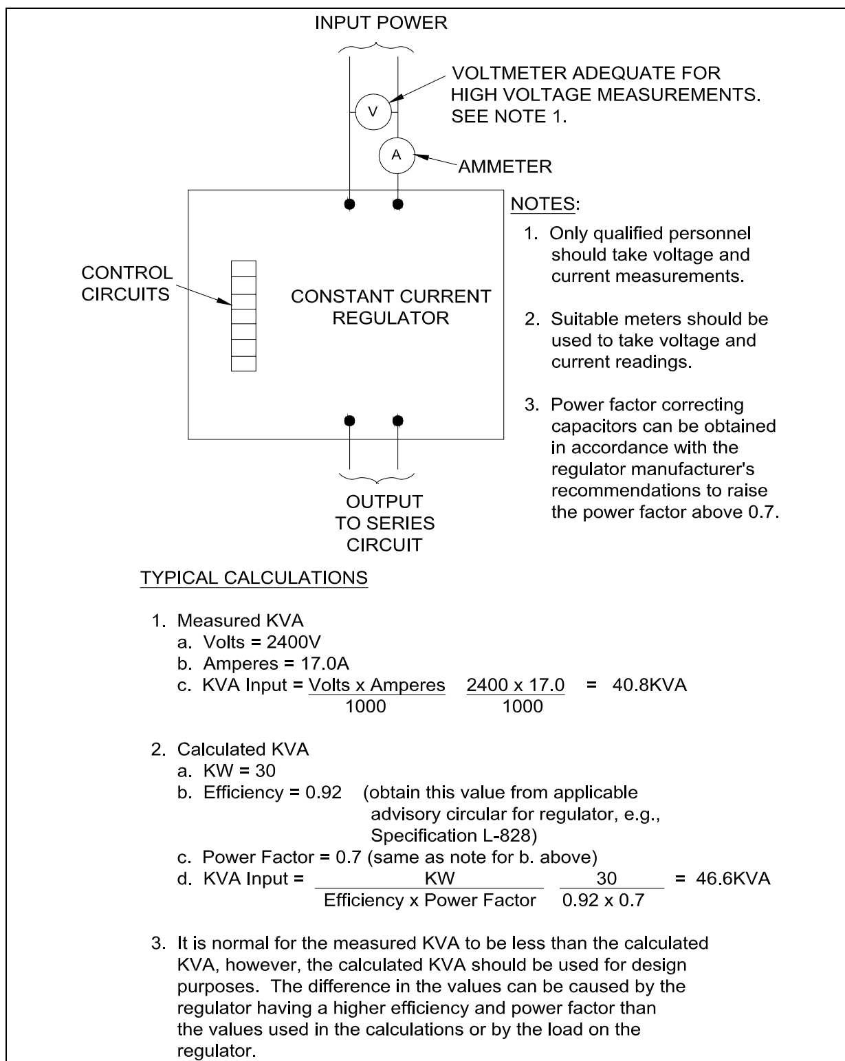
Figure 93. Typical KVA Input Requirements.
