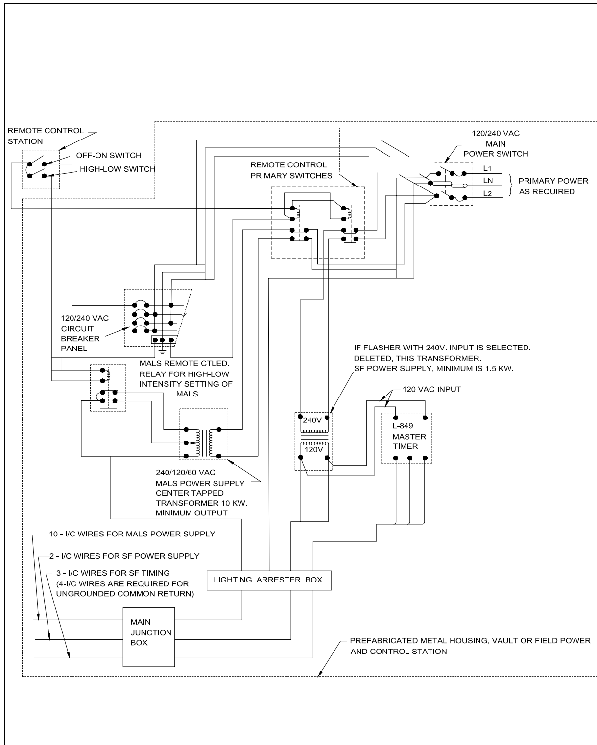
Figure 82. General Wiring Diagram for MALS with 120-Volt, AC Remote Control.
