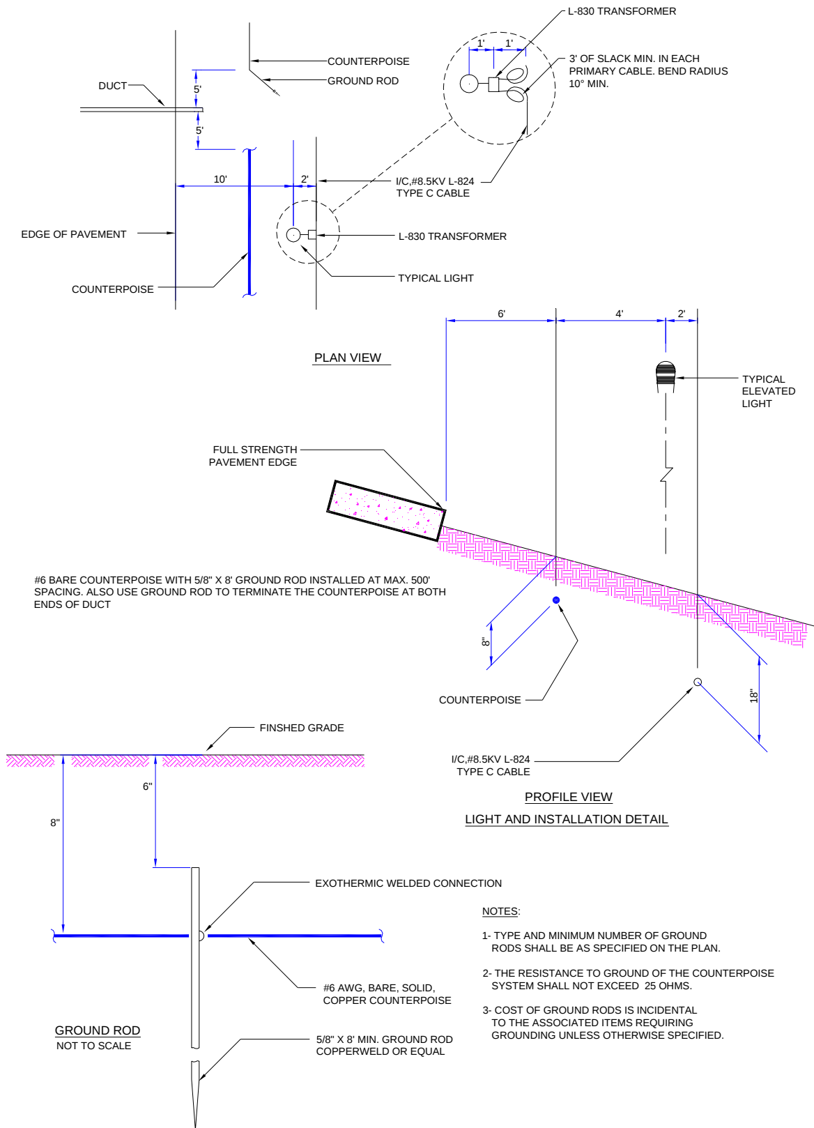
Figure 109. Counterpoise Installation.
