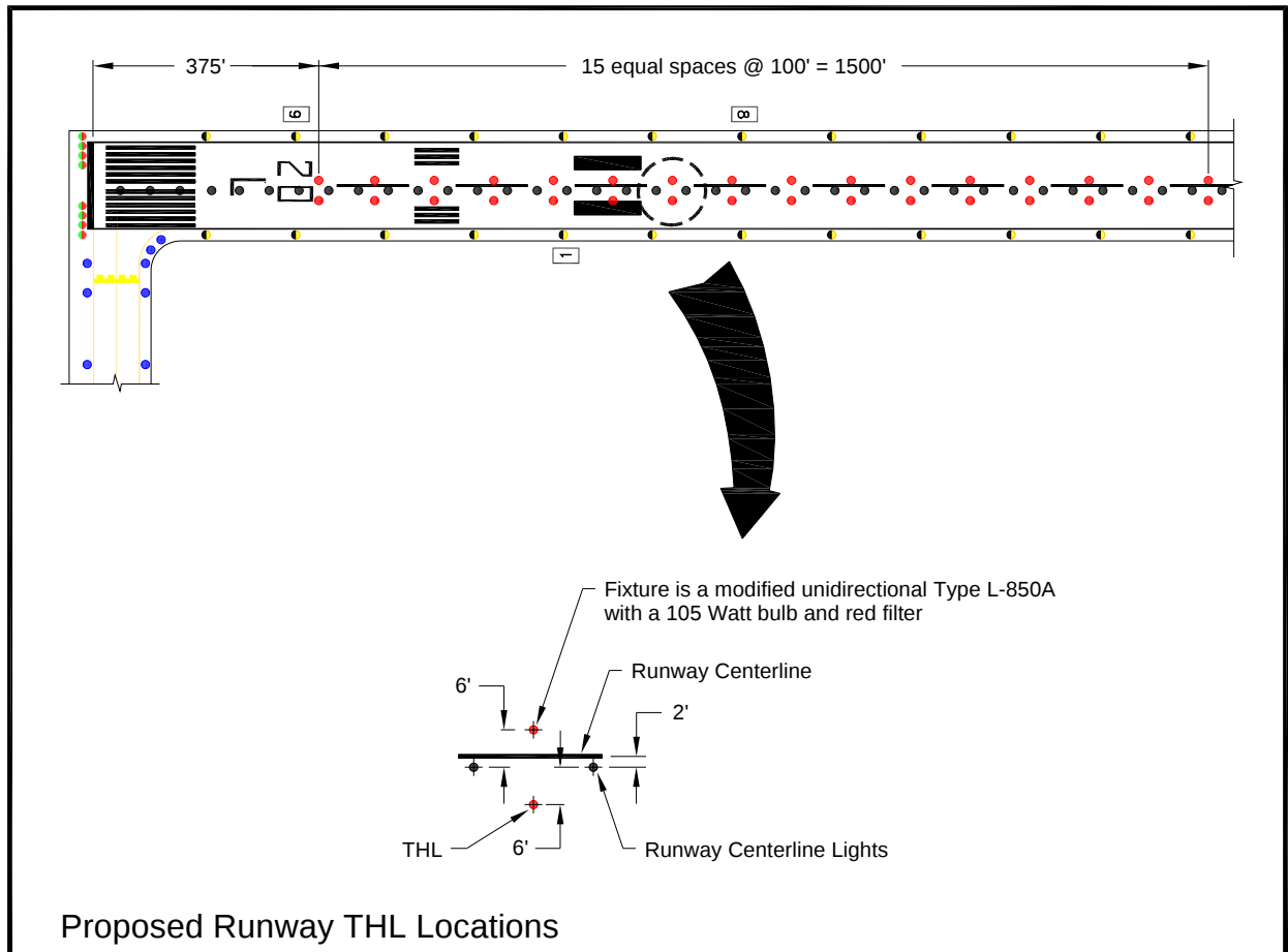
Figure 145. Takeoff/Hold Lights
