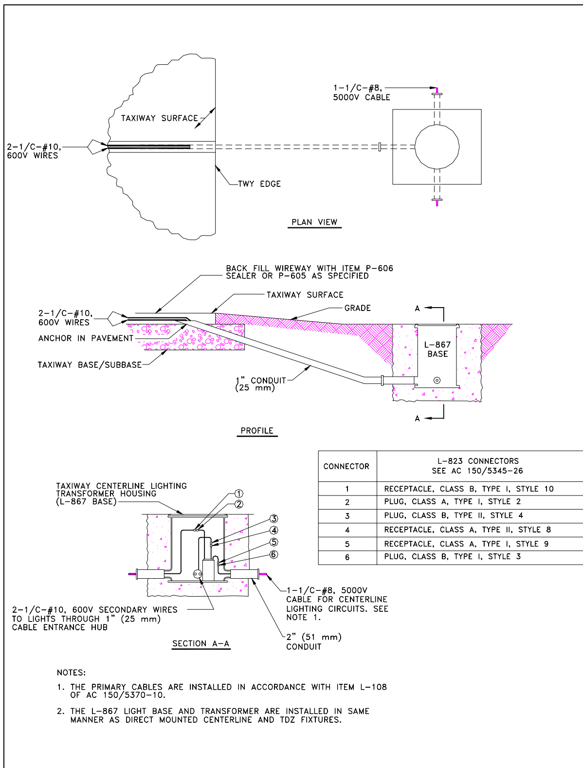
Figure 106. Typical Transformer Housing and Conduit Installation Details for Taxiway Centerline Lights.
