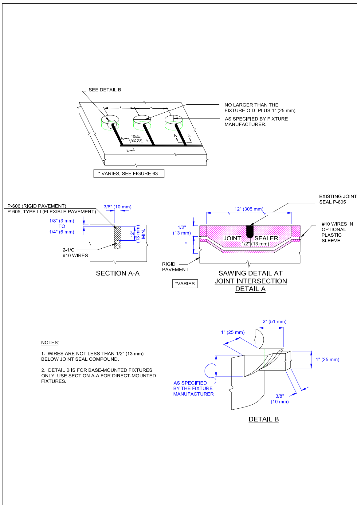
Figure 64. Sawing &amp; Drilling Details for In-pavement Land &amp; Hold Short Lights.
