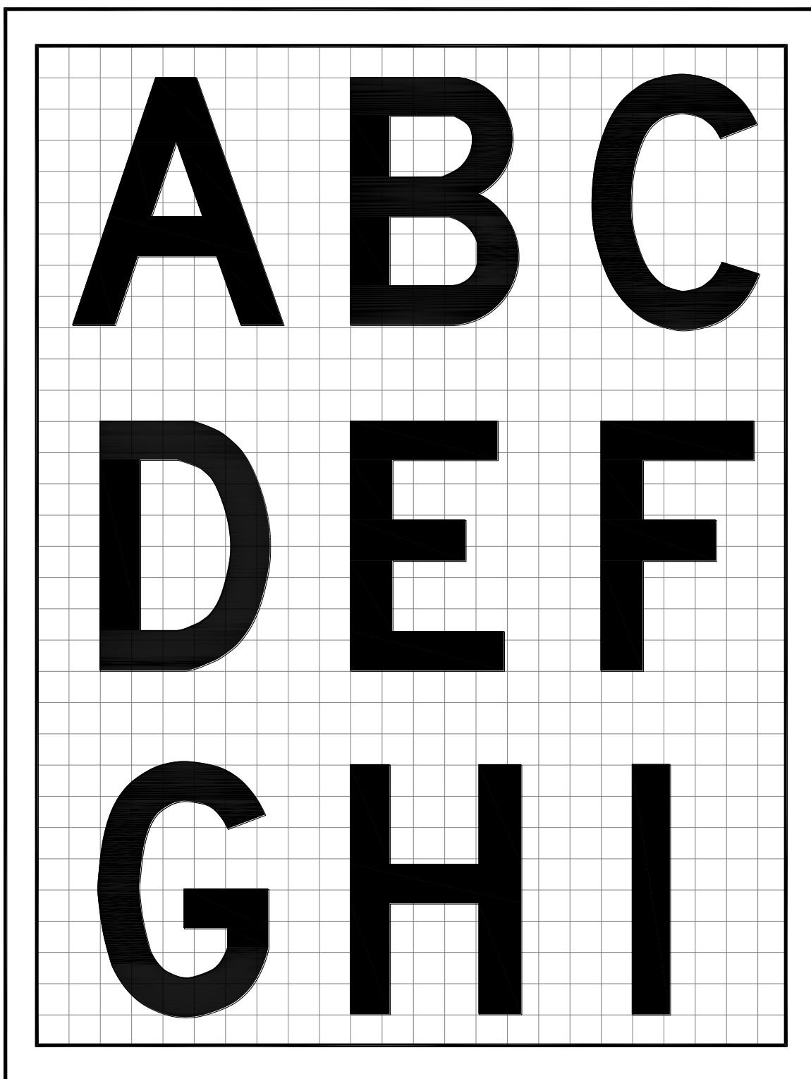
Figure 1. Sign Legend Characters for Size 1, 2, and 3 Signs, Types L-858Y, L-858R and L-858L
