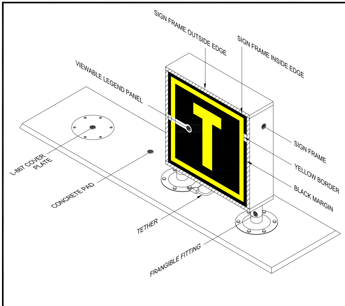
Figure 17. Typical Sign and Component Parts
