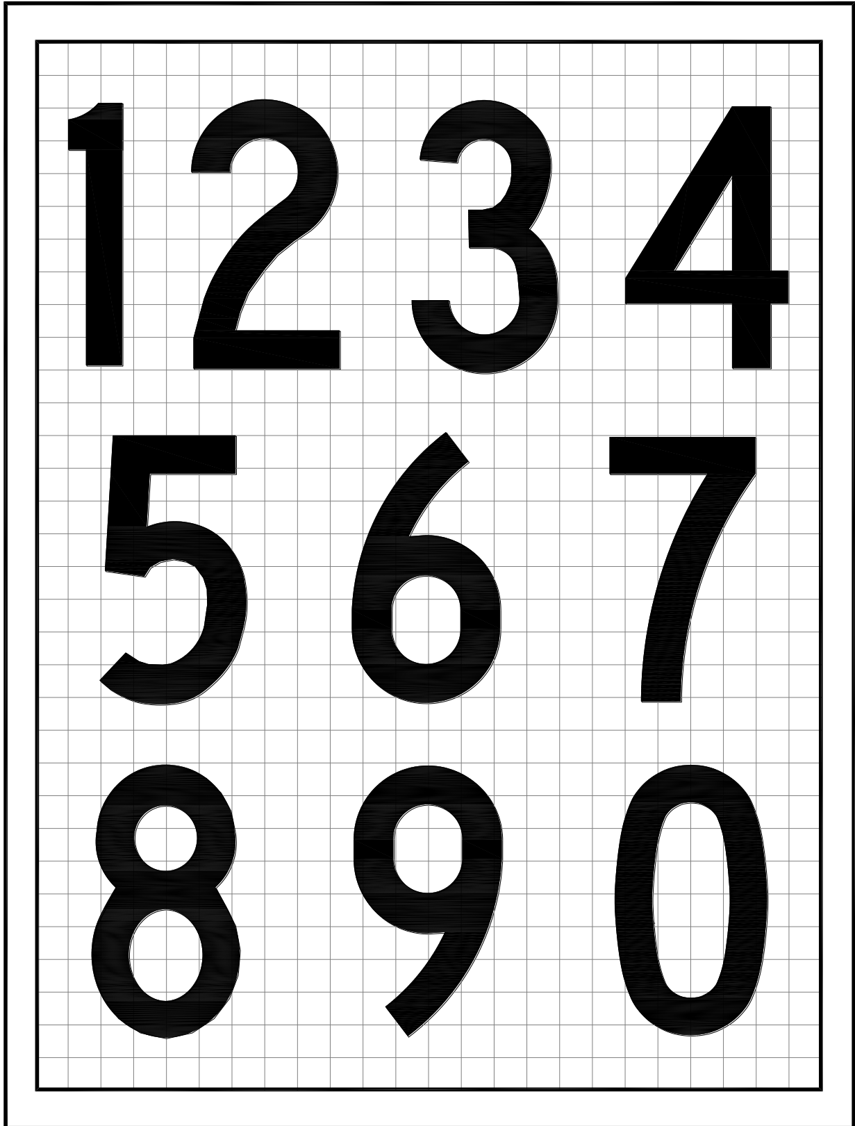
Figure 6. Numerals for Size 4 and 5 Signs (Types L-858B and L-858Ba)
