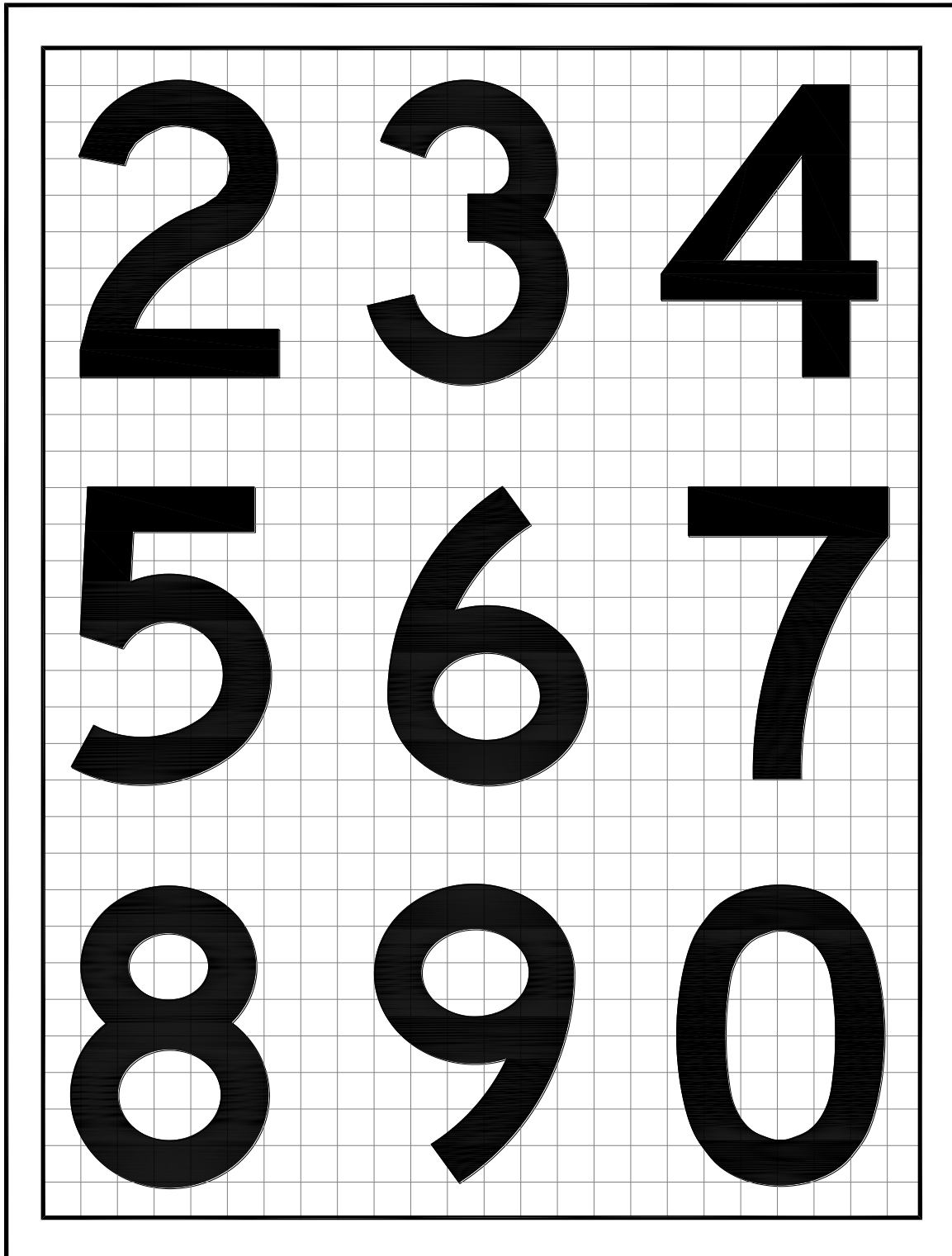
Figure 4. Numerals for Size 1, 2, and 3 Signs Types L-858Y, L-858R and L-858
