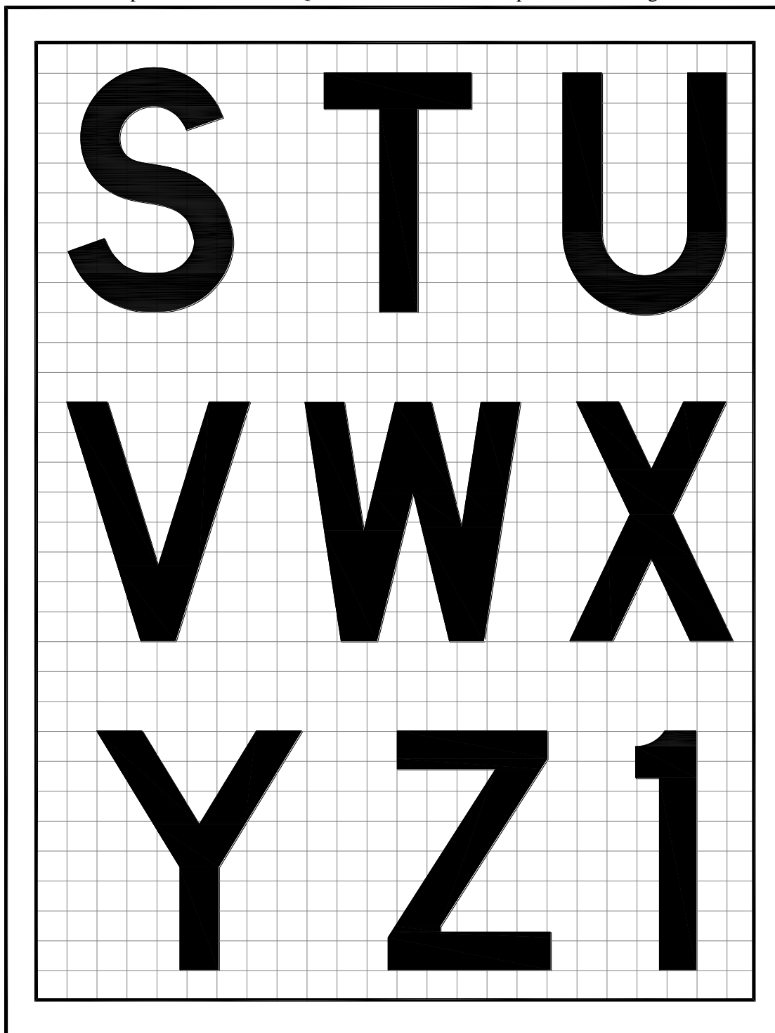
Figure 3. Sign Legend Characters and Numeral 1 for Size 1, 2, and 3 Signs Types L-858Y, L-858R and L-858L
