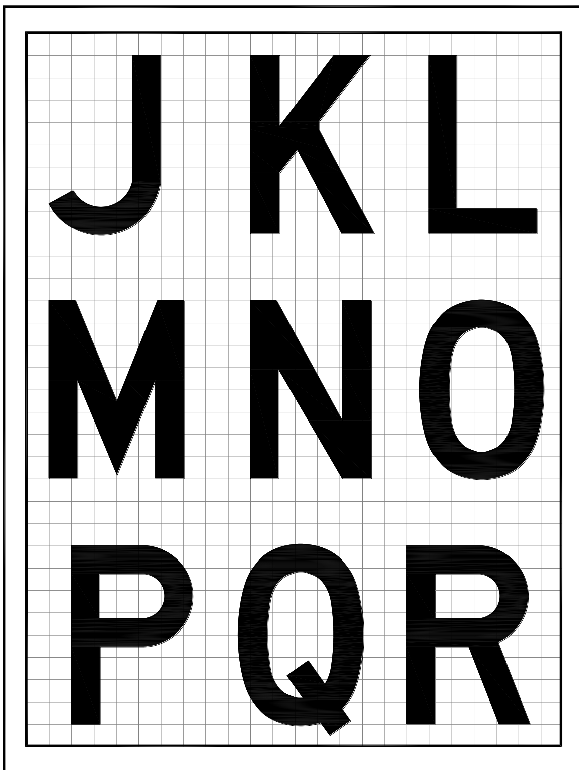
Figure 2. Sign Legend Characters for Size 1, 2, and 3 Signs Types L-858Y, L-858R and L-858L
