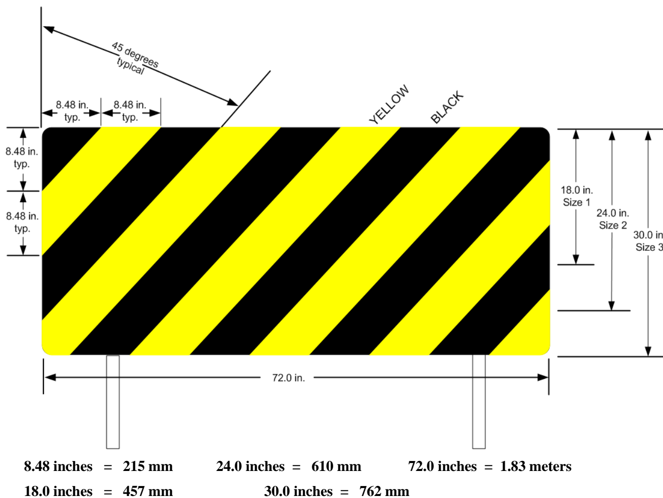
Figure 15. Type L-858C, 72.0 Inch Taxiway Ending Marker Signs
