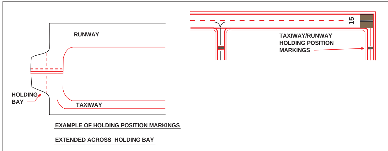
FIG 2-3-13 Runway Holding Position Markings on Taxiway
