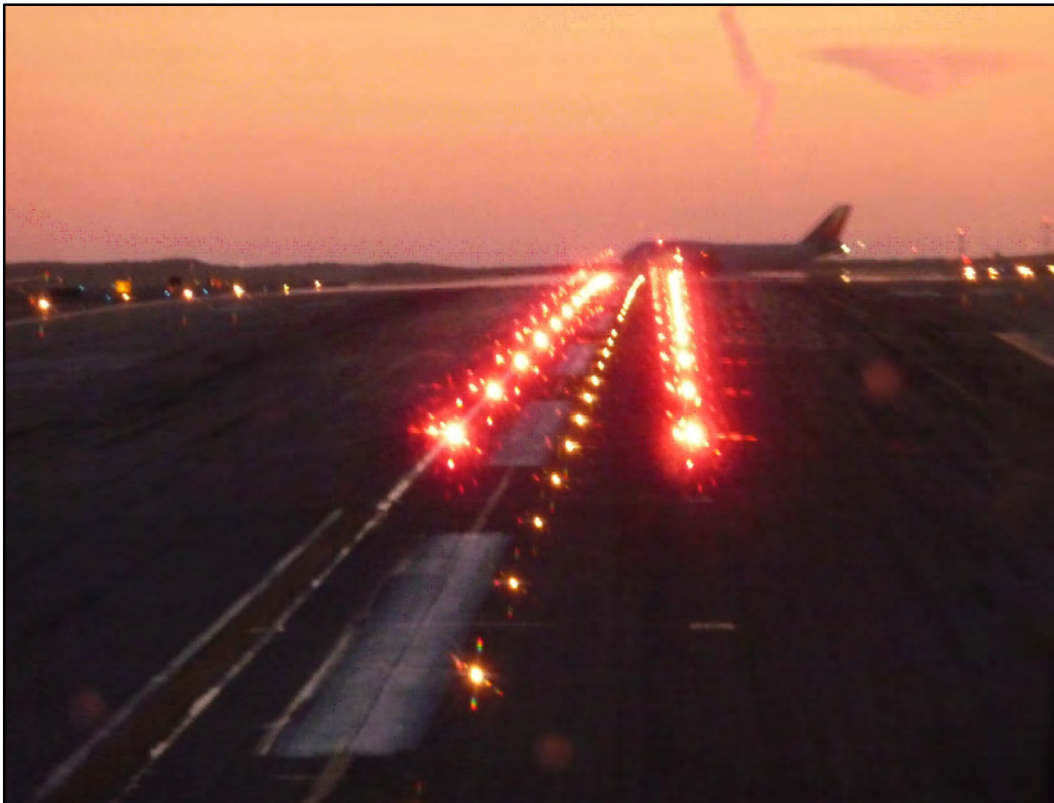
FIG 2-1-11 Takeoff Hold Lights
