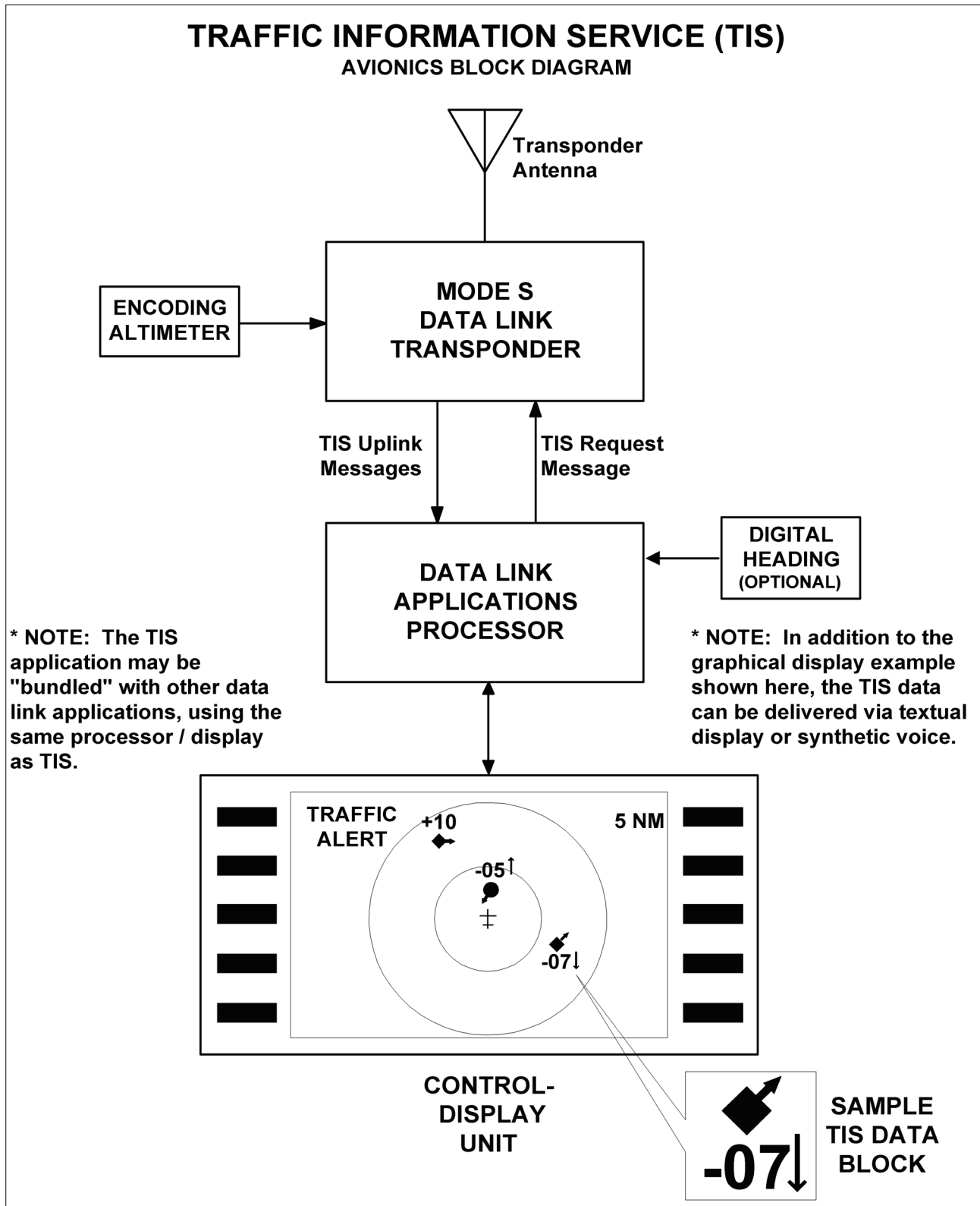
FIG 4-5-5 Traffic Information Service (TIS) Avionics Block Diagram
