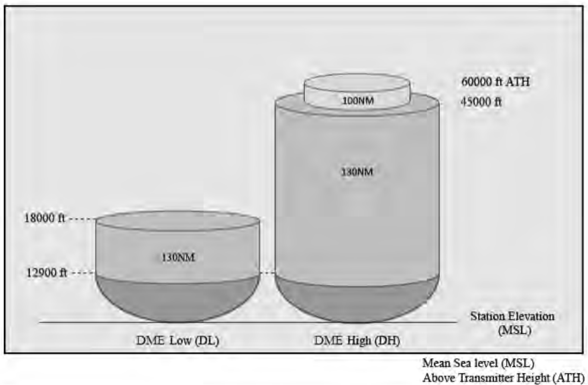
FIG 1-1-5 New DME Service Volumes
