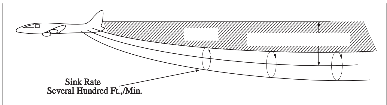
FIG GEN 3.5-20 Vortex Flow Field
