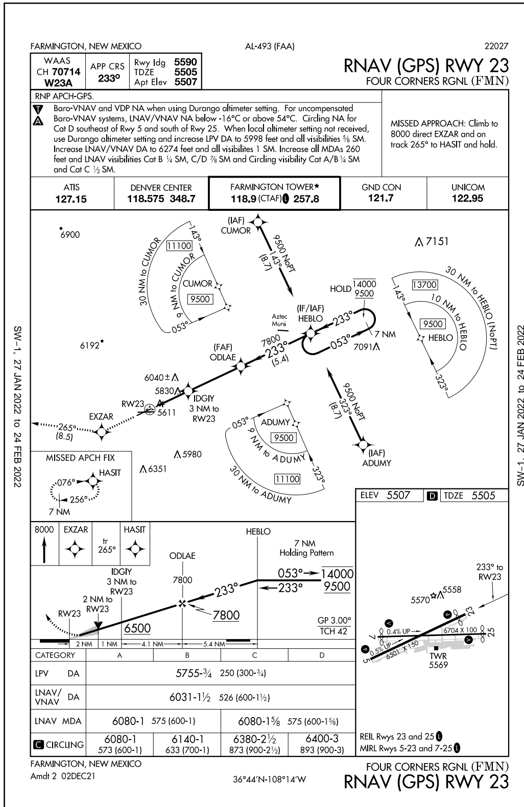
FIG ENR 1.5-22 RNAV (GPS) Approach Chart
