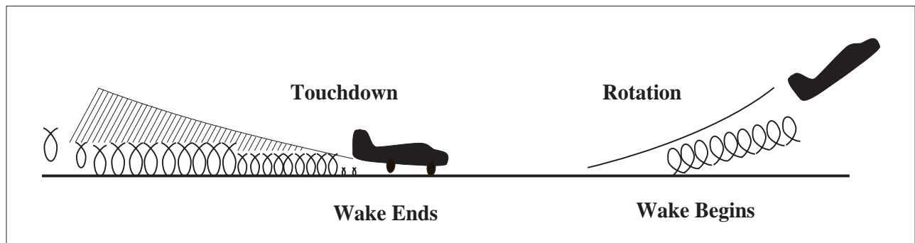
FIG GEN 3.5-19 Wake Ends/Wake Begins
