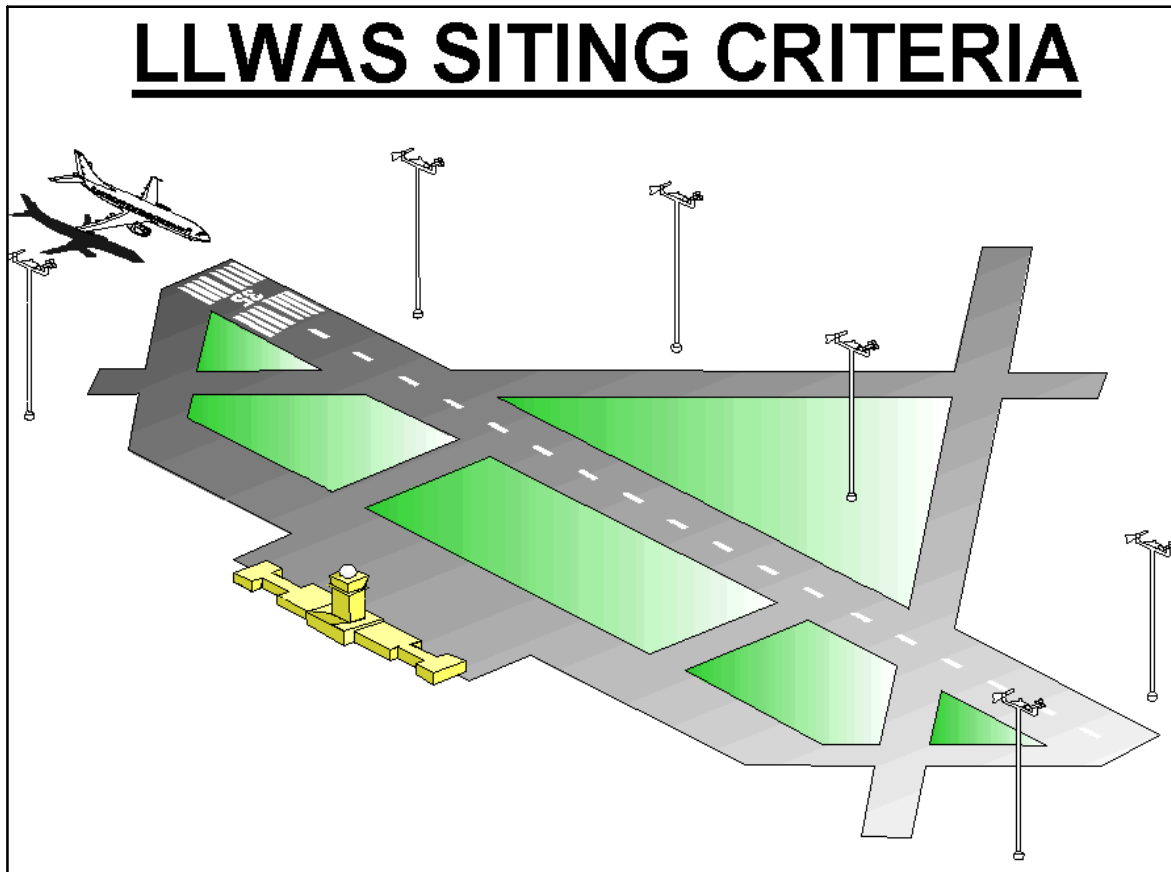
FIG GEN 3.5–II LLWAS Siting Criteria
