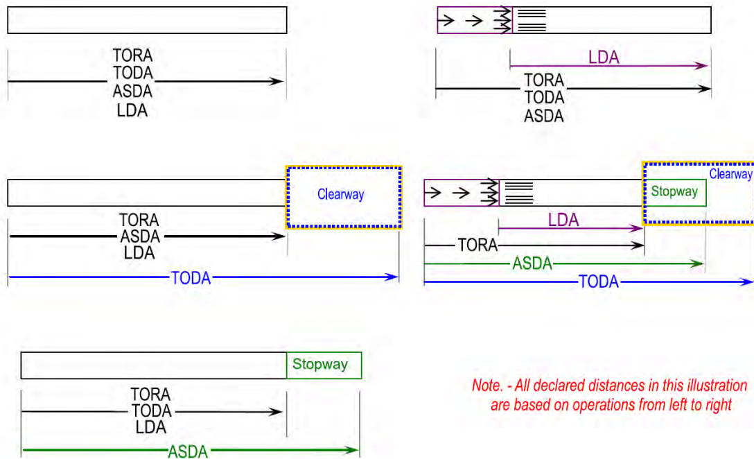
FIG ENR 1.1-5 Declared Distances with Full-Standard Runway Safety Areas, Runway Object Free Areas, and Runway Protection Zones
