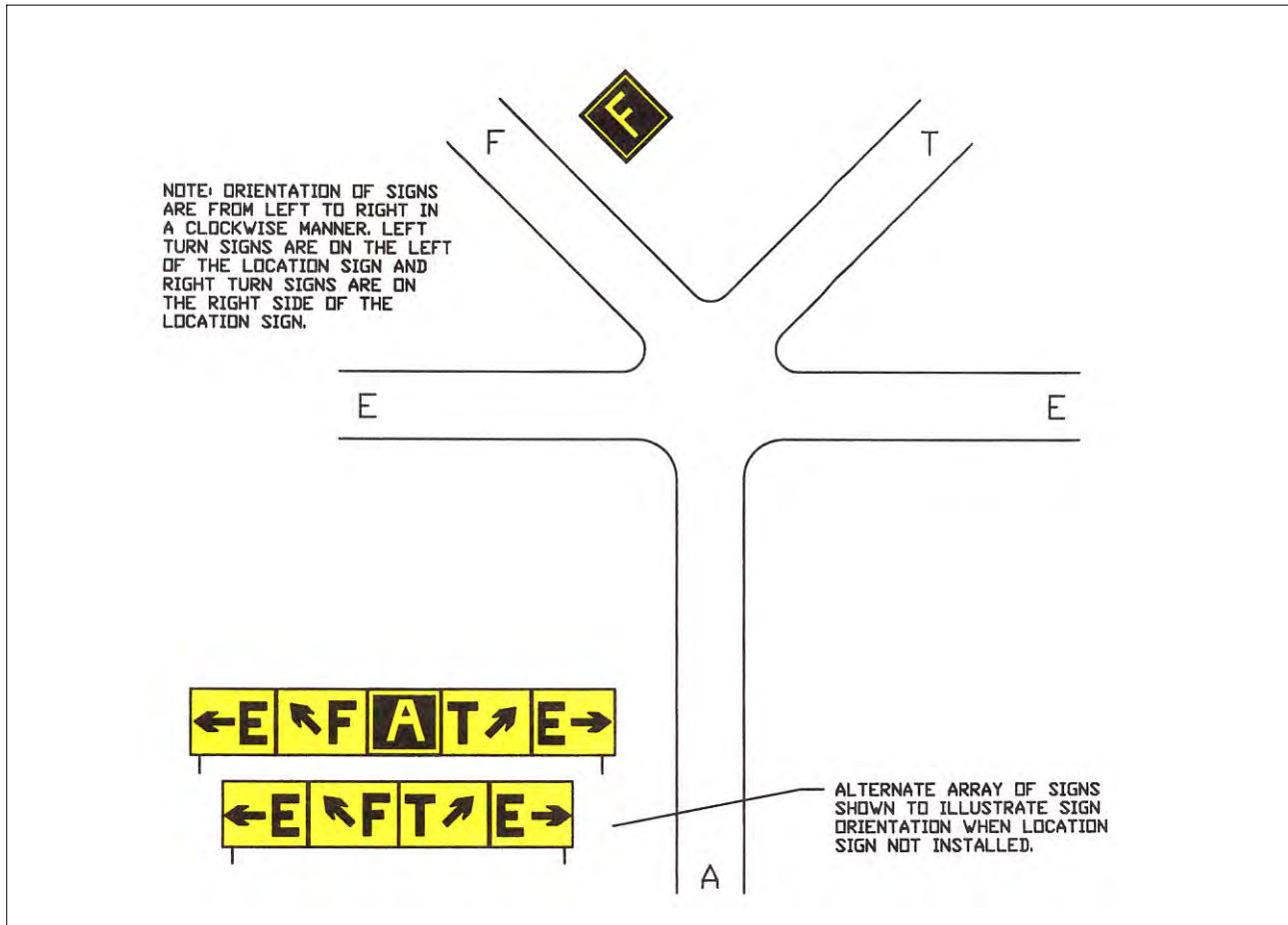
FIG AD 1.1-47 Direction Sign Array with Location Sign on Far Side of Intersection
