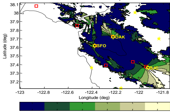
Figure 9. RNP coverage at 500 ft AGL with Pseudolite using DME & GBT sites, assumed range accuracy is 108.6 m
