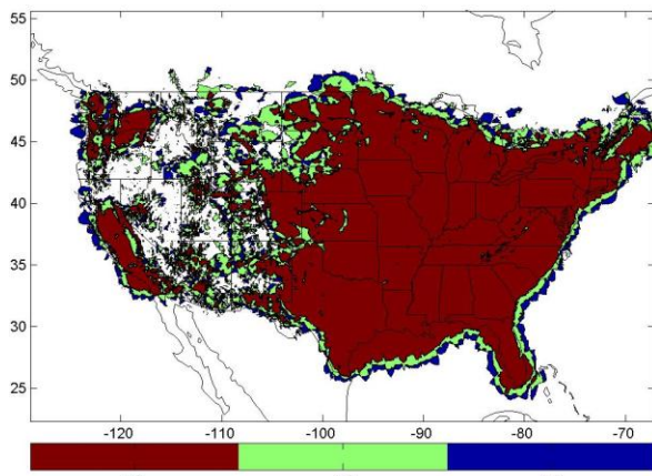
Figure 7. CONUS DOPs for Passive Range at 5000 ft AGL with DME & GBT [9]
