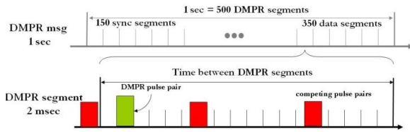
Figure 4. DMPR message & transmission structure
