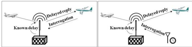
Figure 5. Comparison of nominal DME & DME passive ranging operations
