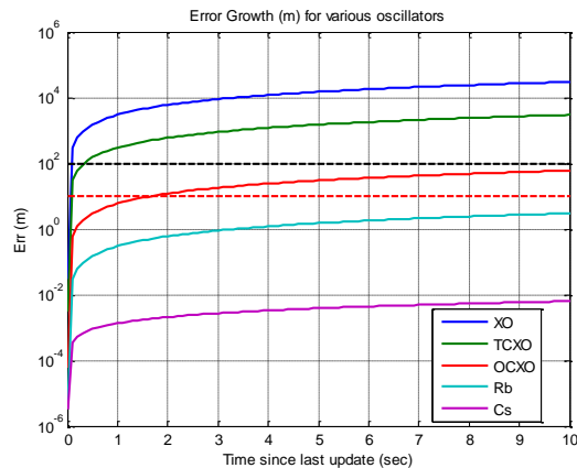
Figure 10. Clock Error Growth over time (various clocks) compared to approximate acceptable levels for surveillance (red dash) and RNP 0.3 (black dash)
