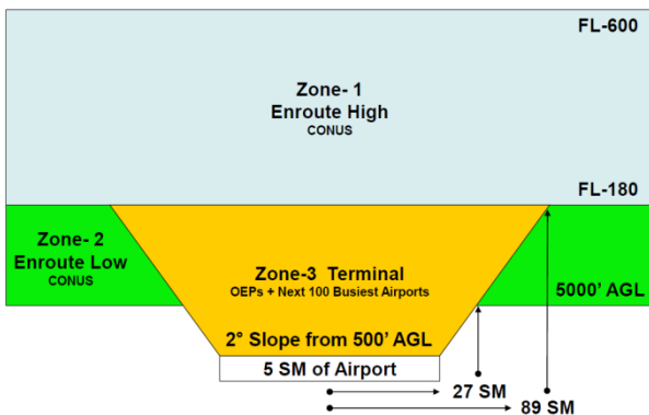
Figure 1. APNT Service Volume defined into 3 Zones. SM = statute mile. Operational Evolution Partnership (OEP) airports = top 35 busiest airports.
