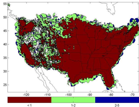
Figure 8. CONUS DOPs for True Range at 5000 ft AGL with DME & GBT [9]
