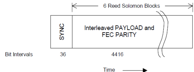
Figure 3. UAT Ground Segment Message (with Forward Error Correction (FEC)) [2]
