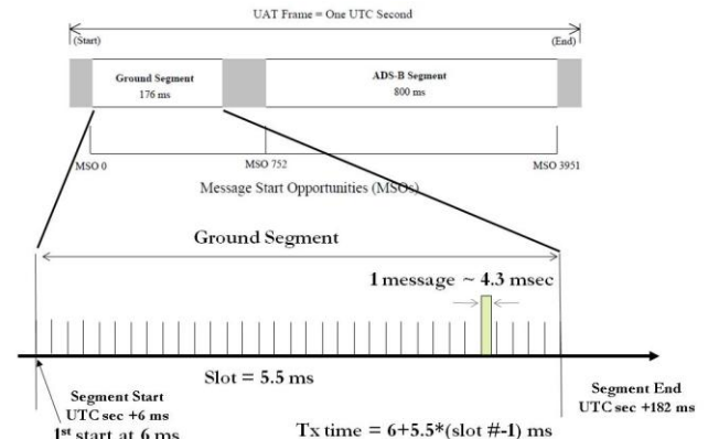
Figure 2. UAT Frame (grey areas = guard band) with expanded view of Ground Segment [2]
