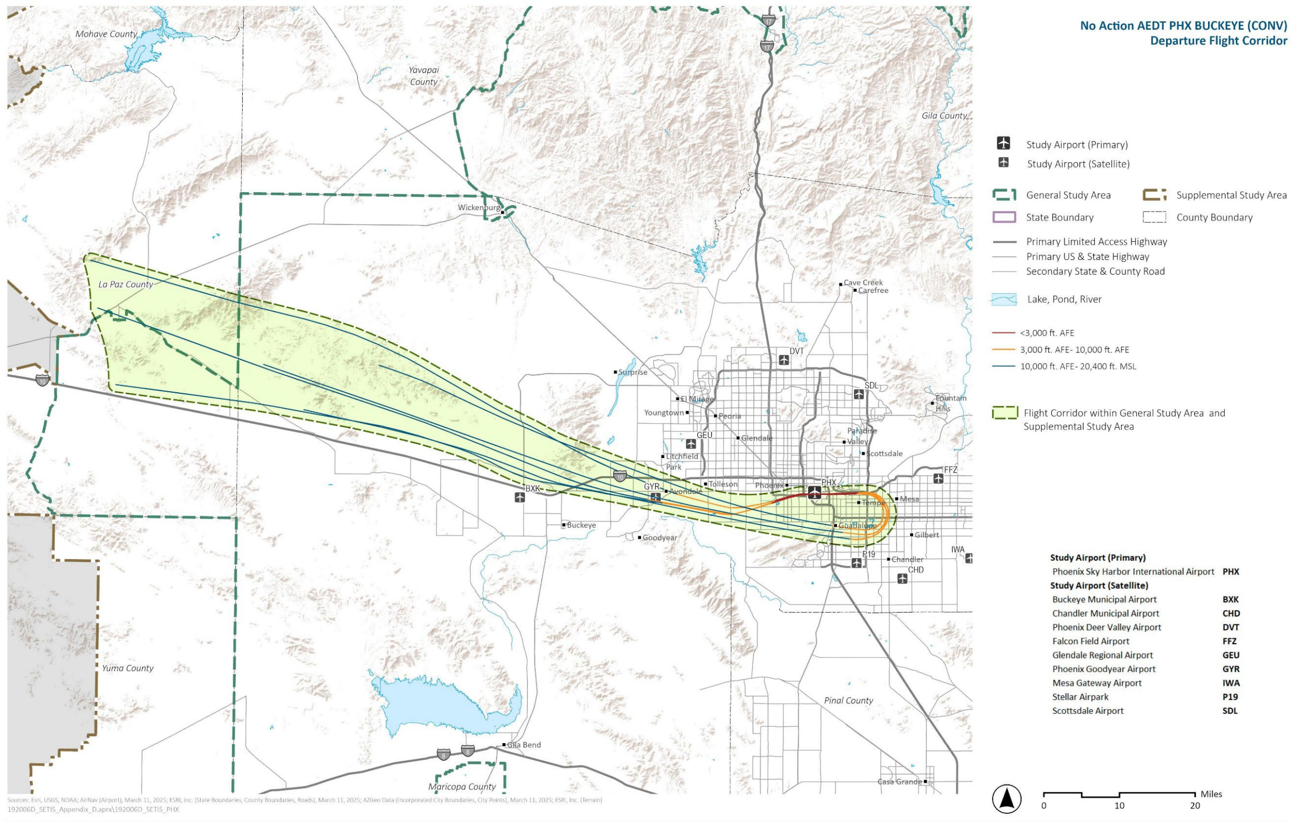
Exhibit H.1-14. No Action AEDT PHX BUCKEYE (CONV) Departure Flight Corridor
