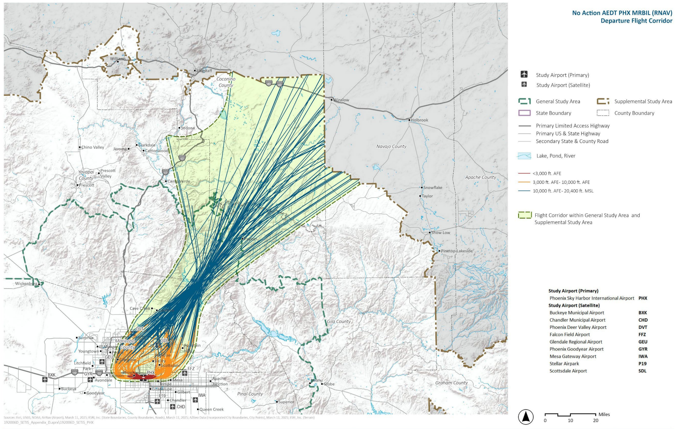
Exhibit H.1-20. No Action AEDT PHX MRBIL (RNAV) Departure Flight Corridor
