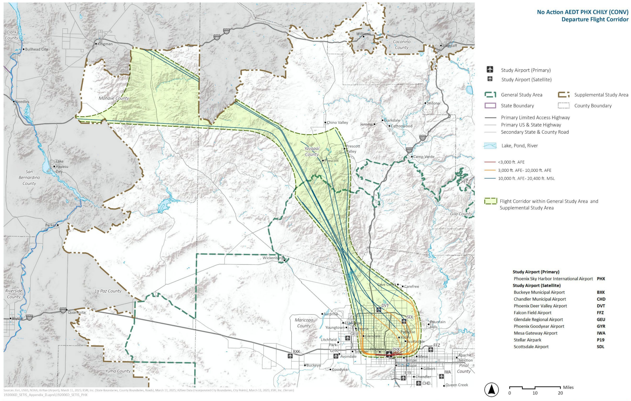
Exhibit H.1-15. No Action AEDT PHX CHILY (CONV) Departure Flight Corridor
