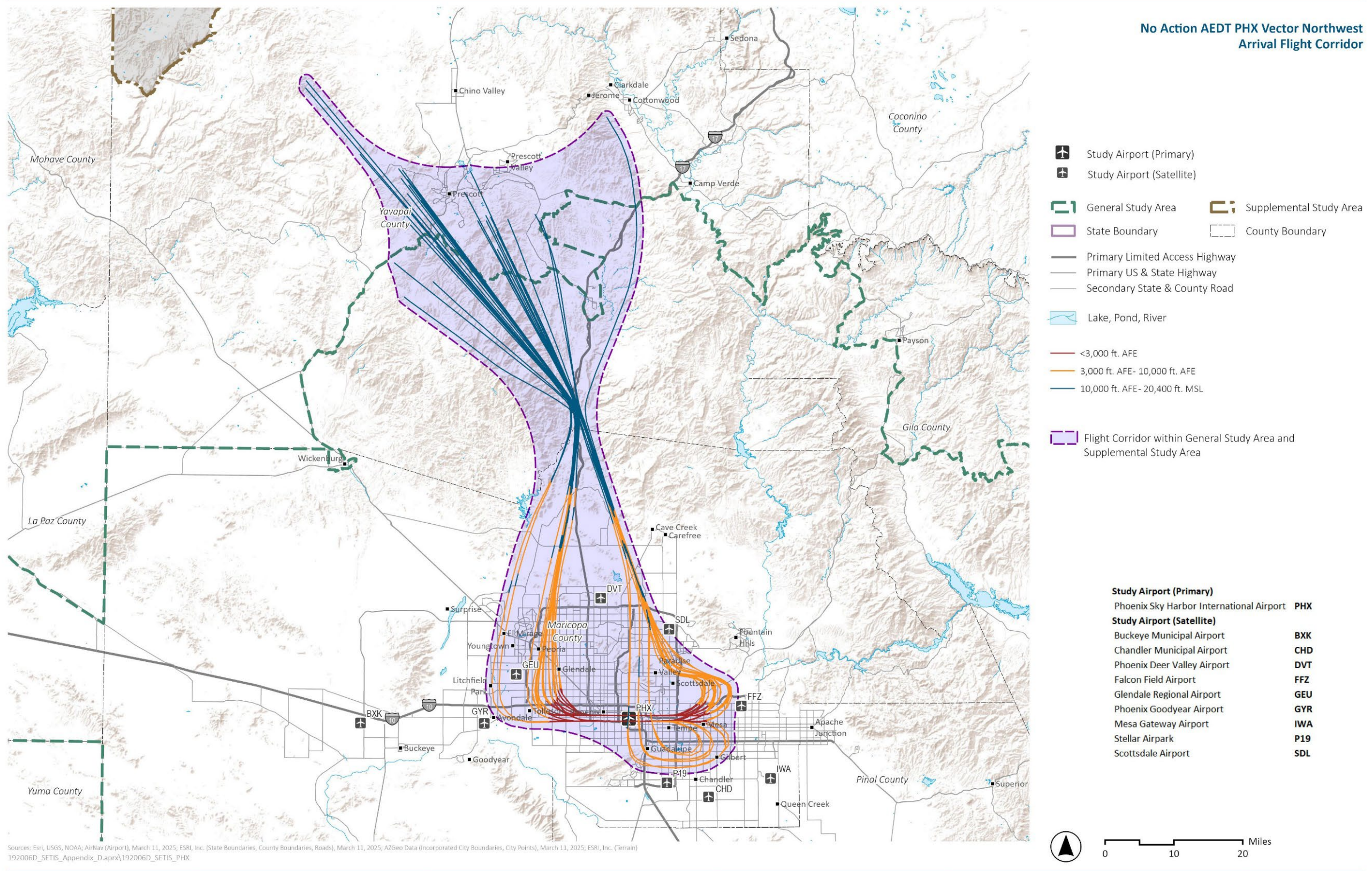
Exhibit H.1-11. No Action AEDT PHX Vector Northwest Arrival Flight Corridor
