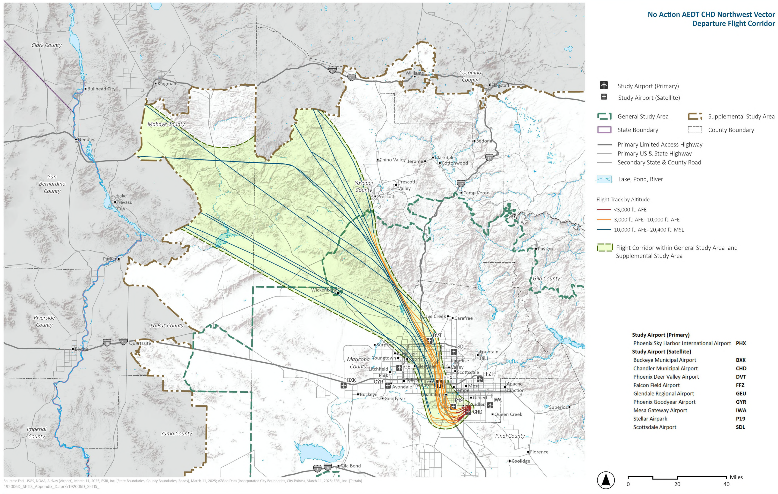
Exhibit H.3-20. No Action AEDT CHD Northwest Vector Departure Flight Corridor
