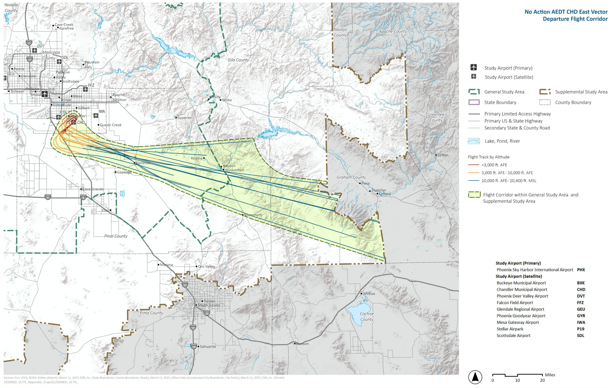
Exhibit H.3-17. No Action AEDT CHD East Vector Departure Flight Corridor
