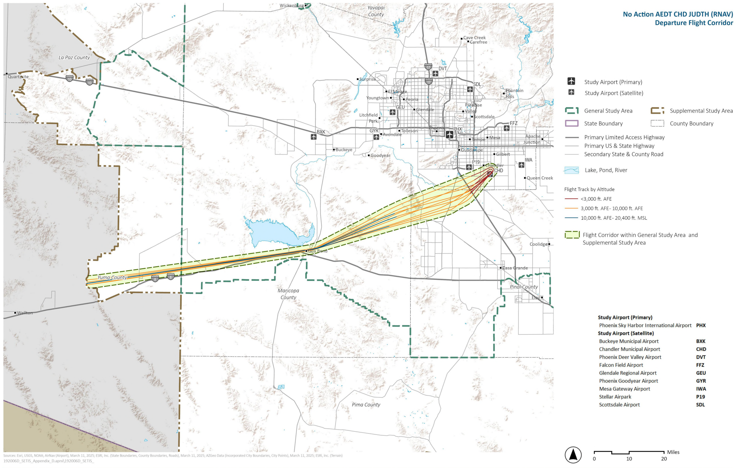
Exhibit H.3-13. No Action AEDT CHD JUDTH (RNAV) Departure Flight Corridor
