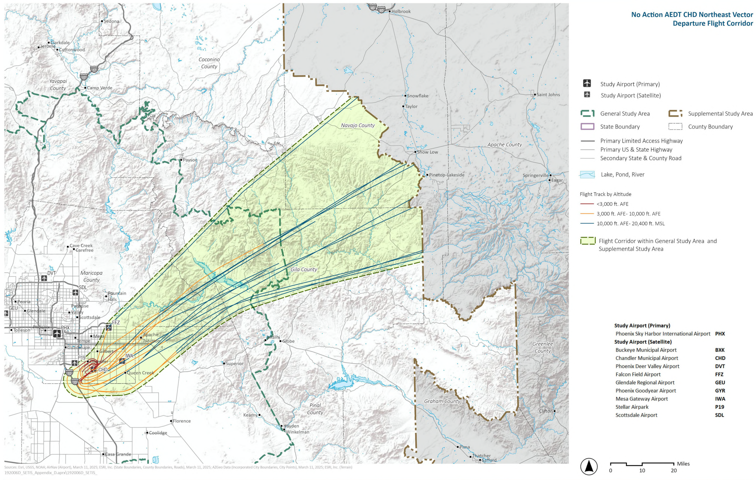
Exhibit H.3-19. No Action AEDT CHD Northeast Vector Departure Flight Corridor
