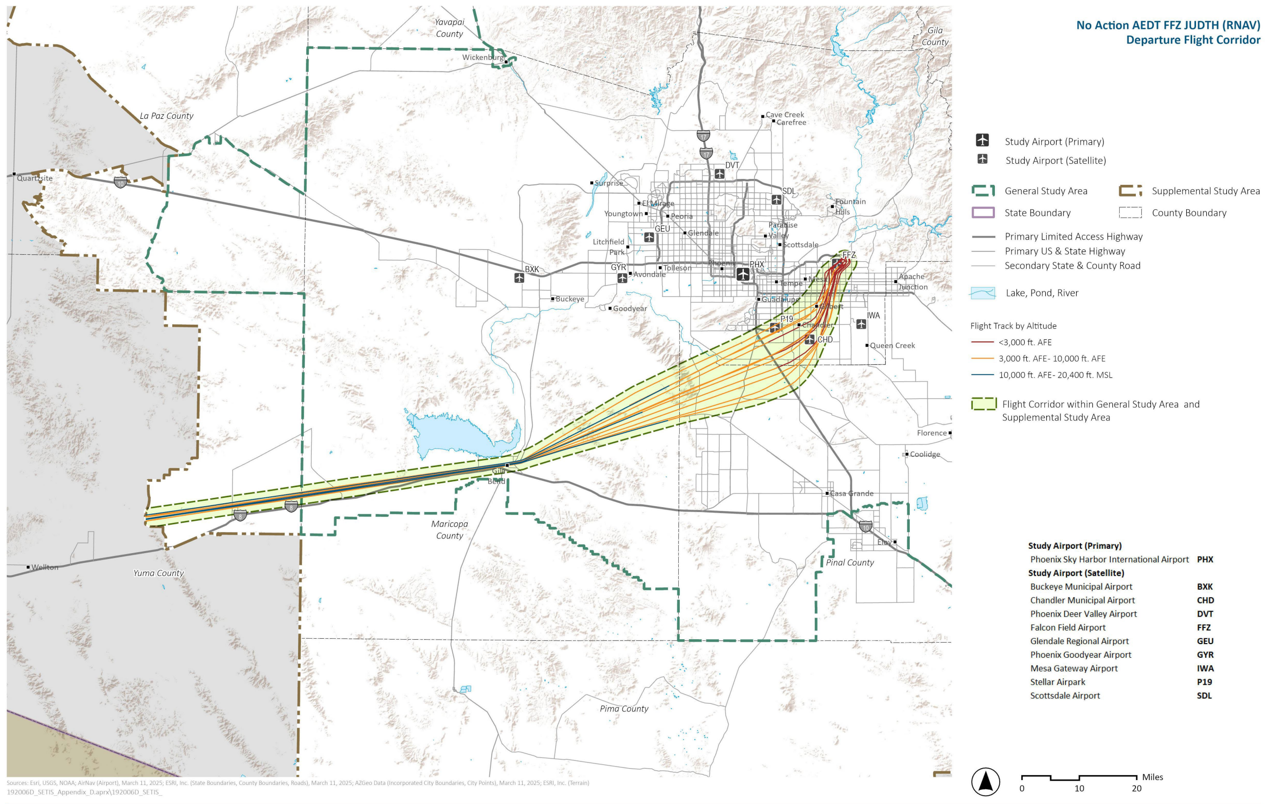
Exhibit H.5-15. No Action AEDT FFZ JUDTH (RNAV) Departure Flight Corridor
