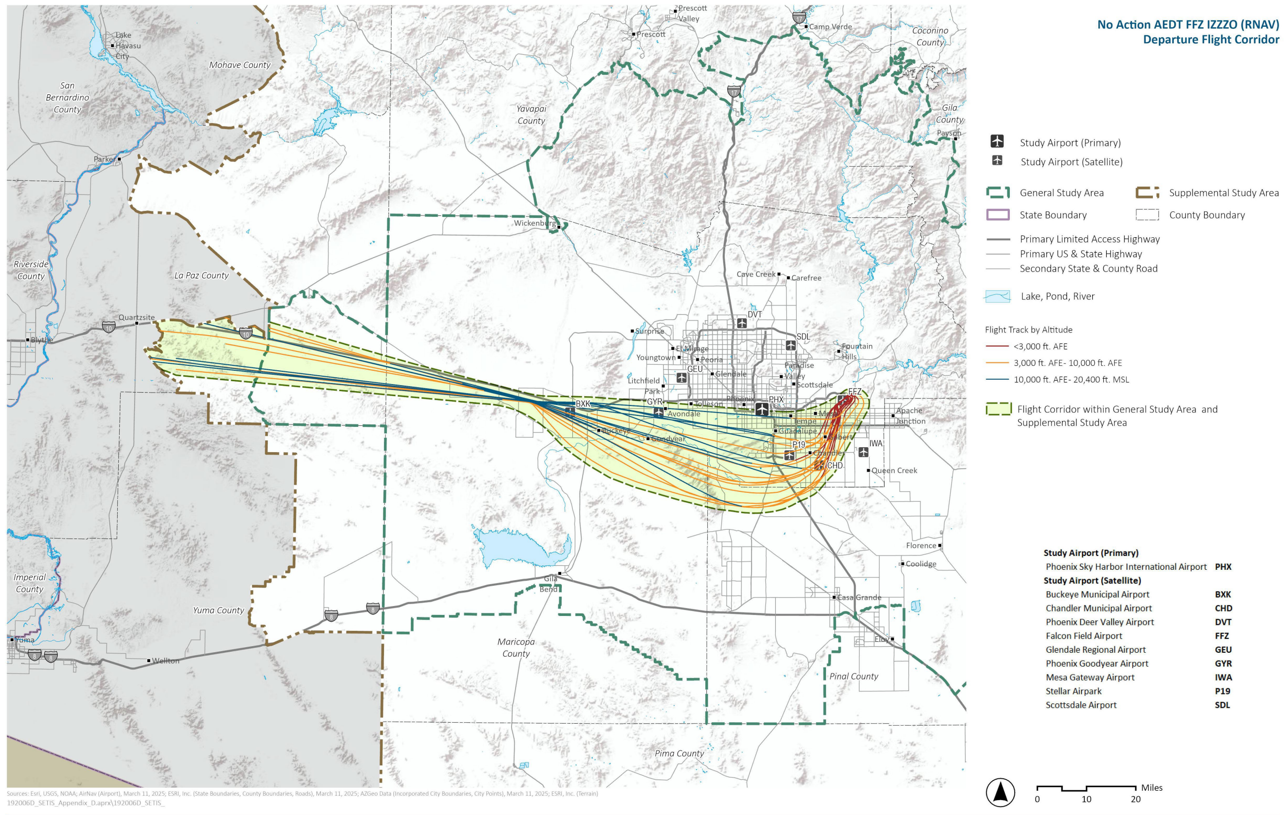
Exhibit H.5-13. No Action AEDT FFZ IZZO (RNAV) Departure Flight Corridor
