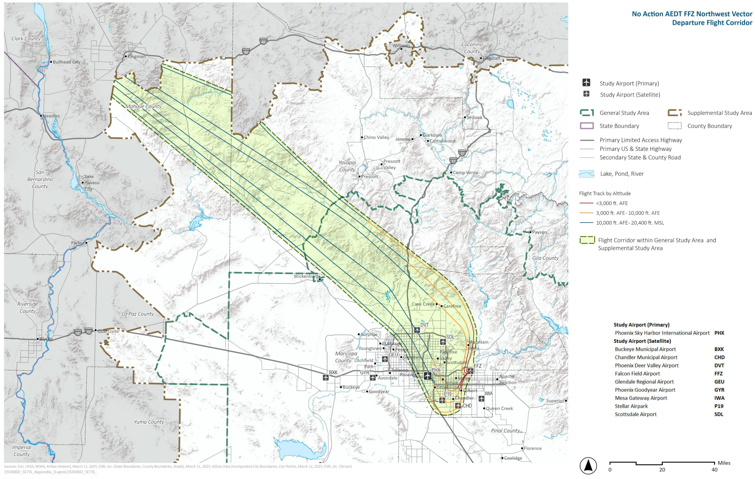
Exhibit H.5-23. No Action AEDT FFZ Northwest Vector Departure Flight Corridor
