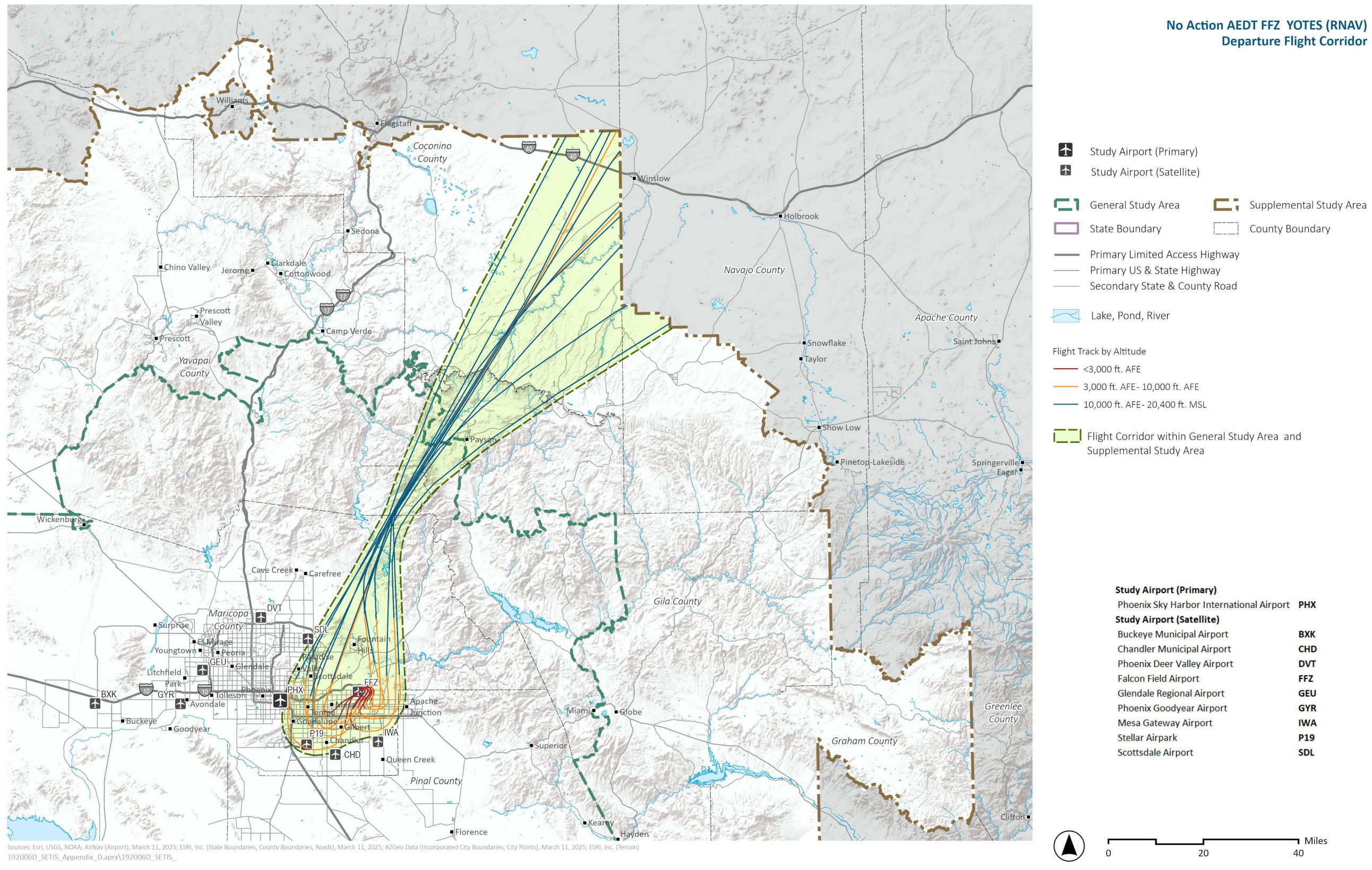
Exhibit H.5-25. No Action AEDT FFZ YOTES (RNAV) Departure Flight Corridor
