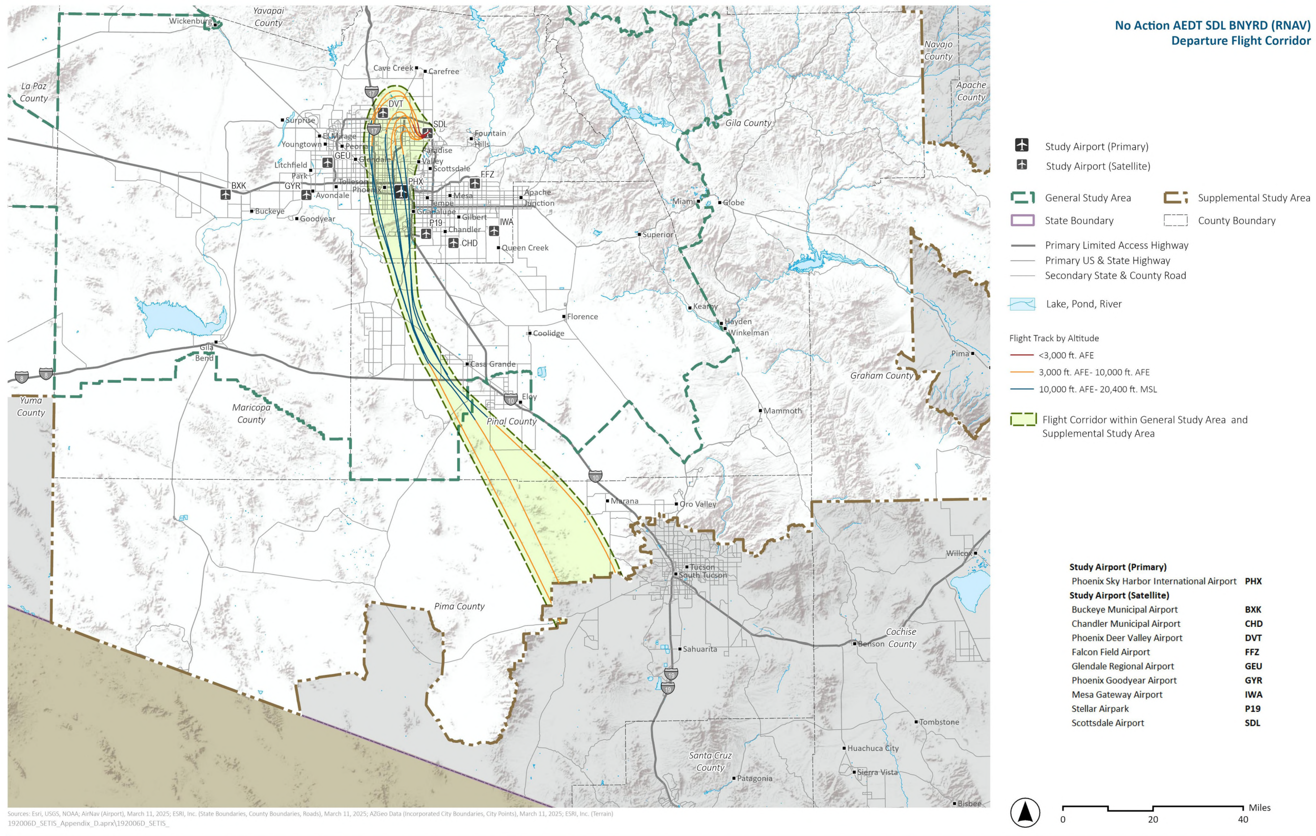
Exhibit H.10-8. No Action AEDT SDL BNYRD (RNAV) Departure Flight Corridor
