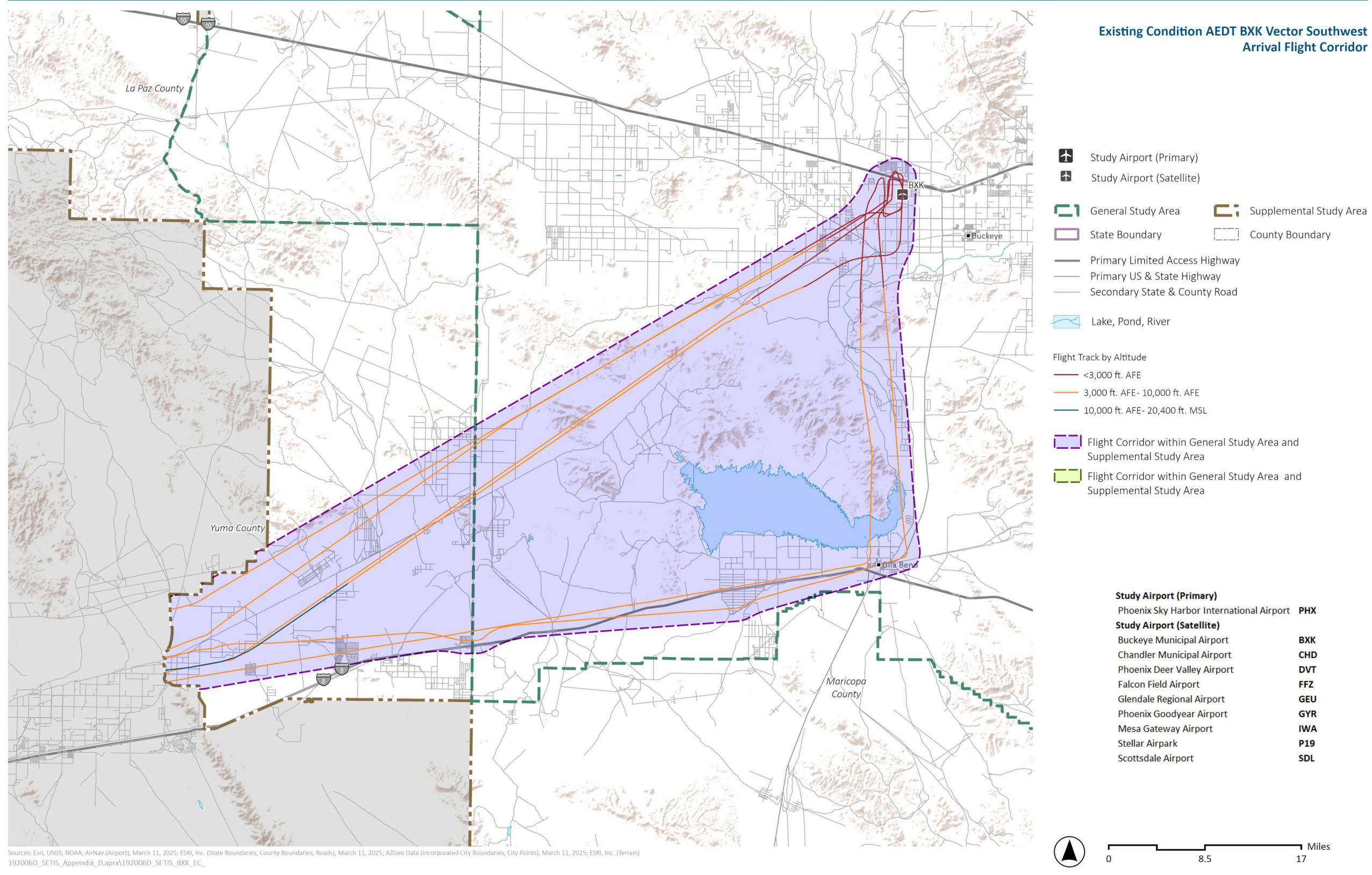
Exhibit H.11-5. Existing Condition AEDT BXK Vector Southwest Arrival Flight Corridor
