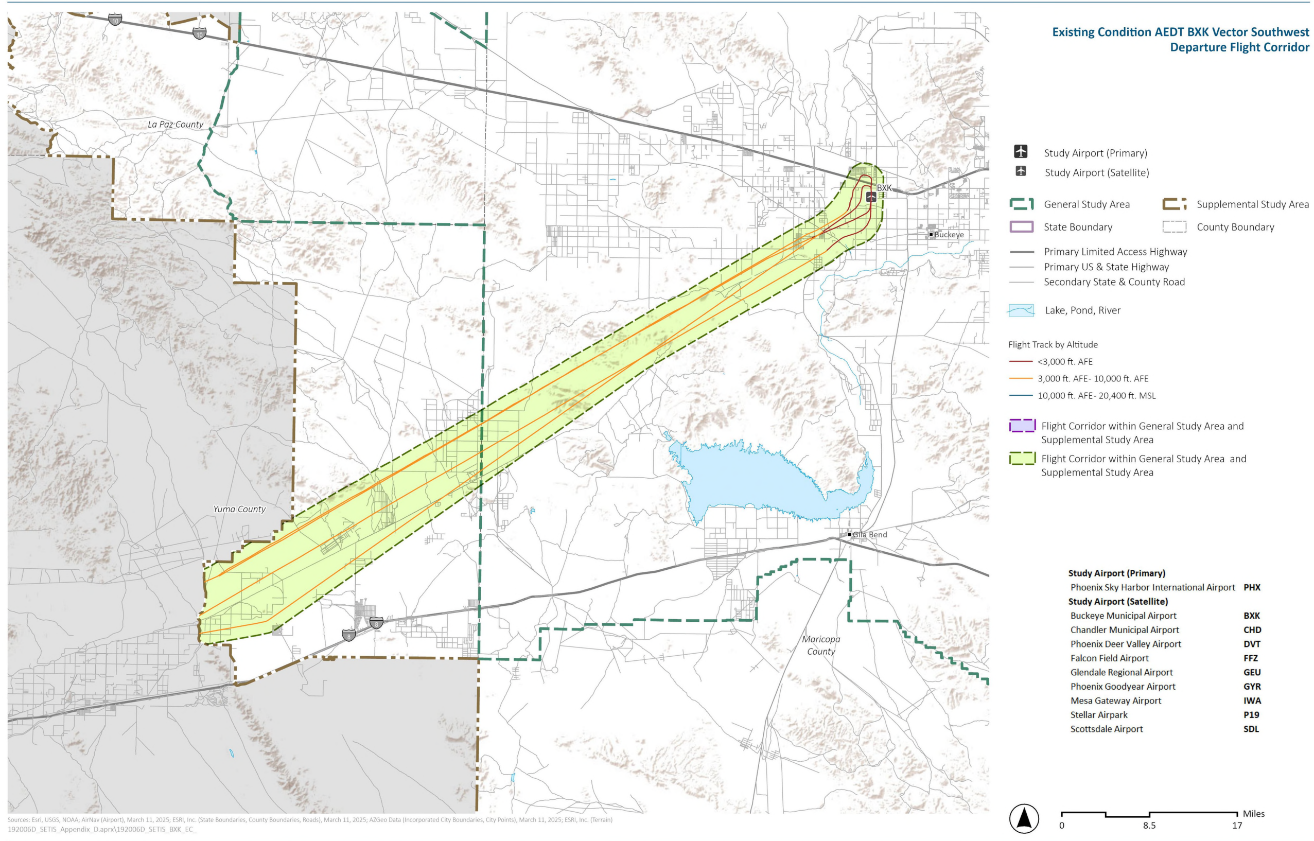
Exhibit H.11-11. Existing Condition AEDT BKK Vector Southwest Departure Flight Corridor
