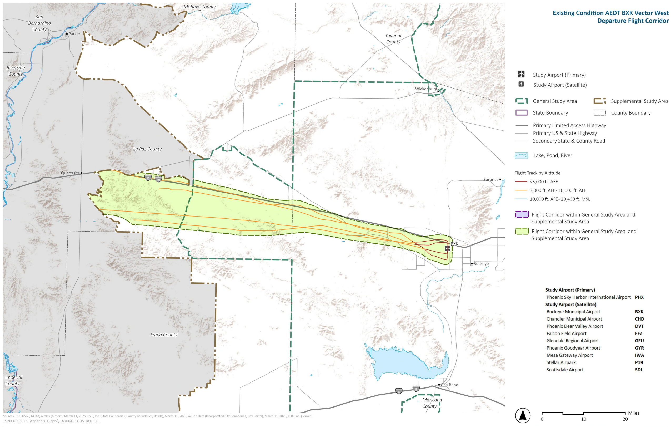
Exhibit H.11-12. Existing Condition AEDT BXK Vector West Departure Flight Corridor
