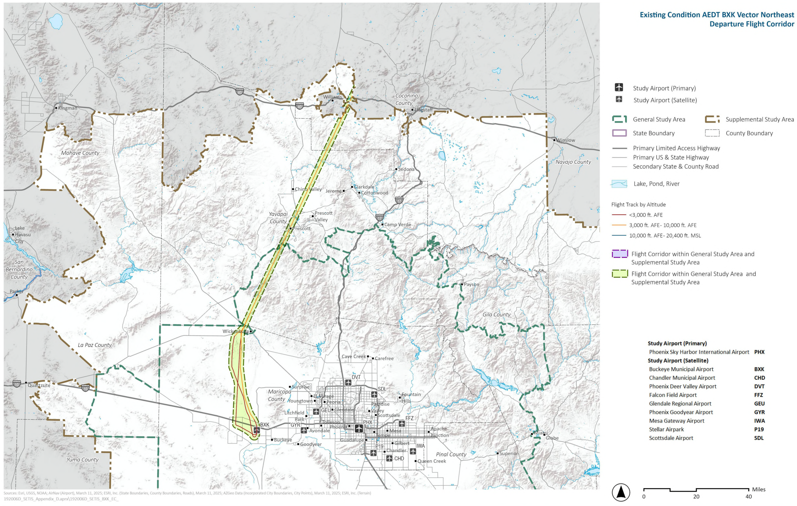
Exhibit H.11-8. Existing Condition AEDT BXK Vector Northeast Departure Flight Corridor
