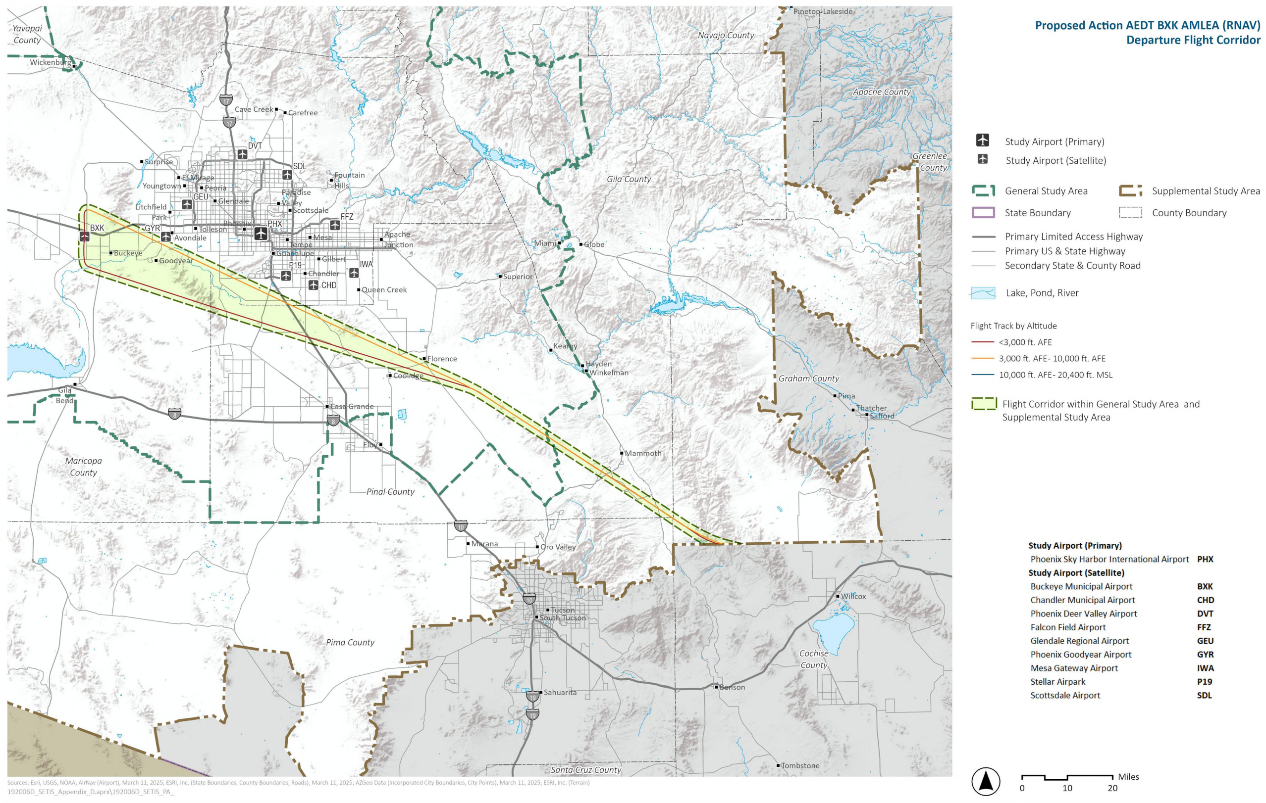
Exhibit I.2-8. Proposed Action AEDT BXK AMLEA (RNAV) Departure Flight Corridor
