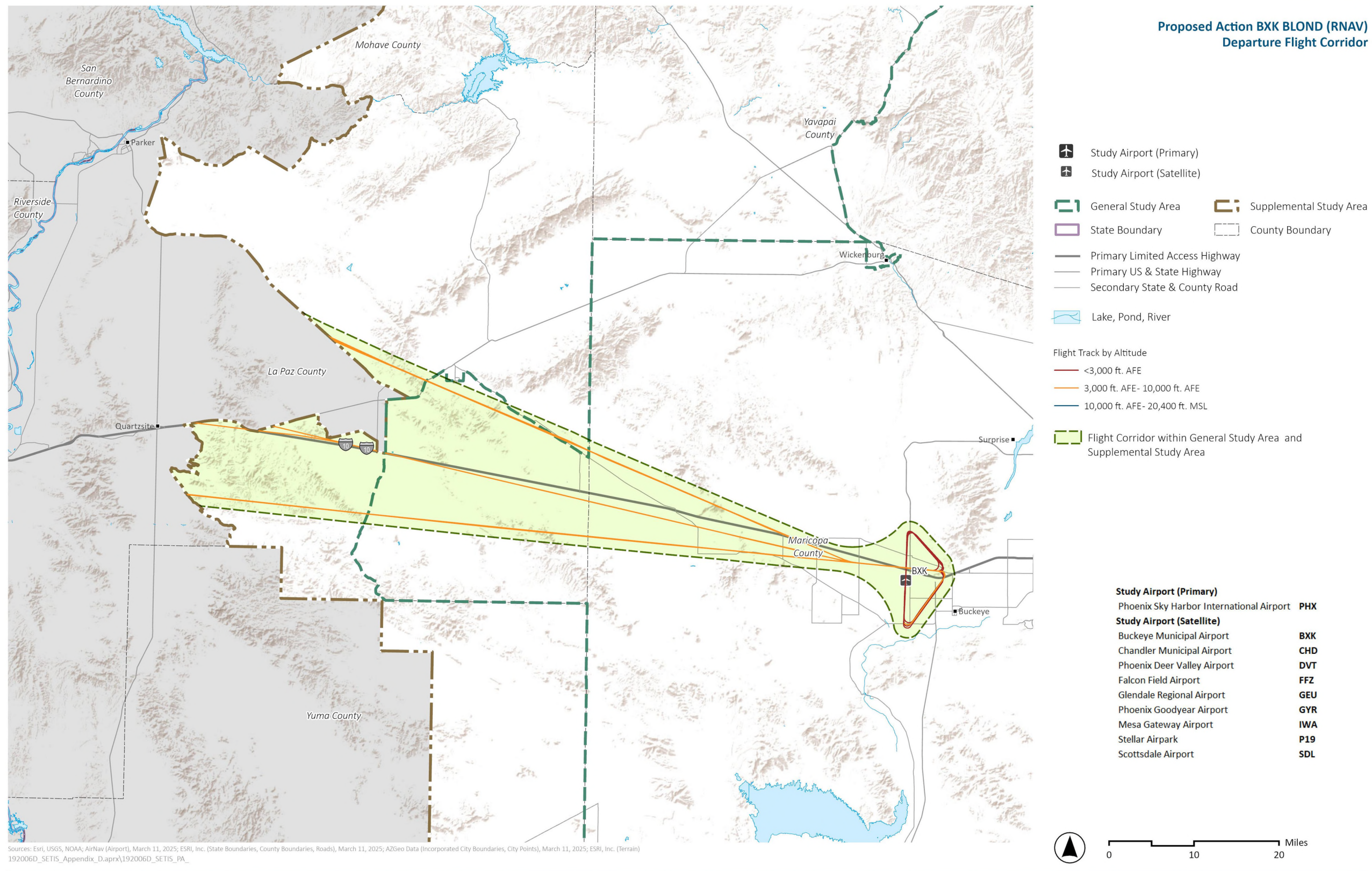
Exhibit I.2-9. Proposed Action AEDT BXK BLOND (RNAV) Departure Flight Corridor
