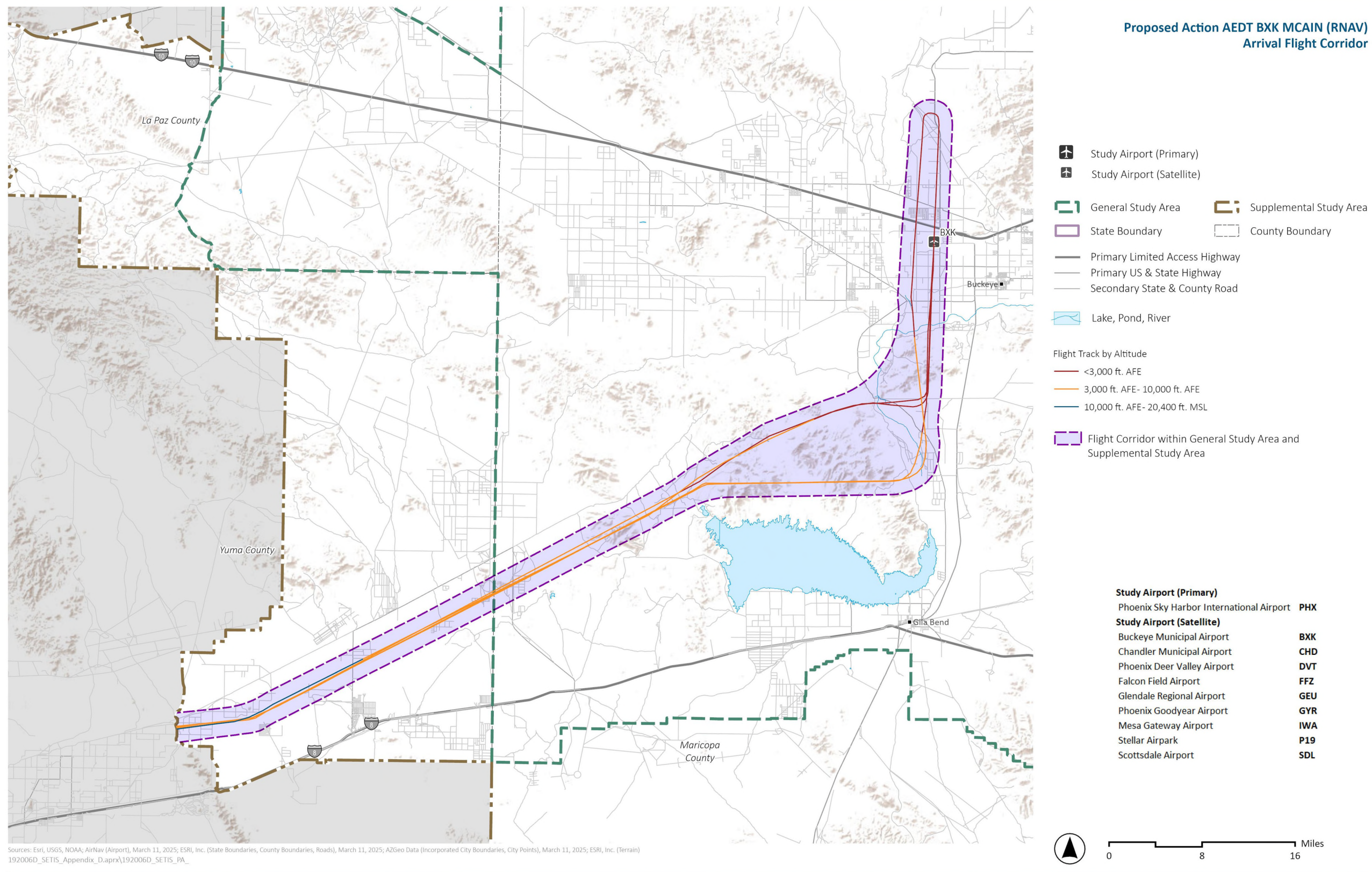
Exhibit I.2-3. Proposed Action AEDT BXK MCAIN (RNAV) Arrival Flight Corridor
