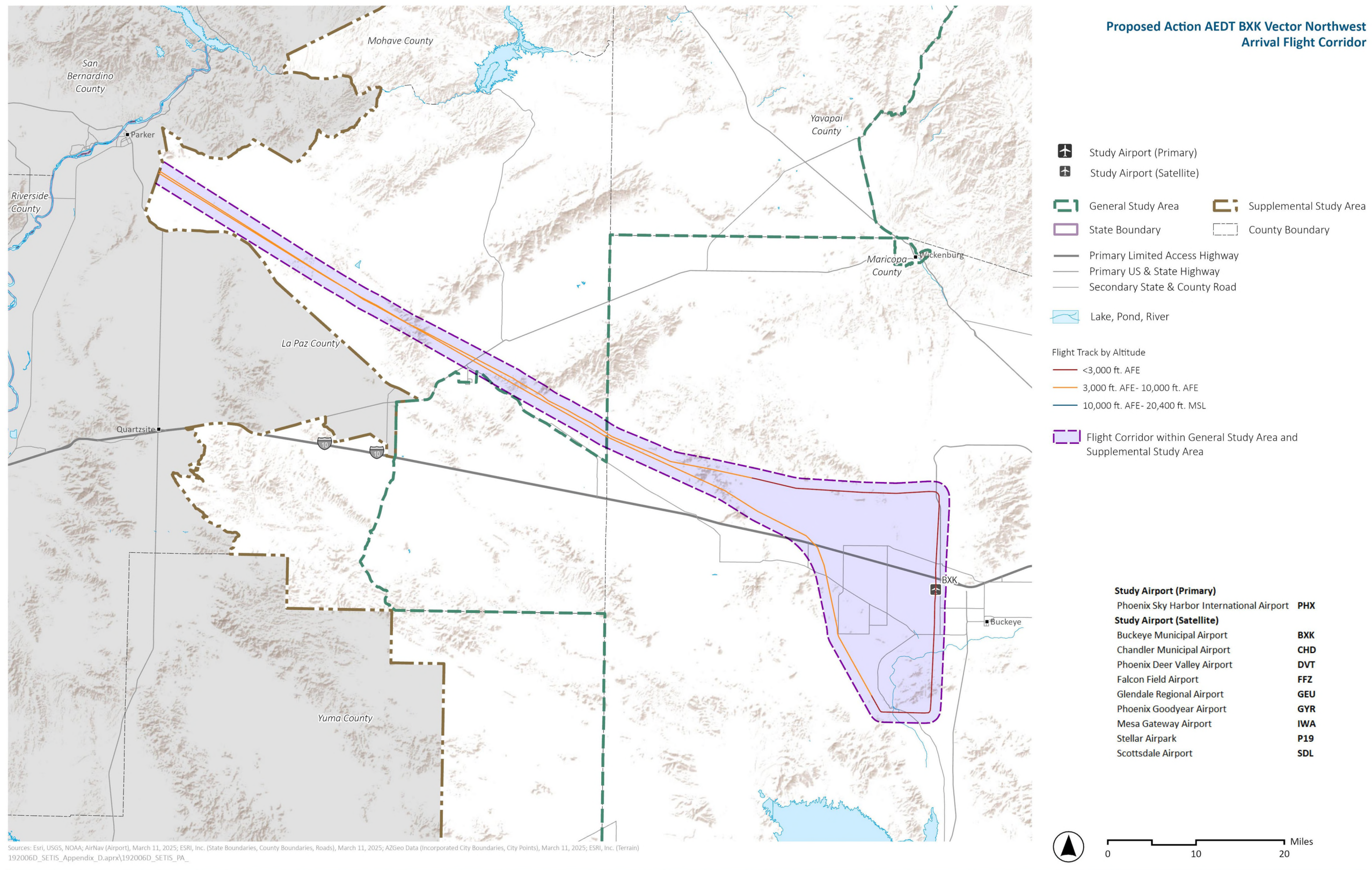
Exhibit I.2-6. Proposed Action AEDT BXK Vector Northwest Arrival Flight Corridor
