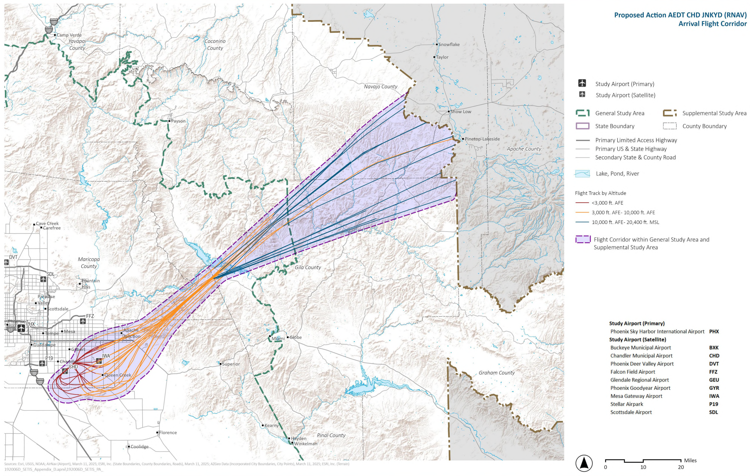
Exhibit I.3-2. Proposed Action AEDT CHD JNKYD (RNAV) Arrival Flight Corridor
