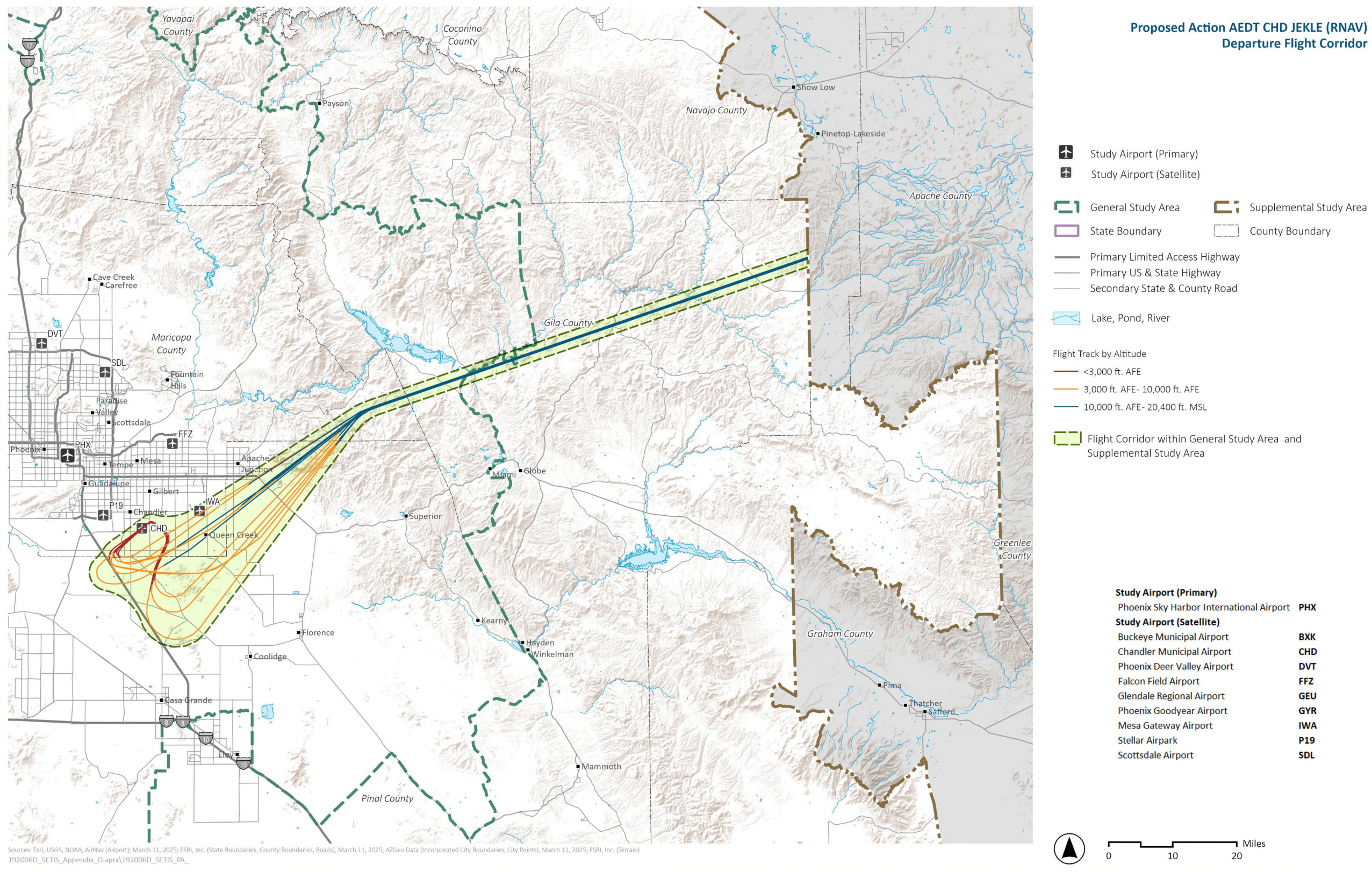
Exhibit I.3-10. Proposed Action AEDT CHD JEKLE (RNAV) Departure Flight Corridor
