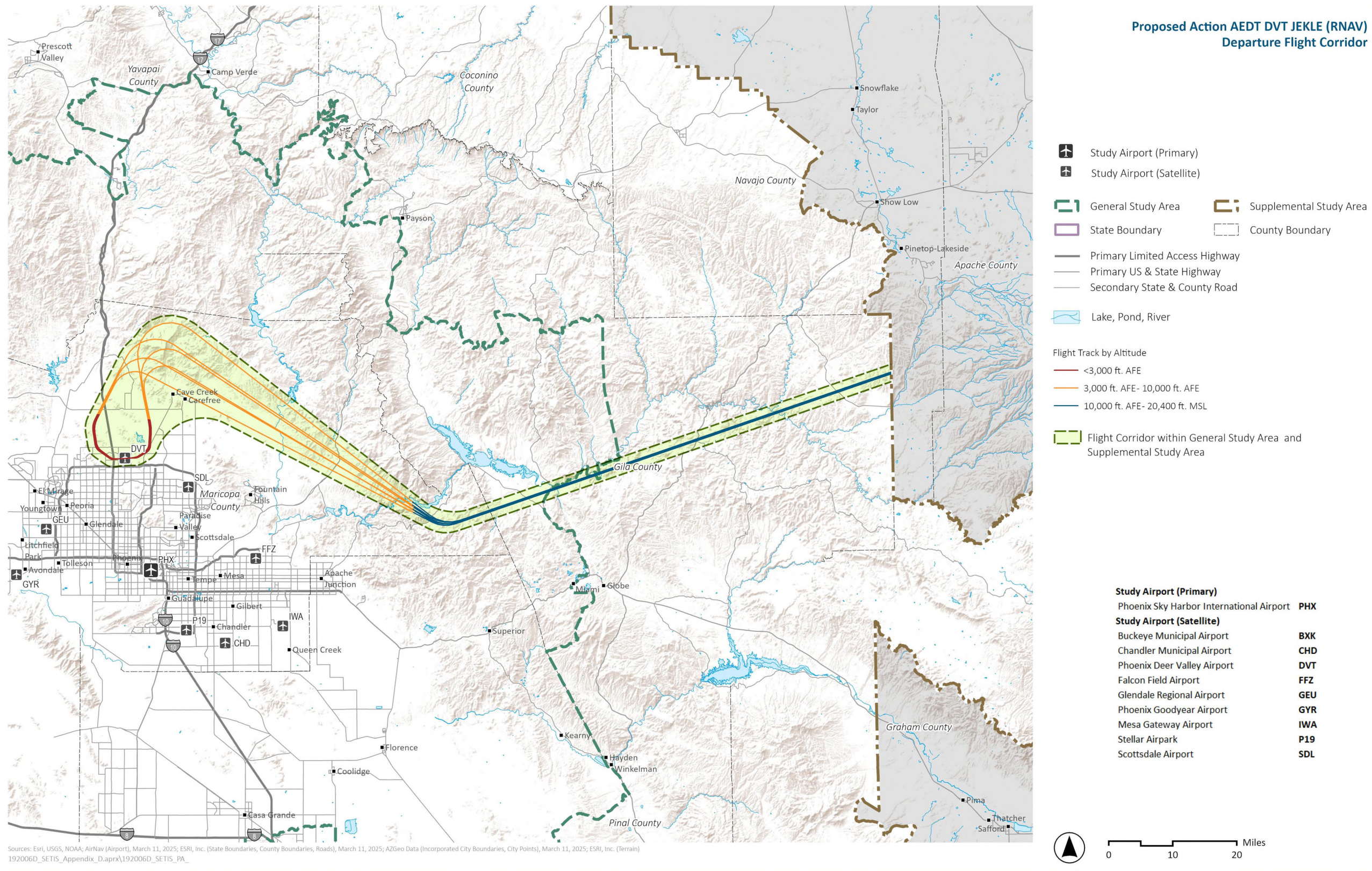
Exhibit I.4-11. Proposed Action AEDT DVT JEKLE (RNAV) Departure Flight Corridor
