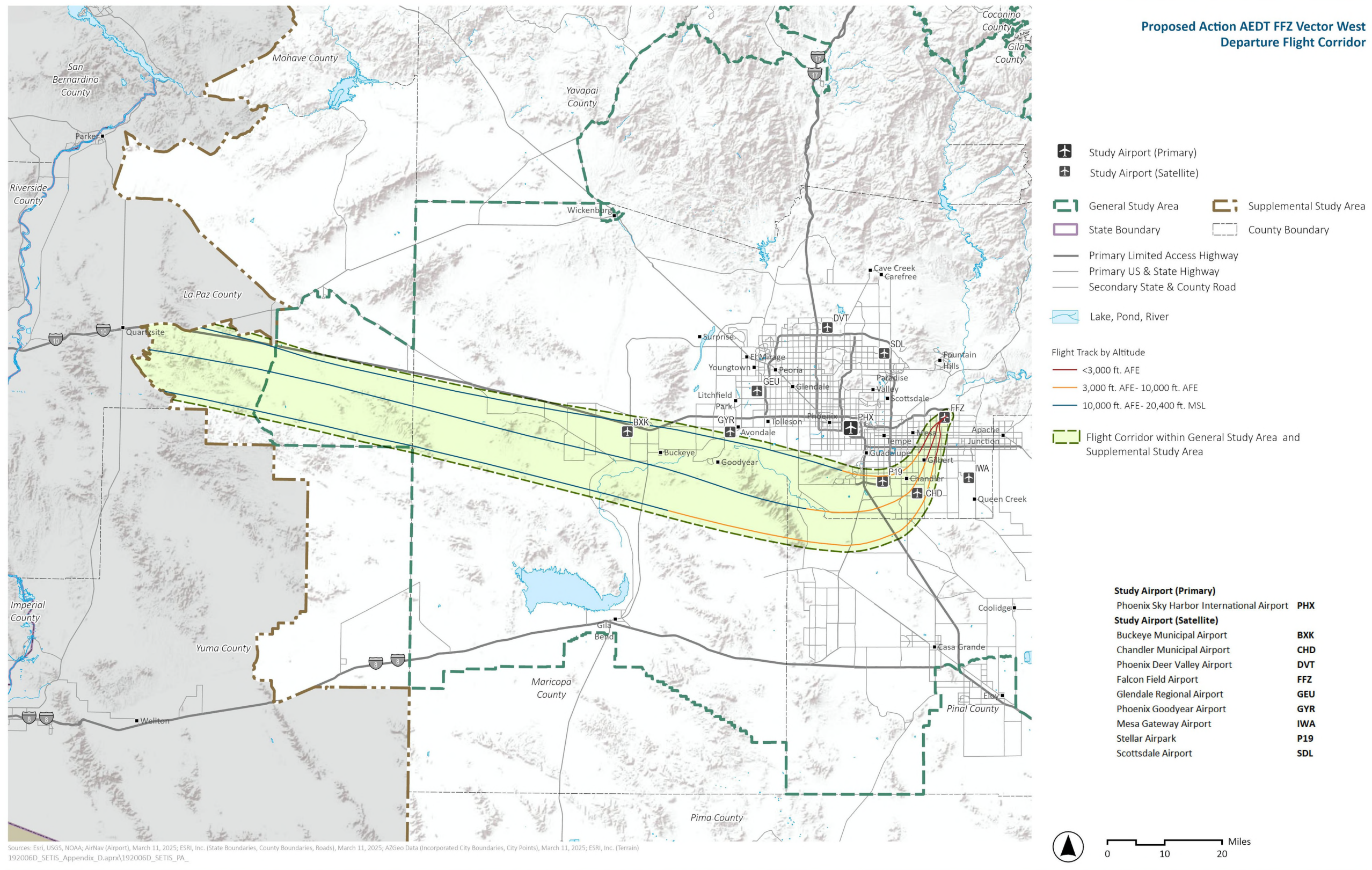
Exhibit I.5-16. Proposed Action AEDT FFZ Vector West Departure Flight Corridor
