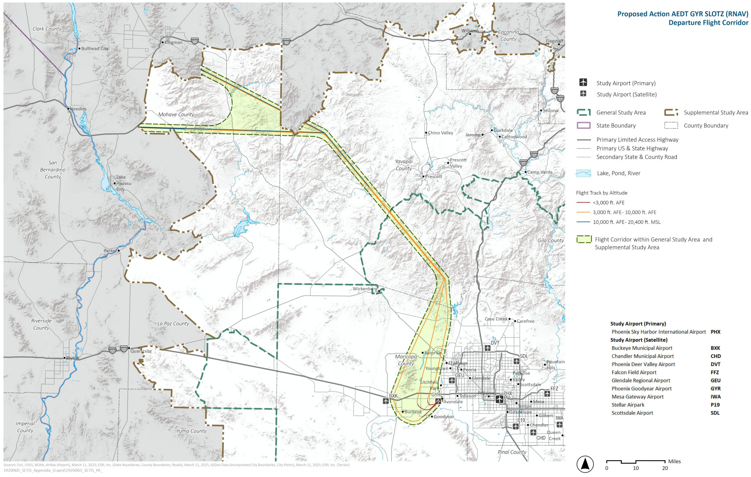
Exhibit I.7-8. Proposed Action AEDT GYR SLOTZ (RNAV) Departure Flight Corridor
