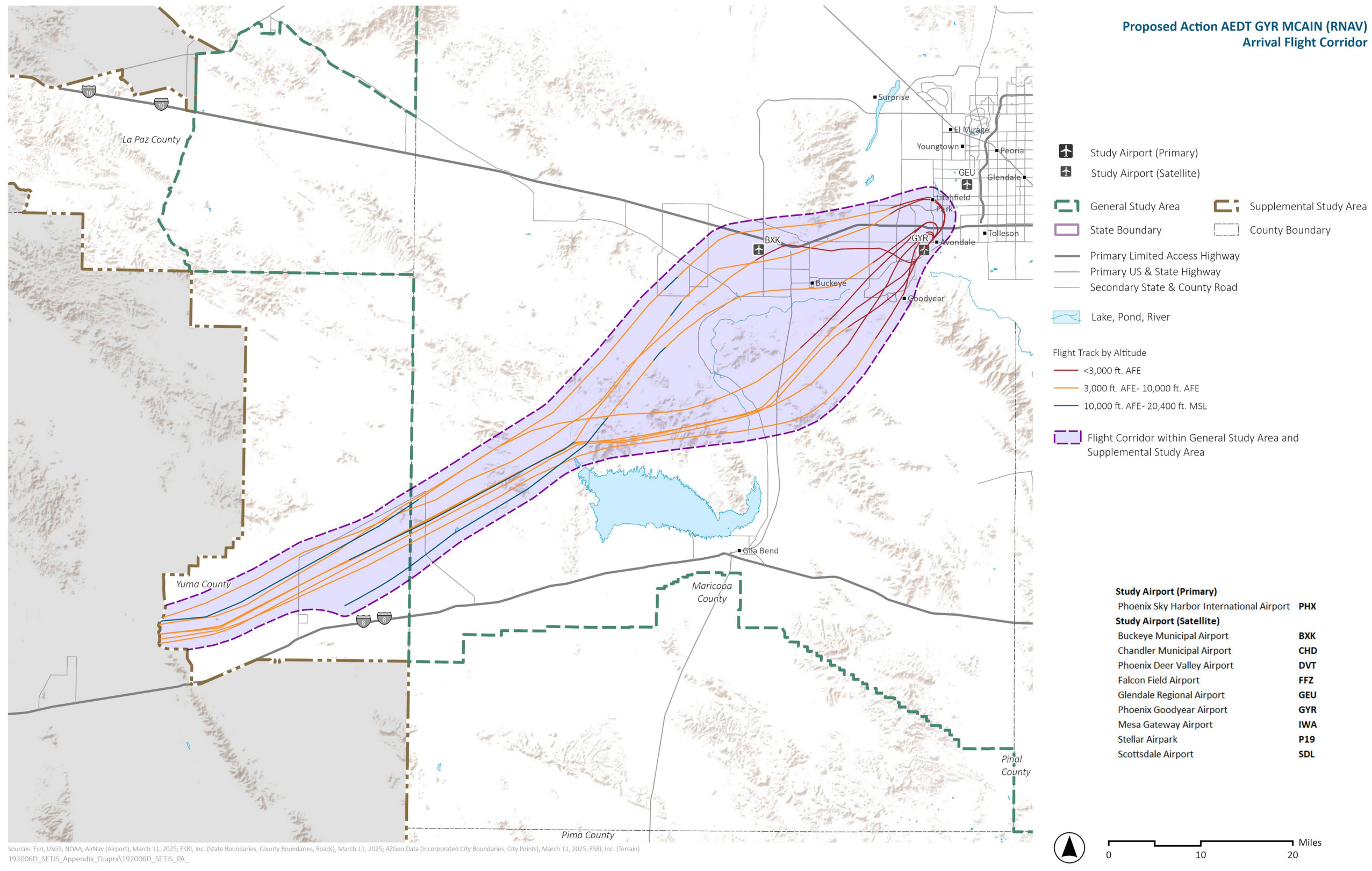
Exhibit I.7-2. Proposed Action AEDT GYR MCAIN (RNAV) Arrival Flight Corridor
