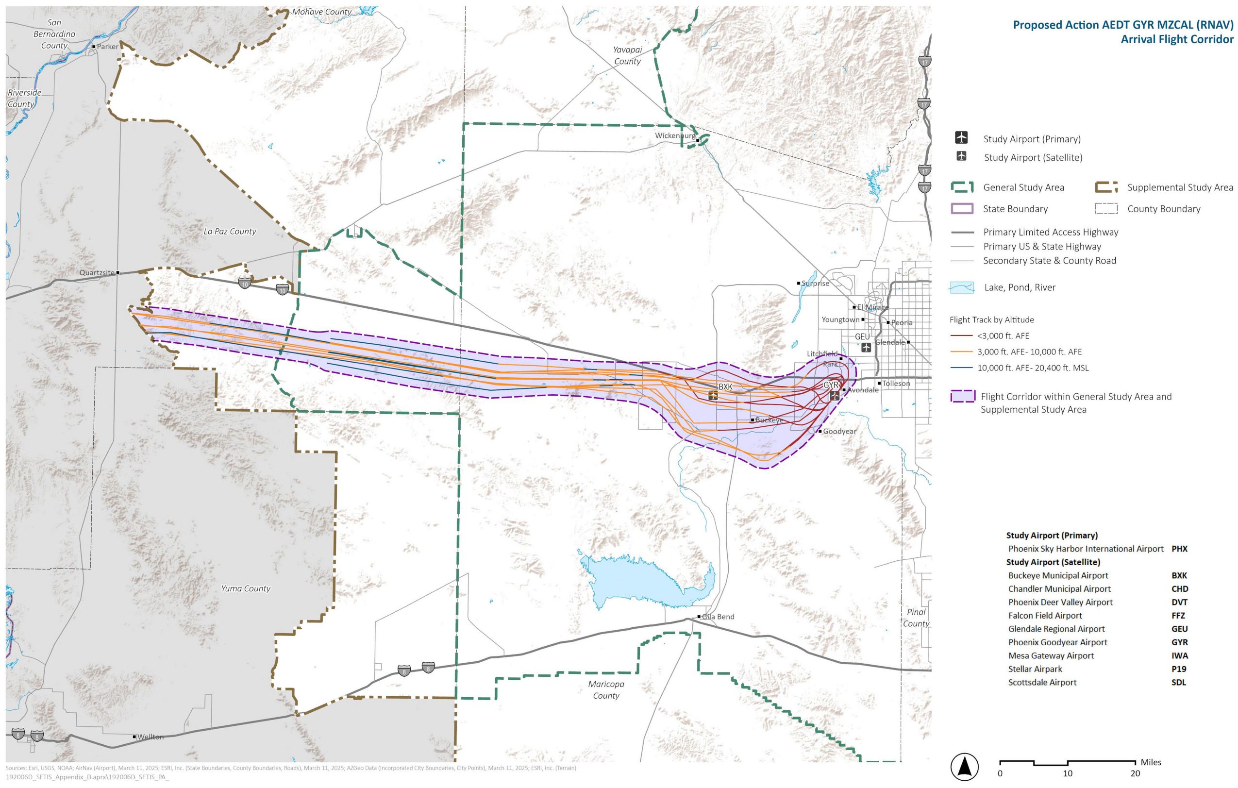
Exhibit I.7-3. Proposed Action AEDT GYR MZCAL (RNAV) Arrival Flight Corridor
