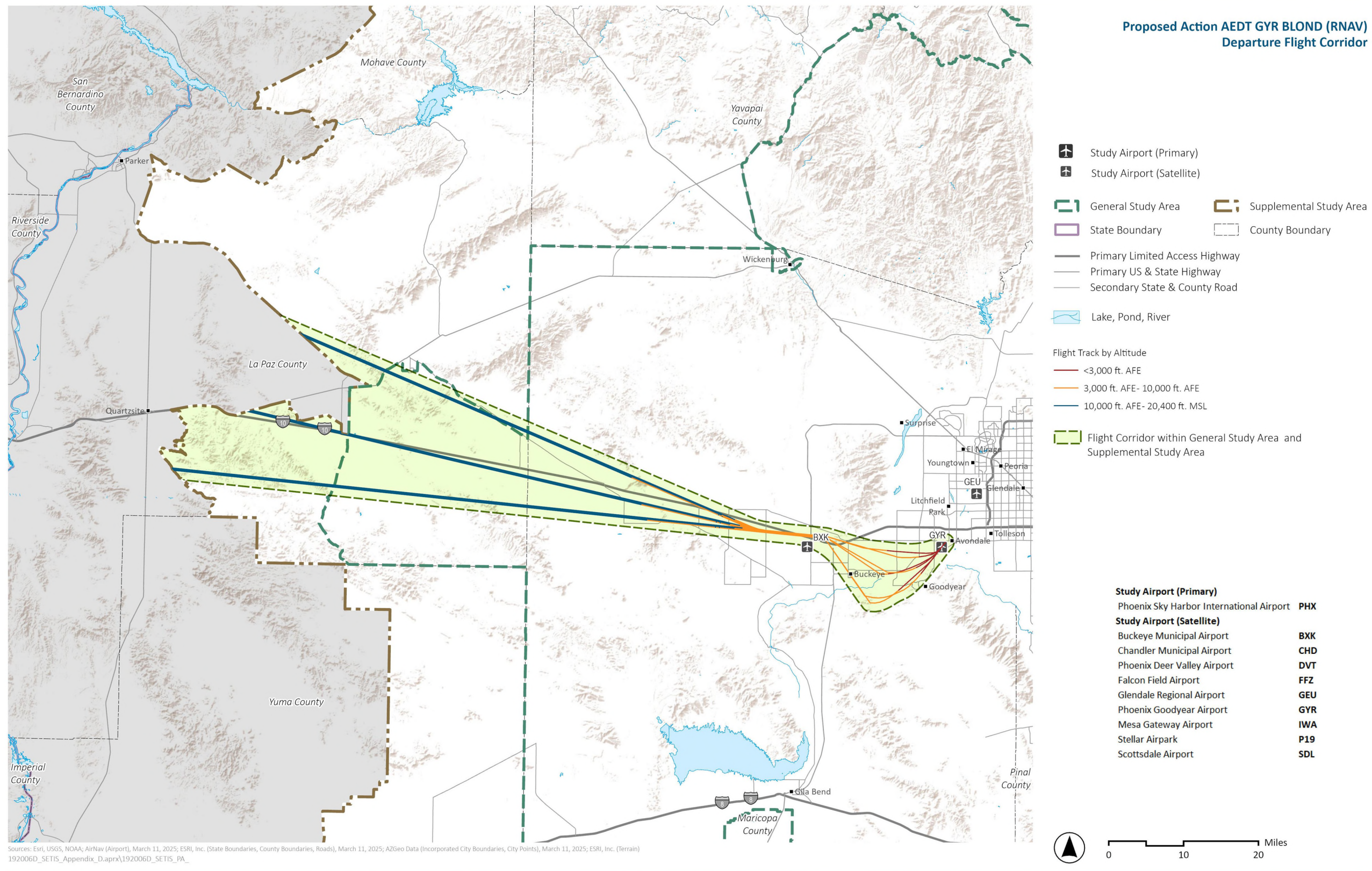
Exhibit I.7-6. Proposed Action AEDT GYR BLOND (RNAV) Departure Flight Corridor
