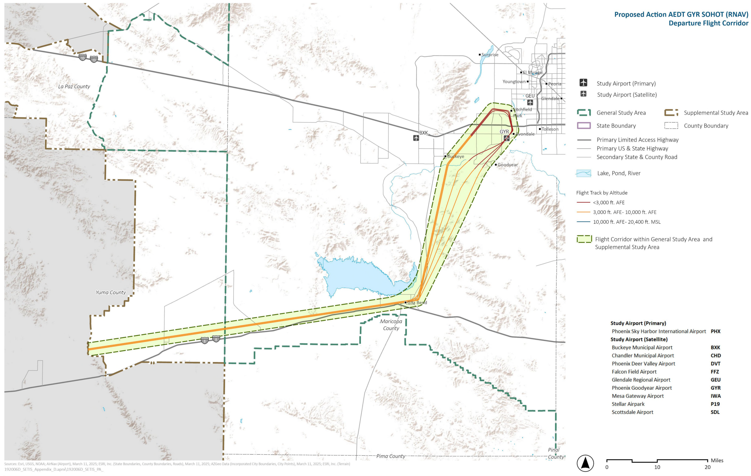
Exhibit I.7-10. Proposed Action AEDT GYR SOHOT (RNAV) Departure Flight Corridor
