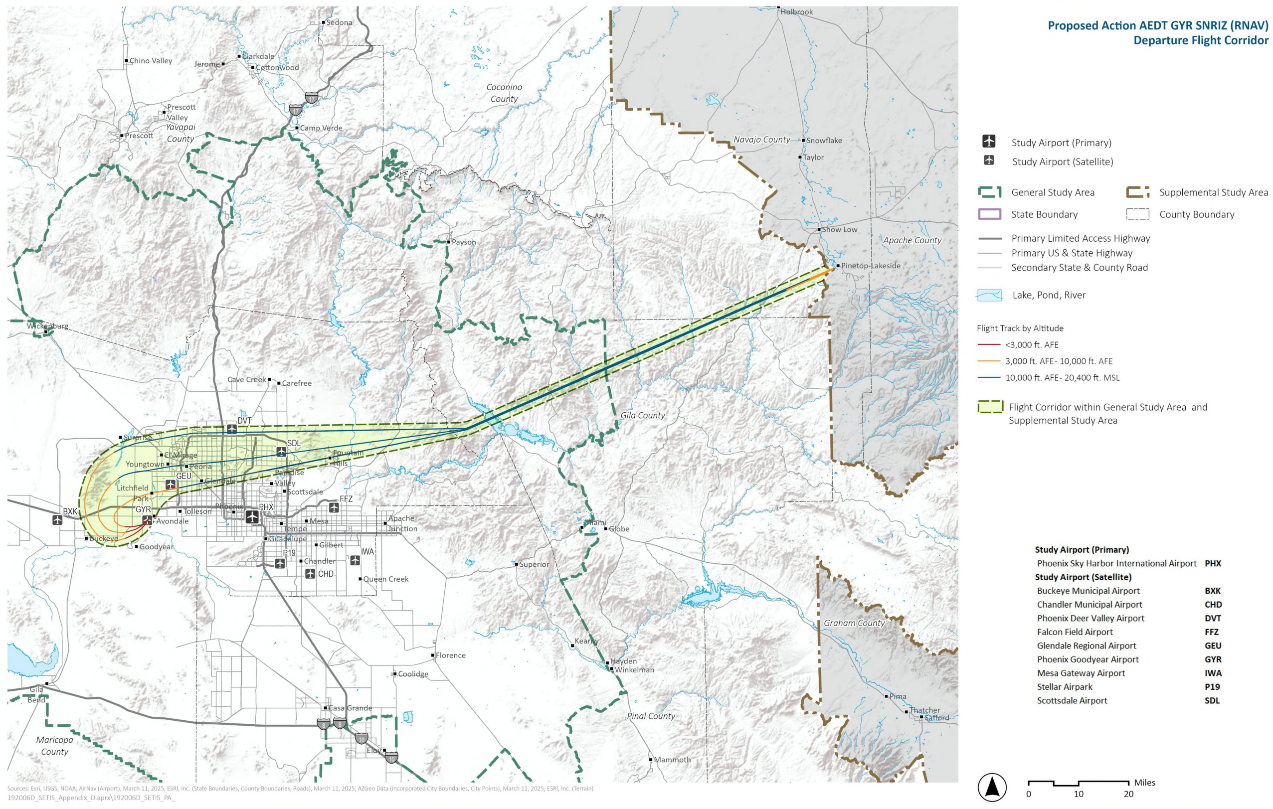
Exhibit I.7-9. Proposed Action AEDT GYR SNRIZ (RNAV) Departure Flight Corridor
