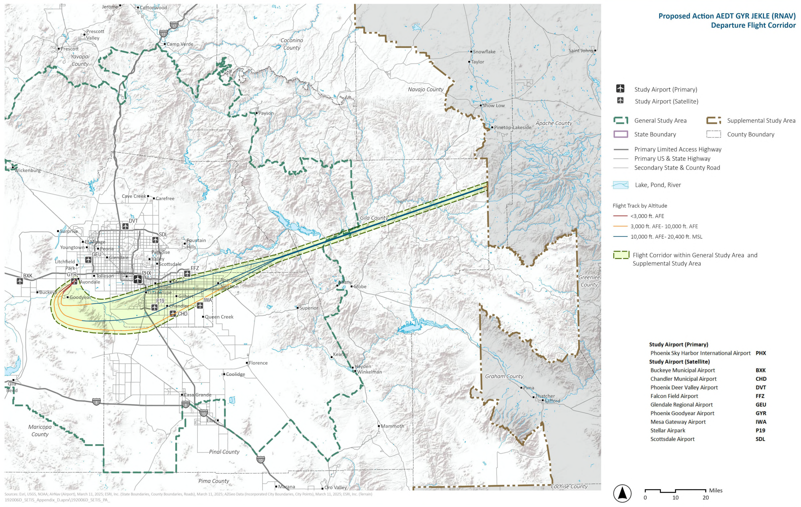
Exhibit I.7-7. Proposed Action AEDT GYR JEKLE (RNAV) Departure Flight Corridor
