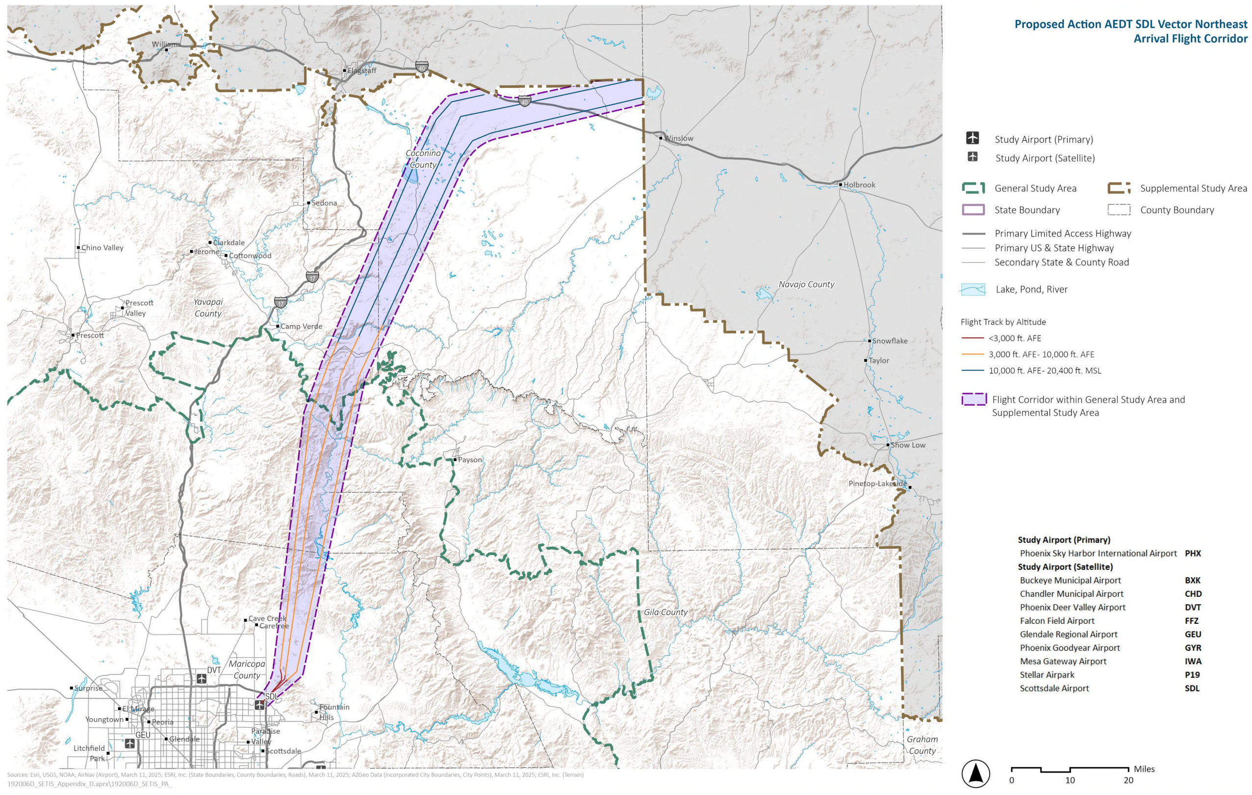
Exhibit I.10-5. Proposed Action AEDT SDL Vector Northeast Arrival Flight Corridor
