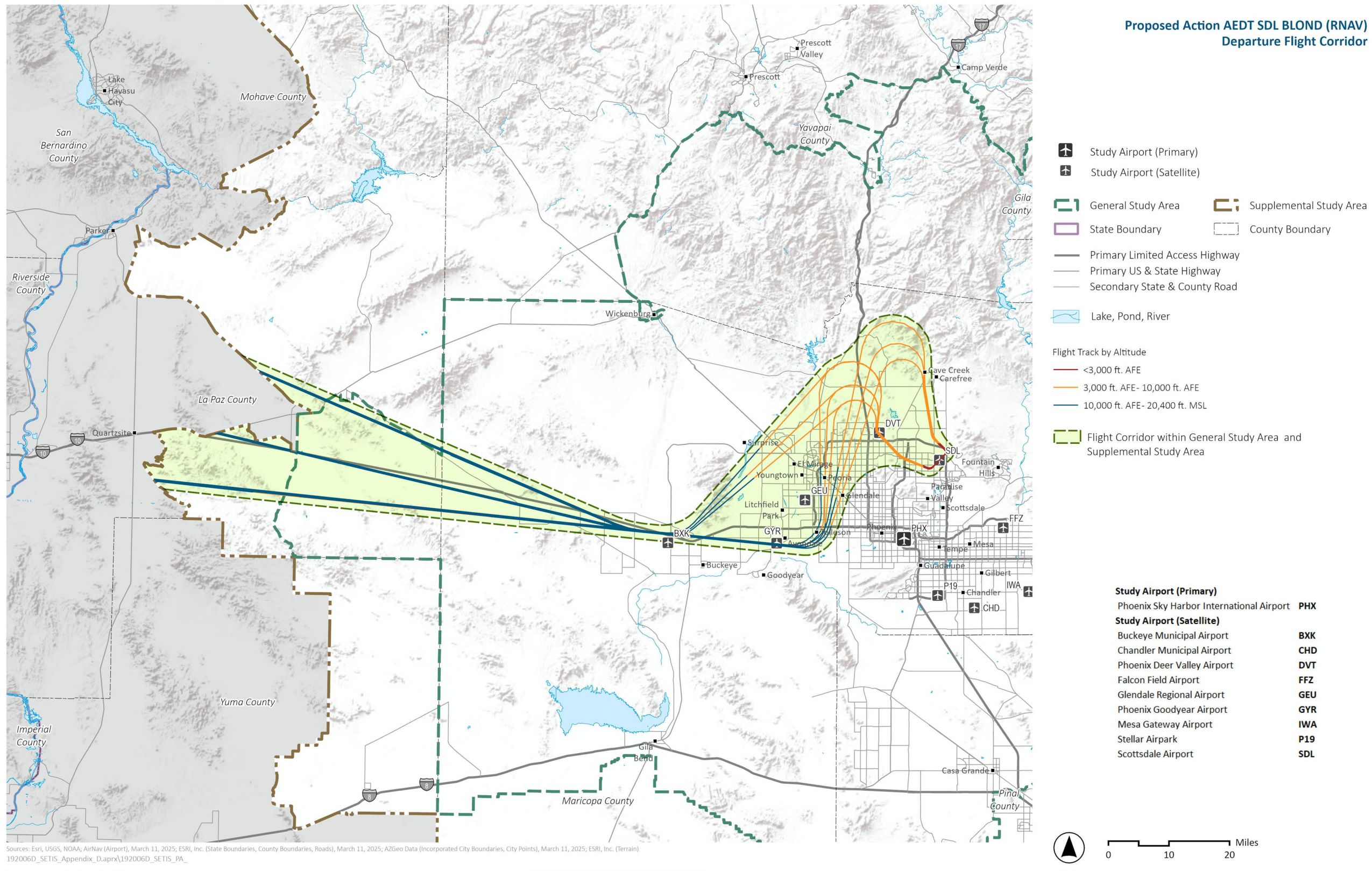
Exhibit I.10-8. Proposed Action AEDT SDL BLOND (RNAV) Departure Flight Corridor
