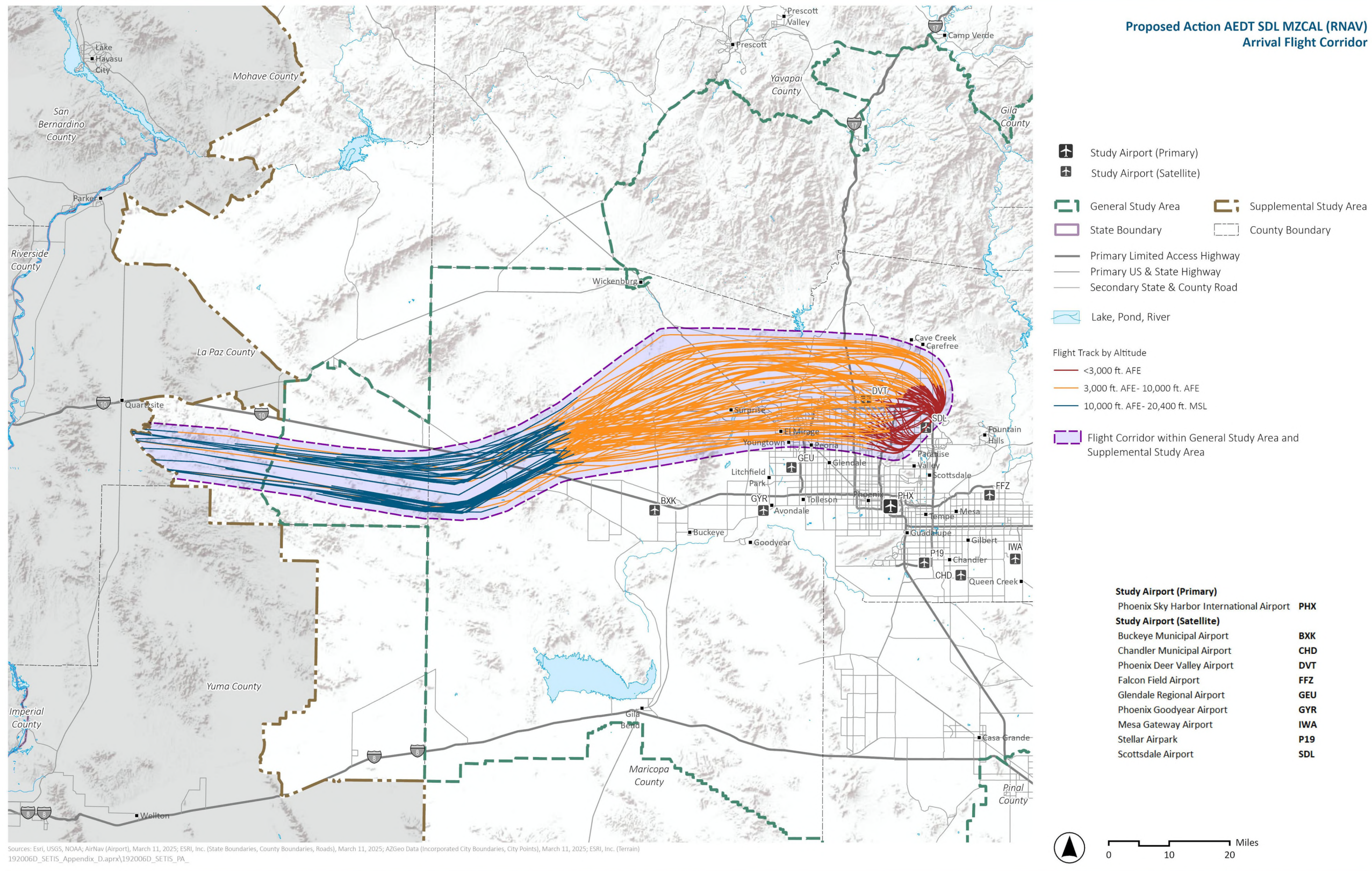
Exhibit I.10-4. Proposed Action AEDT SDL MZCAL (RNAV) Arrival Flight Corridor
