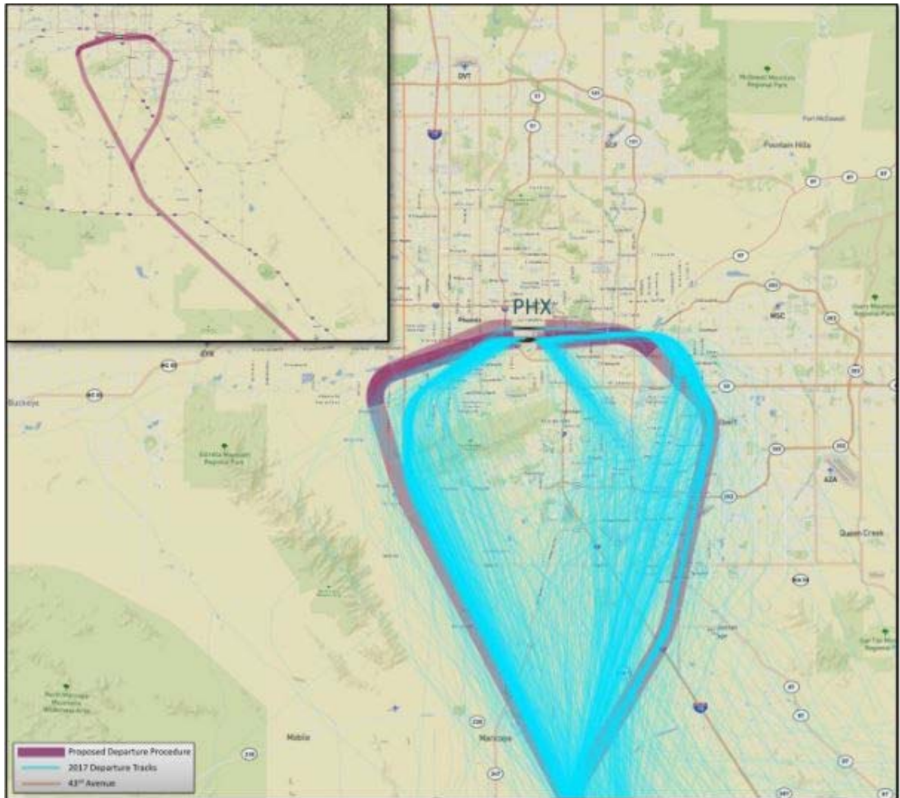
Figure B-7. STRRM RNAV Standard Instrument Departure
