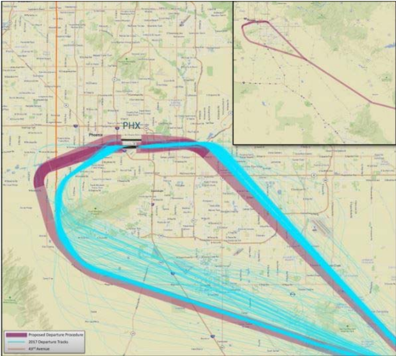
Figure B-6. ECLPS RNAV Standard Instrument Departure
