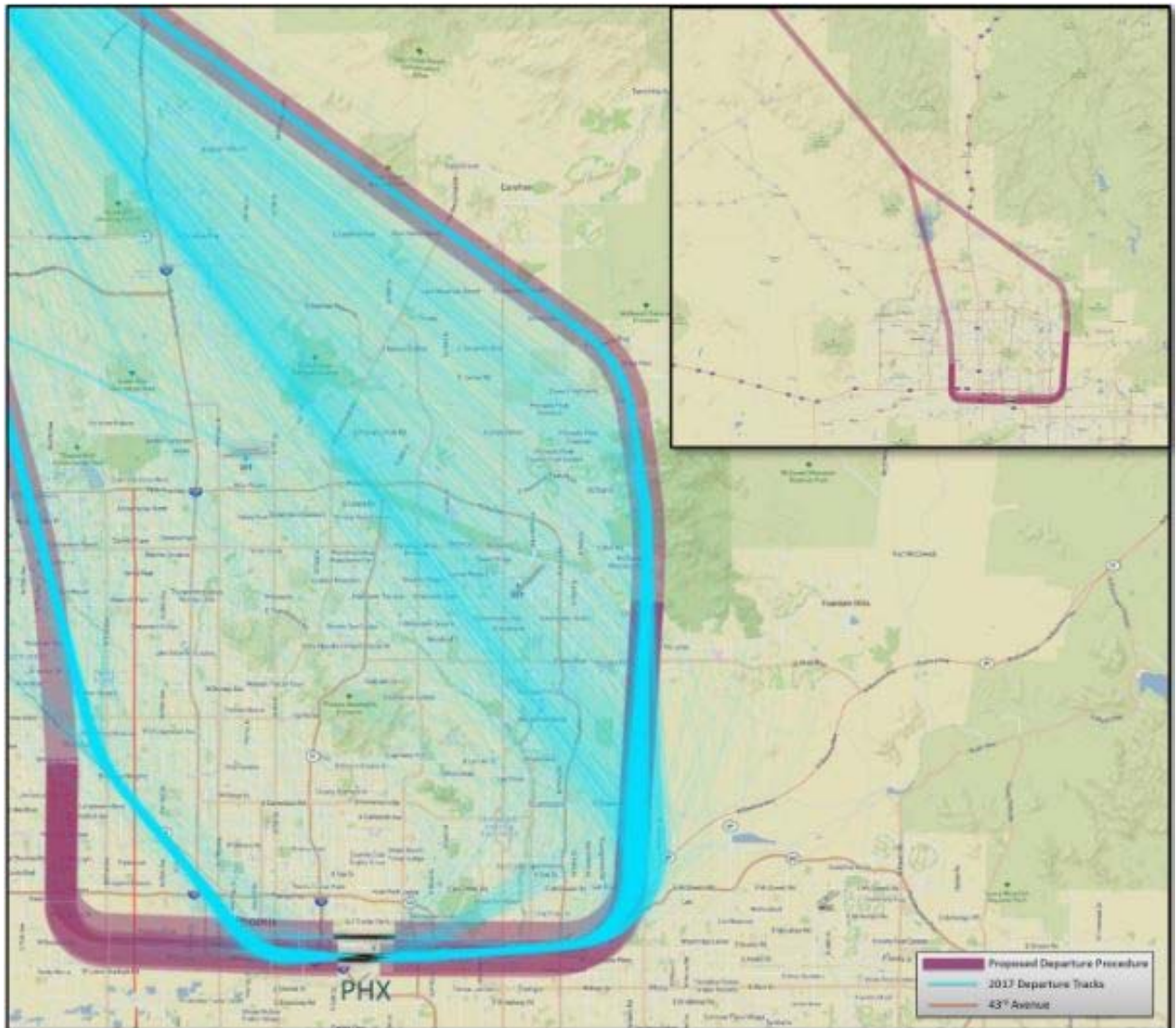
Figure B-1. ZEPER RNAV Standard Instrument Departure
