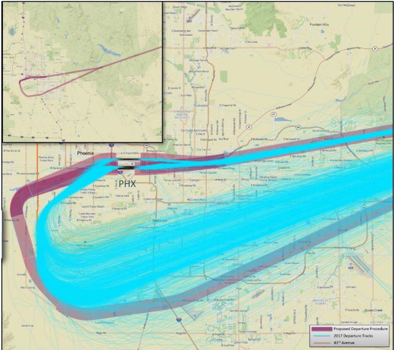
Figure B-5. BROAK RNAV Standard Instrument Departure
