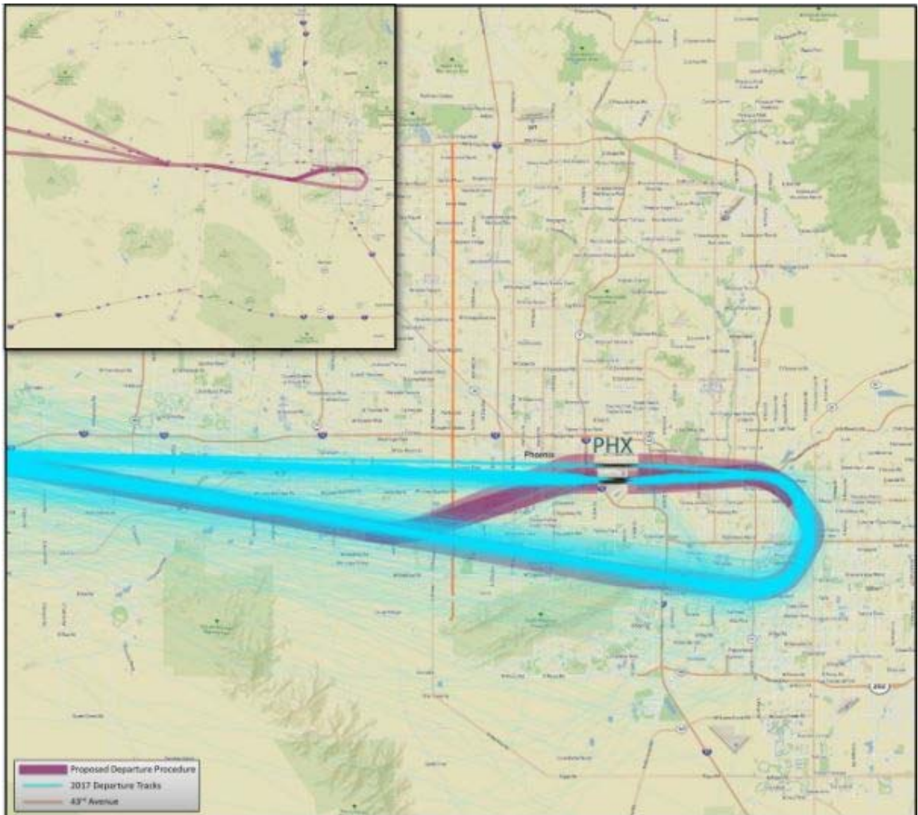
Figure B-9. KEENS RNAV Standard Instrument Departure
