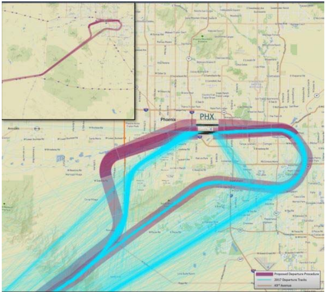
Figure B-8. FYRBD RNAV Standard Instrument Departure
