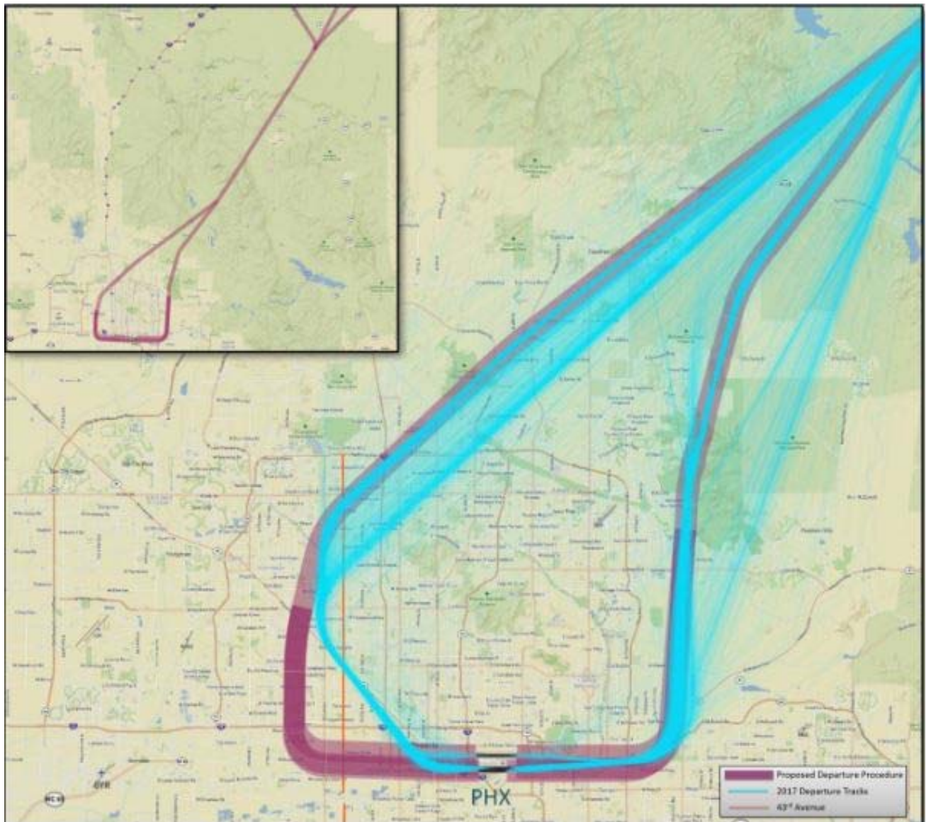
Figure B-3. MRBIL RNAV Standard Instrument Departure
