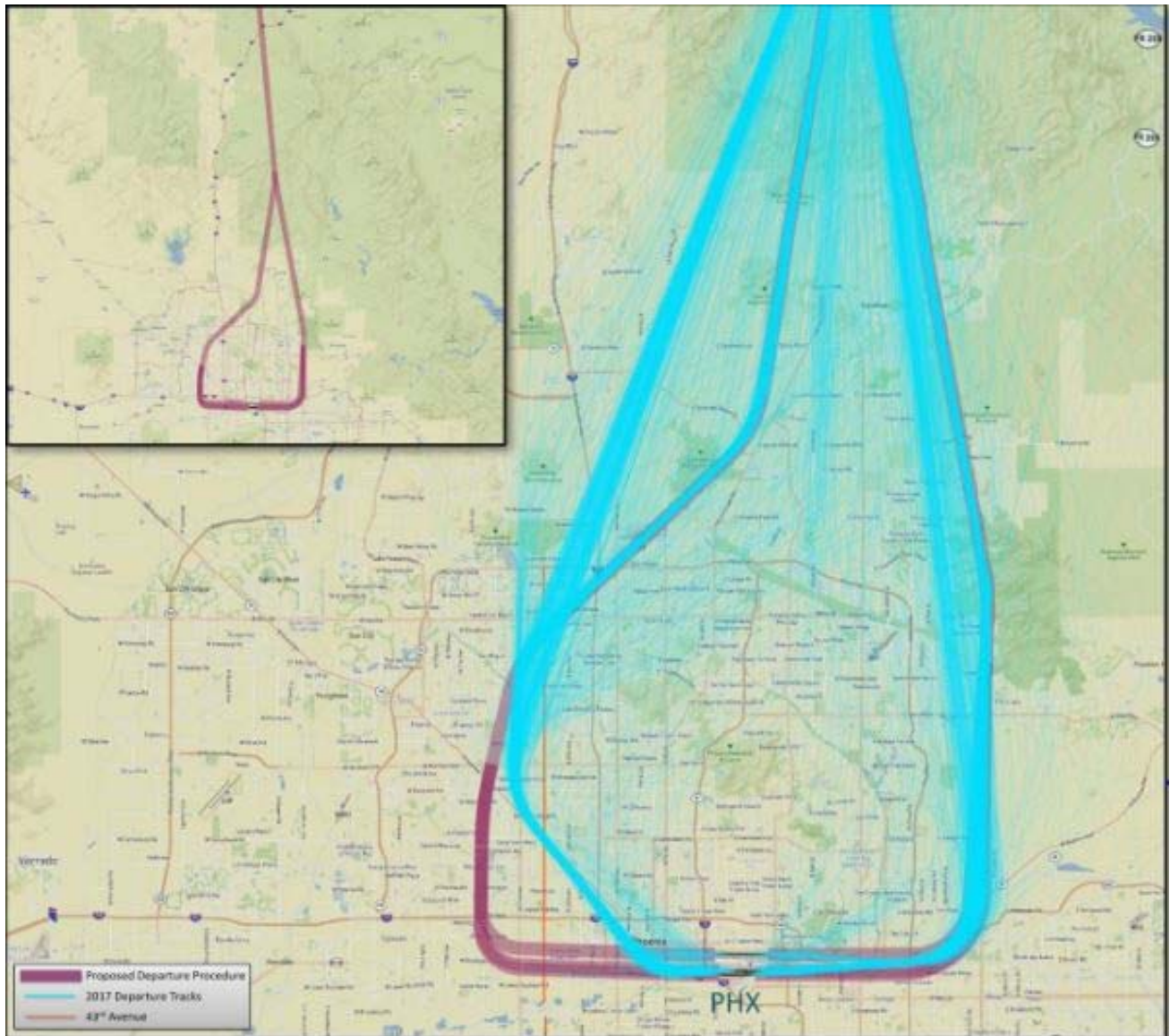
Figure B-2. QUAKY RNAV Standard Instrument Departure
