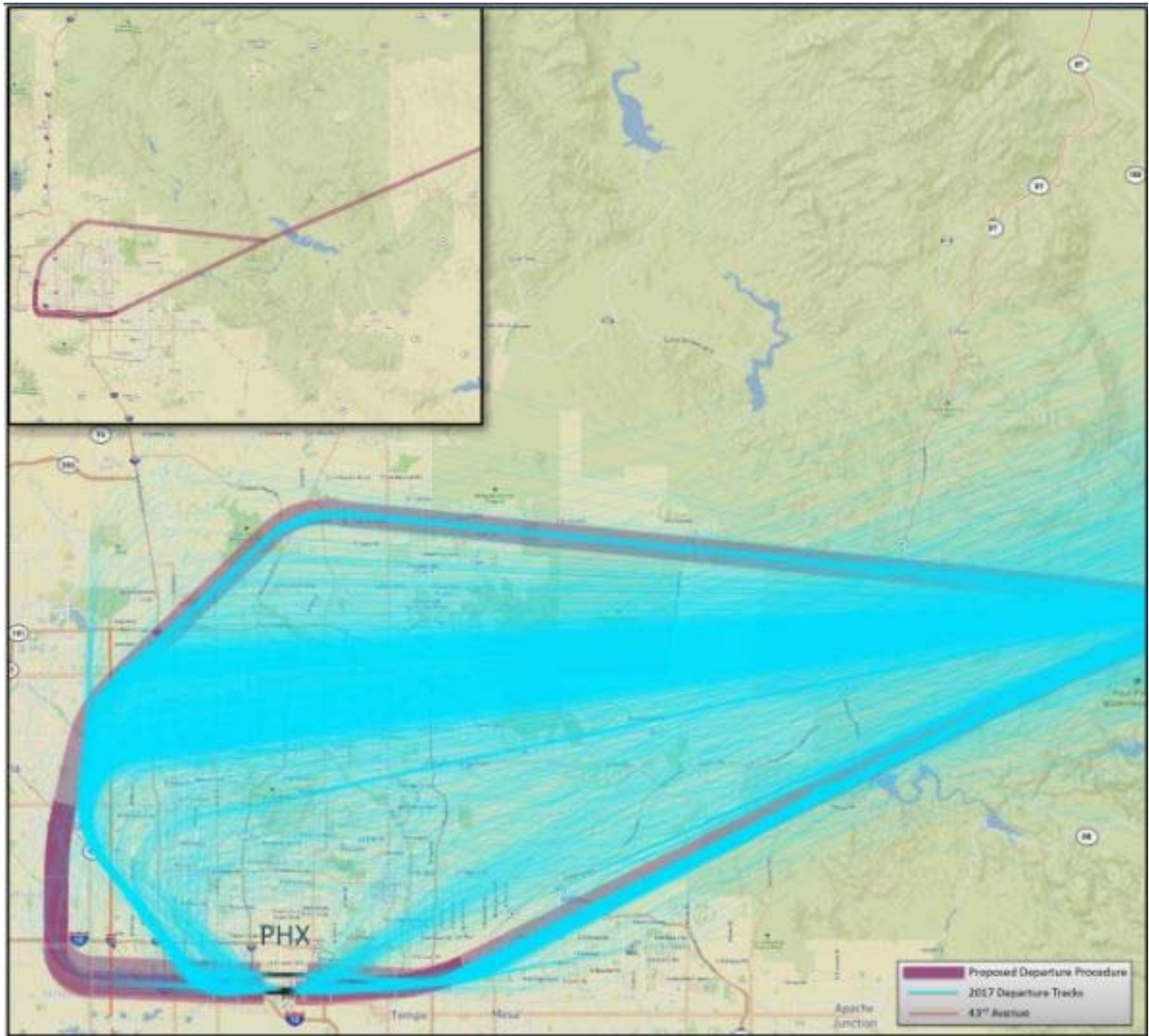
Figure B-4. FORPE RNAV Standard Instrument Departure
