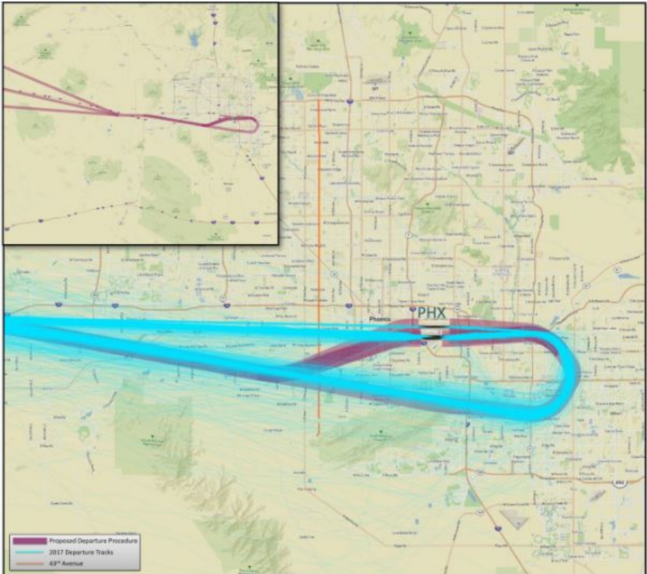
Figure D-5. KEENS RNAV SID – Departure route to the west
