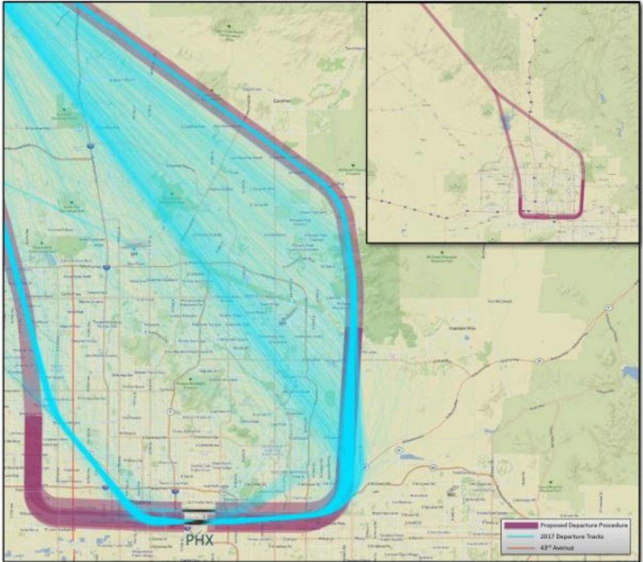
Figure D-1. ZIDOG RNAV SID – Departure route to the northwest
