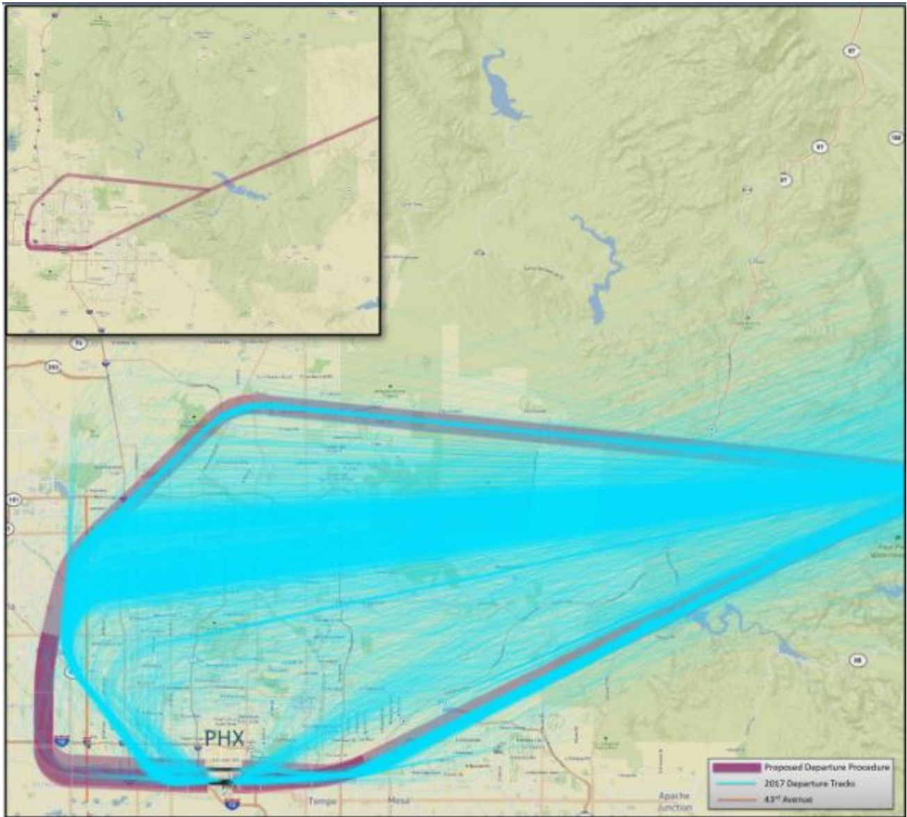
Figure D-4. ZIDOG RNAV SID – Departure route to the east
