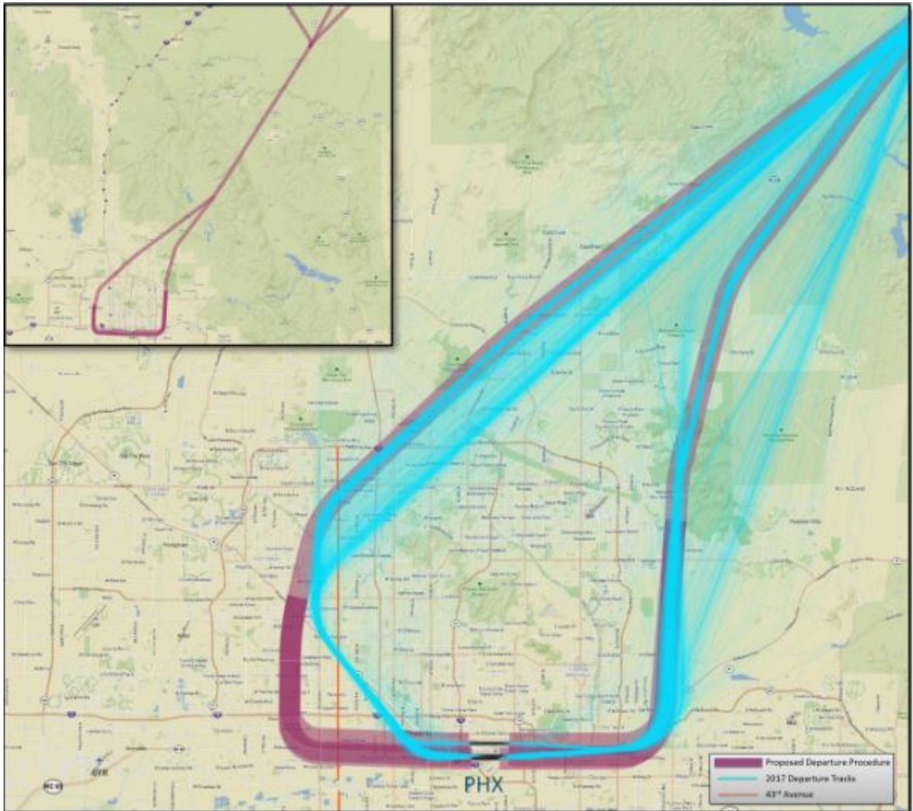
Figure D-3. ZIDOG RNAV SID – Departure route to the northeast
