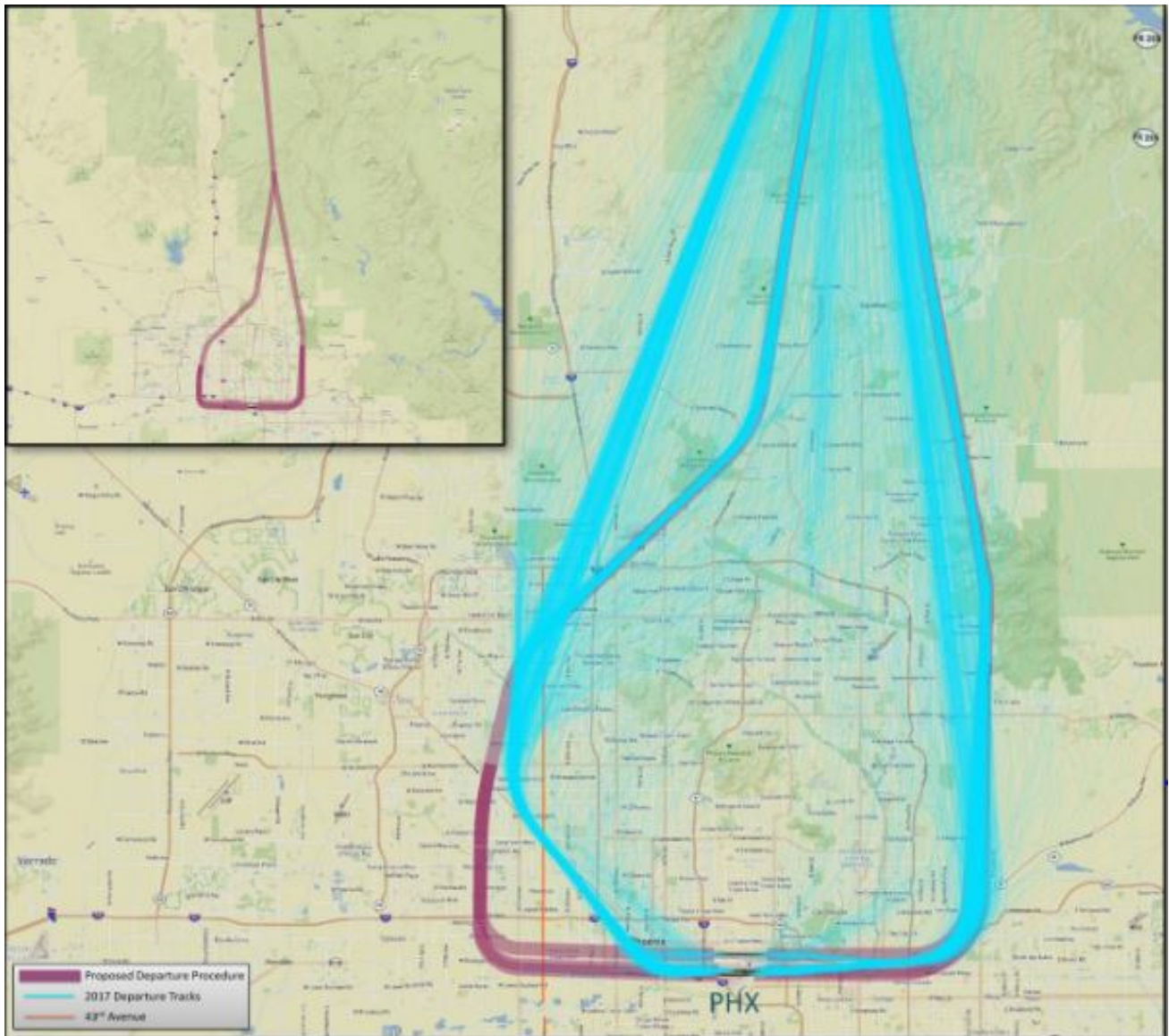
Figure D-2. ZIDOG RNAV SID – Departure route to the north
