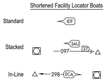
Figure 3.203 Facility Locator Boats in Congested Areas
