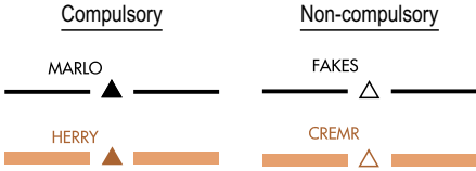
Figure 3.190 Radio Fixes
