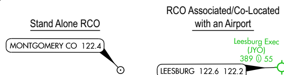
Figure 3.104 RCOs Not Associated with a NAVAID
