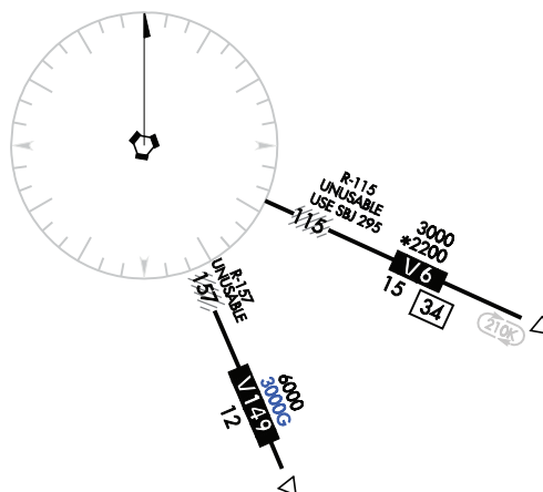
Figure 3.163 Unusable Radial
