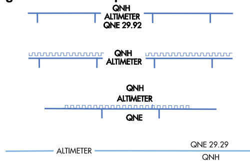
Figure 3.133 Example of Altimeter Settings
