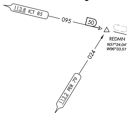
Figure 3.214 Offroute VHF Defined Fix Holding Pattern with Extended Radial Line
