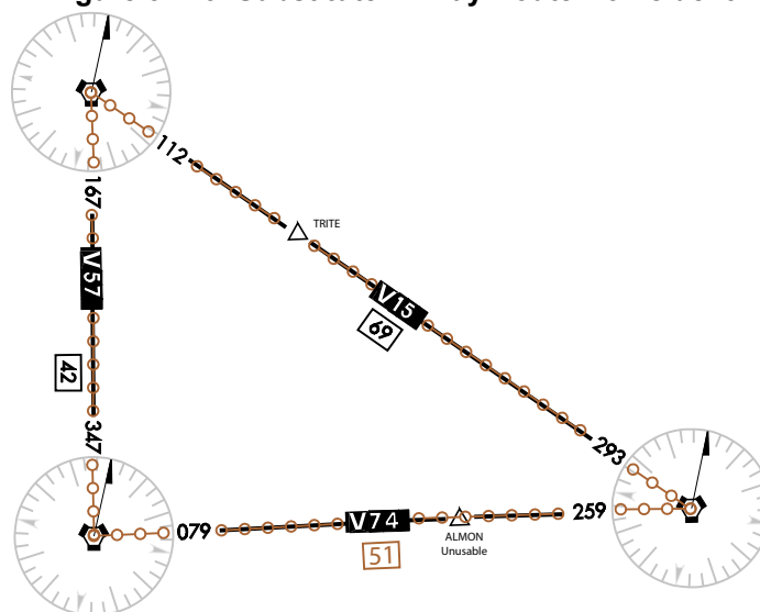
Figure 3.149 Substitute Airway/Route Coincident
