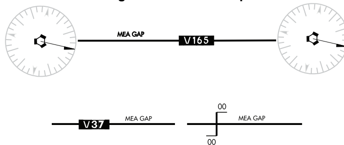
Figure 3.171 MEA Gap
