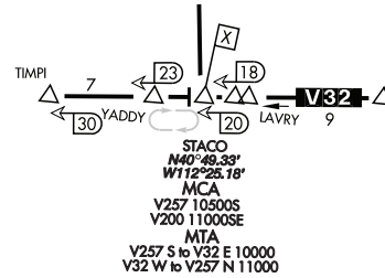
Figure 3.174 MCA &amp; MTA Data Complex Example
