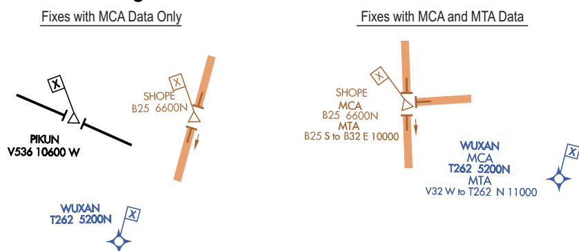
Figure 3.173 MCA and MTA Data at a Fix
