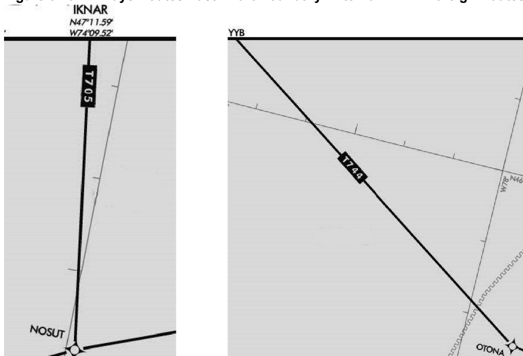
Figure 3.40 Airways/Routes Past Chart Boundary-External-RNAV Foreign Routes
