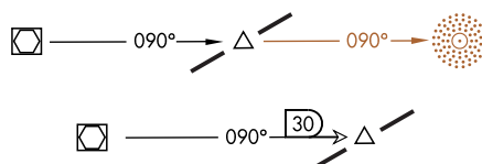
Figure 3.196 NAVAIDs Used for Fix Makeups
