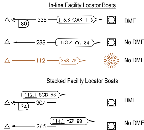
Figure 3.201 Facility Locator Boats
