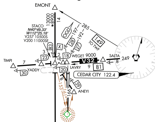
Figure 3.176 MCA in a Congested Area with Leader Line
