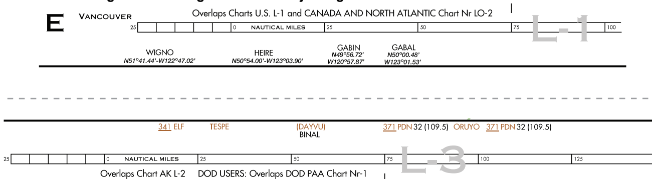
Figure 3.50 Margin Notes for Adjoining Charts - Canadian and DoD Charts
