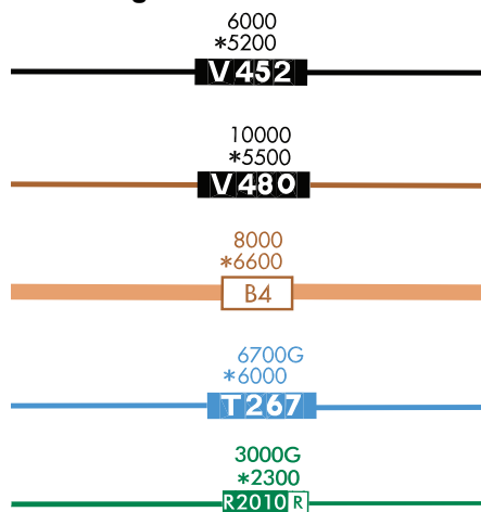
Figure 3.166 MOCAs
