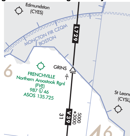
Figure 3.228 Foreign Airways/Routes
