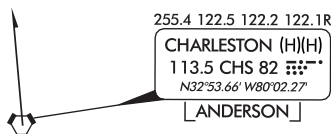
Figure 3.91 VORTAC
