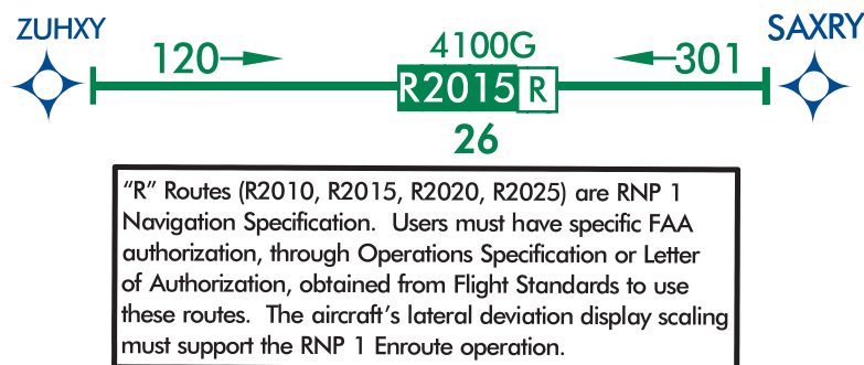
Figure 3.154 R Routes
