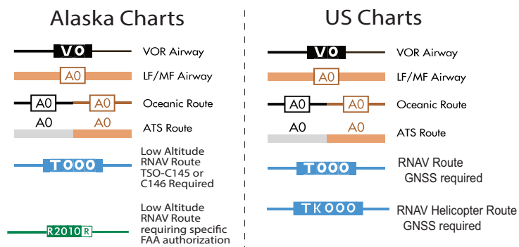
Figure 3.156 Route Identifications
