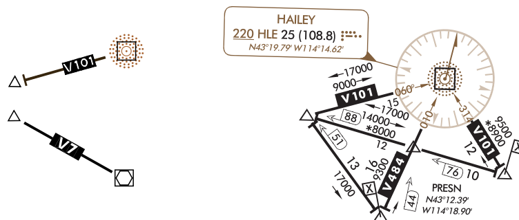
Figure 3.137 Victor Airways
