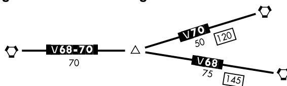
Figure 3.182 Box Mileages - Coincidental Routes
