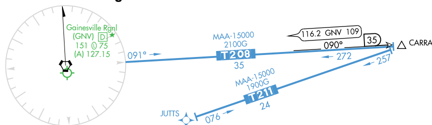
Figure 3.141 RNAV T and TK Routes
