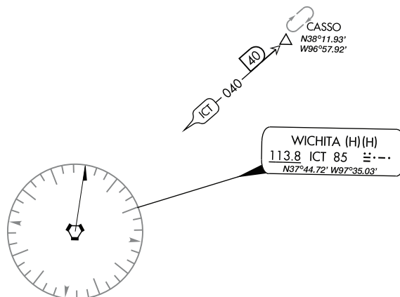
Figure 3.215 Off Route VHF Defined Fix Holding Pattern
