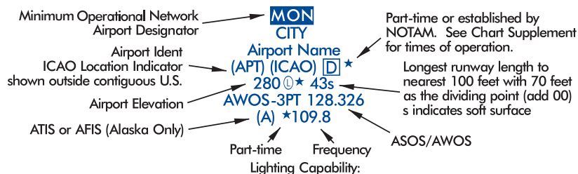
Figure 3.67 Airport Data Block
