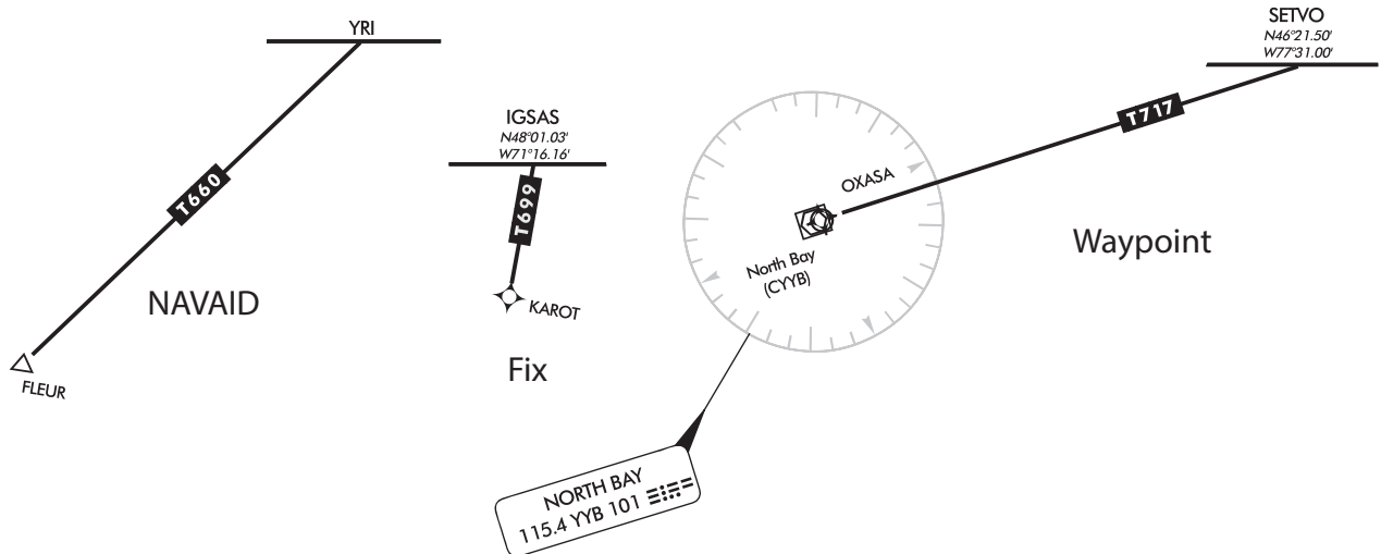
Figure 3.39 Airways/Routes Past Chart Boundary - External - RNAV Route
