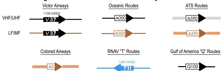
Figure 3.159 Preferred Direction Airways/Routes
