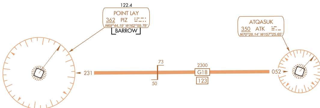
Figure 3.187 Changeover Points (COP) - LF/MF with DME
