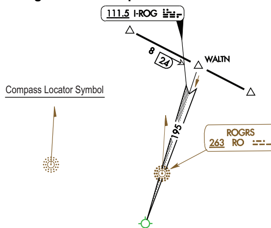
Figure 3.95 Compass Locator Beacon
