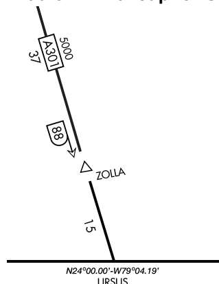
Figure 3.197 Radio Fix Makeup for Offshore Fixes
