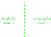
Figure 3.58 Time Zones
