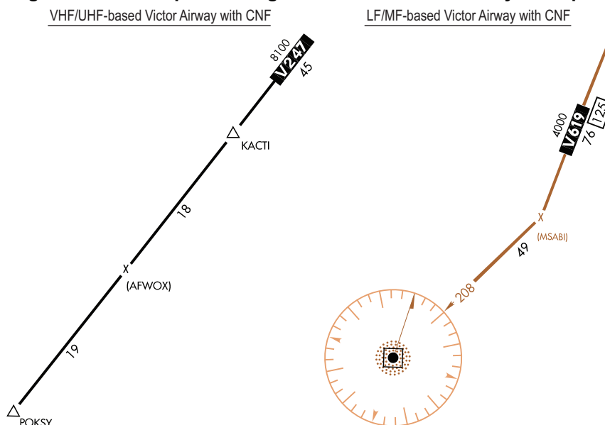
Figure 3.208 Computer Navigation Fixes - Victor Airway Examples
