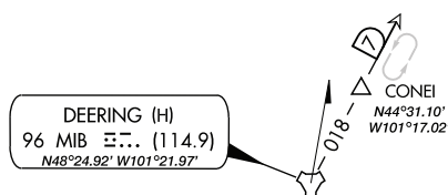
Figure 3.213 Off Route Holding Pattern Off a TACAN
