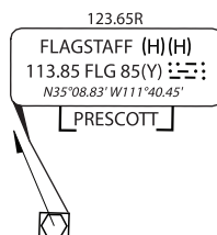
Figure 3.89 VOR/DME
