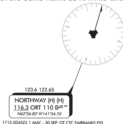
Figure 3.98 FSSs with the Same Name as NAVAID and Not Designated RCO
