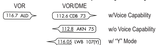
Figure 3.199 VOR and VOR/DME Capability Facility Locator Boats
