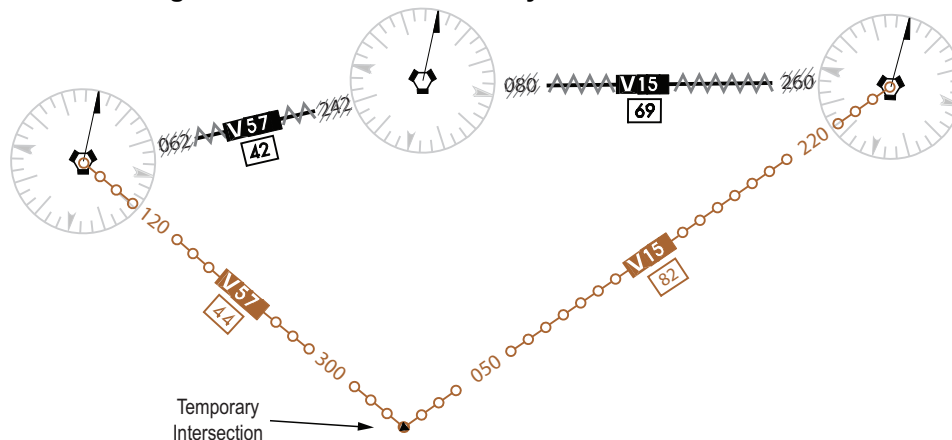
Figure 3.148 Substitute Airway/Route Non Coincident
