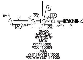
Figure 3.173 MCA &amp; MTA Data Complex Example
