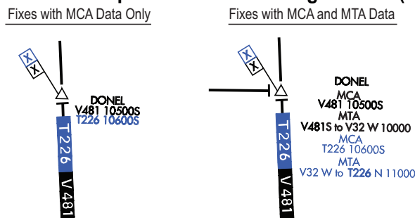
Figure 3.176 Multiple Minimum Crossing Altitude (MCAs)
