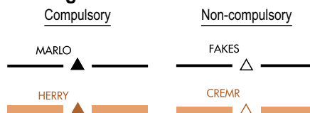
Figure 3.189 Radio Fixes
