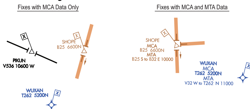
Figure 3.172 MCA and MTA Data at a Fix
