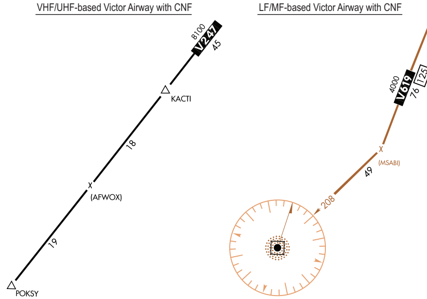
Figure 3.207 Computer Navigation Fixes - Victor Airway Examples
