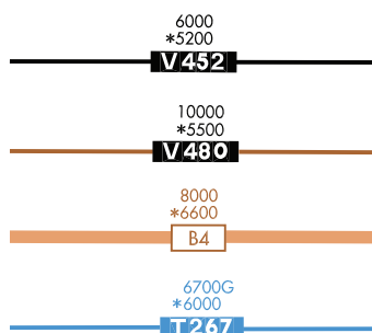
Figure 3.165 MOCAs
