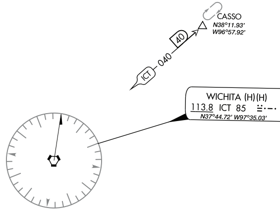
Figure 3.214 Off Route VHF Defined Fix Holding Pattern
