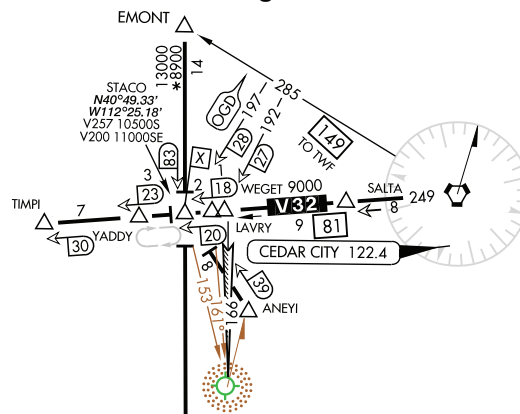
Figure 3.175 MCA in a Congested Area with Leader Line
