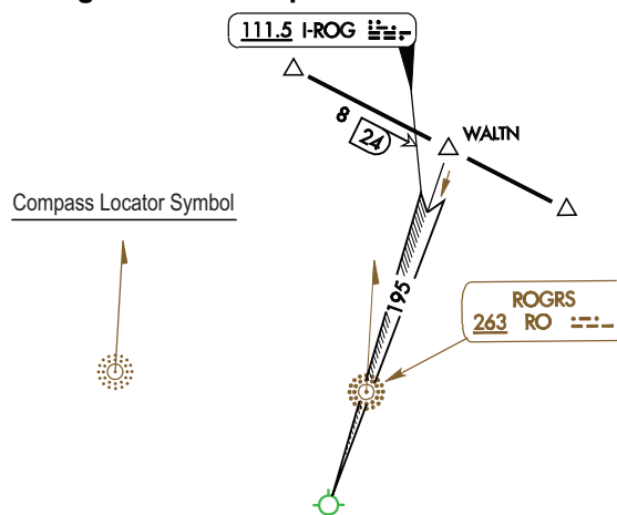
Figure 3.95 Compass Locator Beacon
