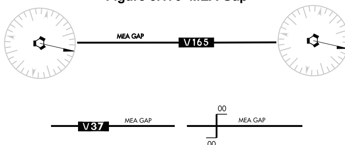
Figure 3.170 MEA Gap
