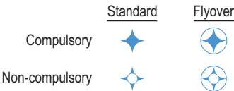
Figure 3.204 RNAV Waypoints Reporting & Flyover Function
