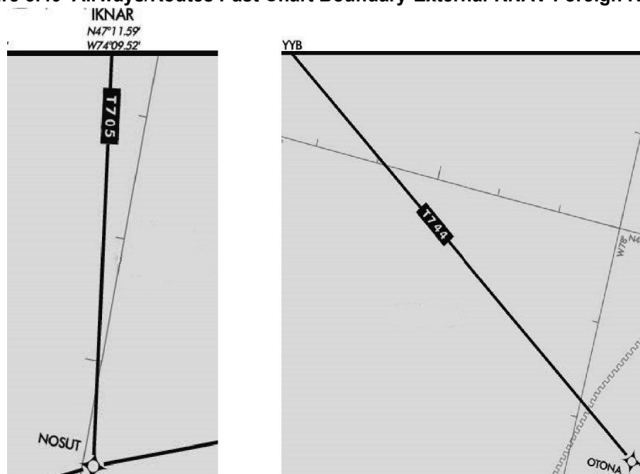
Figure 3.40 Airways/Routes Past Chart Boundary-External-RNAV Foreign Routes
