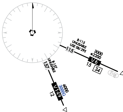
Figure 3.162 Unusable Radial
