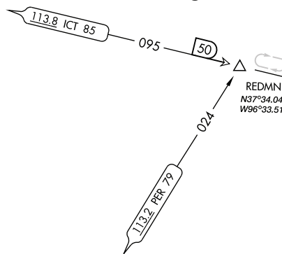
Figure 3.213 Offroute VHF Defined Fix Holding Pattern with Extended Radial Line
