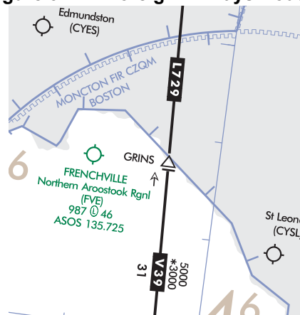
Figure 3.227 Foreign Airways/Routes
