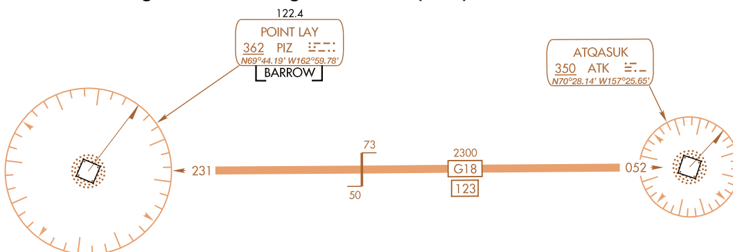
Figure 3.186 Changeover Points (COP) - LF/MF with DME
