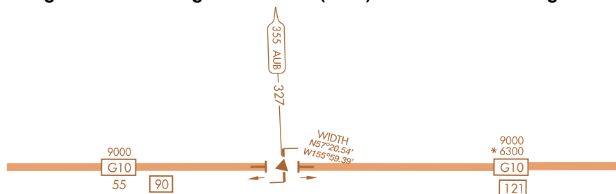
Figure 3.185 Changeover Points (COP) - LF/MF Establishing COP
