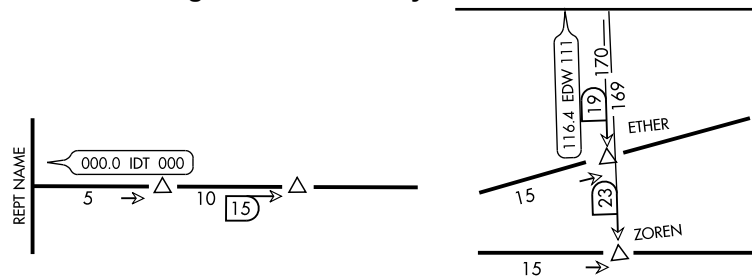
Figure 3.201 Facility Locator Boats
