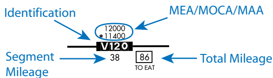
Figure 3.154 Airway/Route Data Grouping
