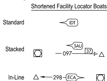
Figure 3.202 Facility Locator Boats in Congested Areas
