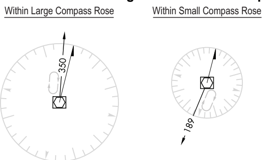
Figure 3.211 Off Route Holding Pattern within Compass Rose
