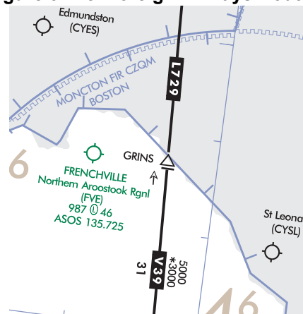
Figure 3.228 Foreign Airways/Routes
