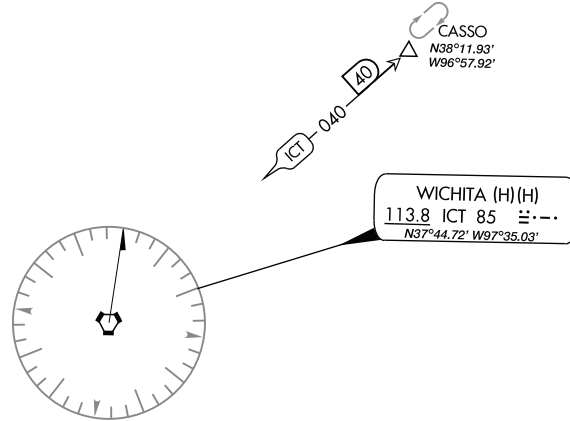
Figure 3.215 Off Route VHF Defined Fix Holding Pattern
