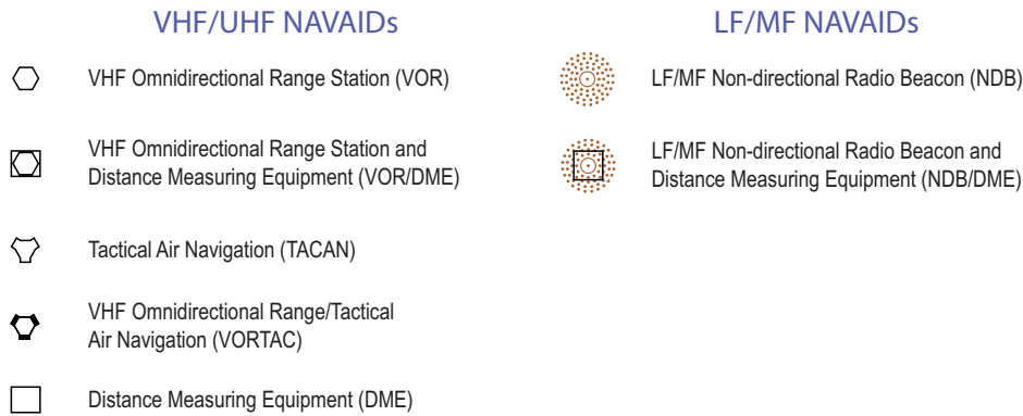
Figure 3.76 NAVAID Symbols
