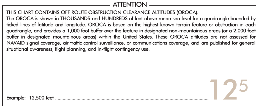
Figure 3.63 OROCA Notice
