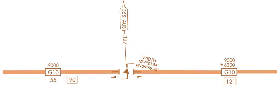
Figure 3.186 Changeover Points (COP) - LF/MF Establishing COP
