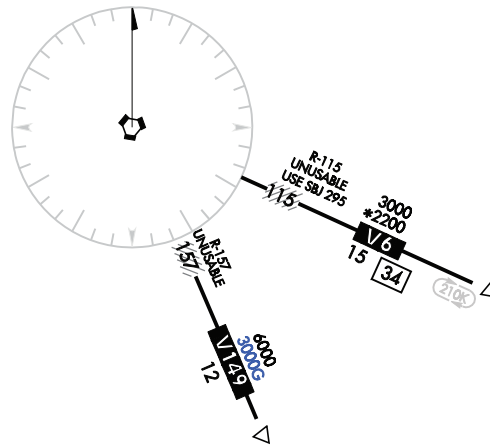
Figure 3.163 Unusable Radial
