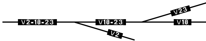
Figure 3.157 Coincidental Routes of the Same Classification
