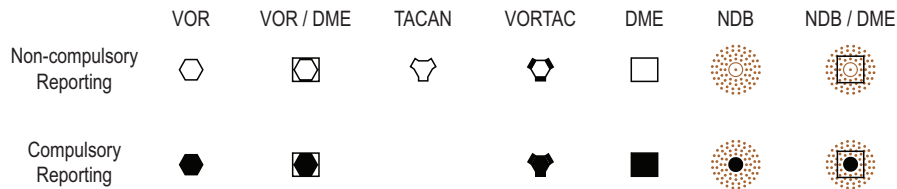
Figure 3.77 NAVAID Symbols with Compulsory and Non-Compulsory Reporting
