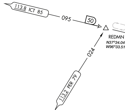
Figure 3.214 Offroute VHF Defined Fix Holding Pattern with Extended Radial Line
