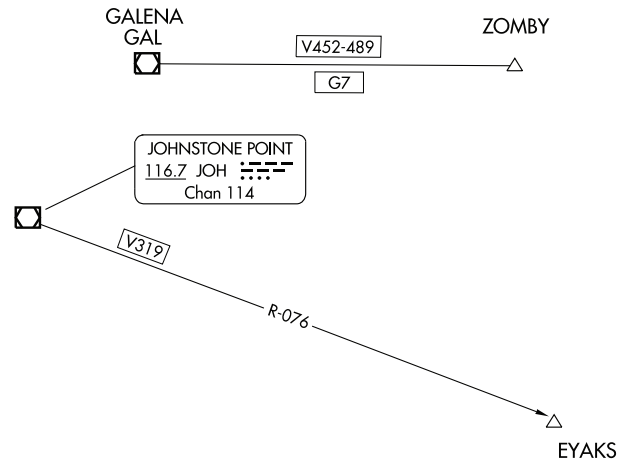
Figure 3.24 Non-Coincidental Routes
