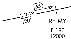
Figure 3.12 Unnamed DME Fix with Colocated CNF
