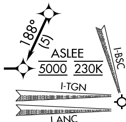
Figure 3.9 Localizer on RNAV STAR
