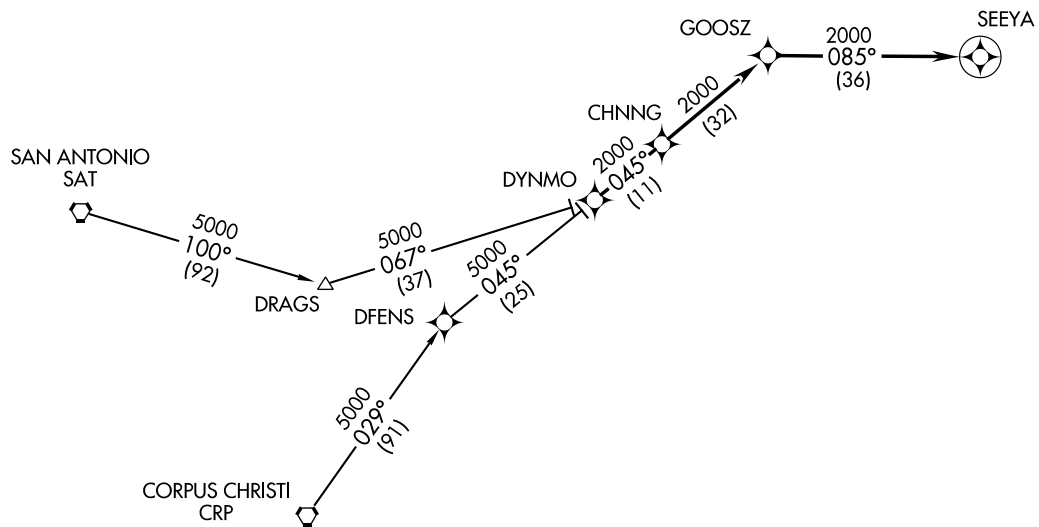
Figure 3.10 Waypoint Depiction
