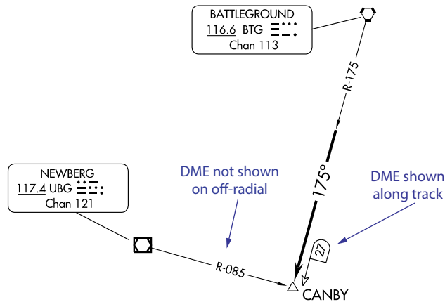
Figure 3.15 Off-Radial DME
