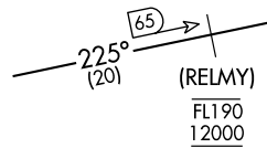
Figure 3.13 Un-Name DME Fix with Colocated CNF
