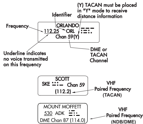
Figure 3.8 NAVAID Symbolization
