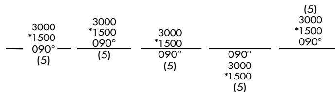
Figure 3.21 Route Data Stacking Order
