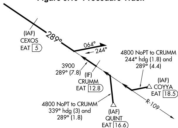
Figure 3.10 Procedure Track
