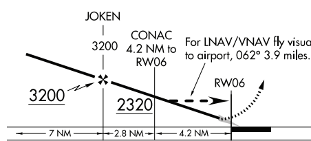
Figure 3.52 RNAV Fly Visual Example
