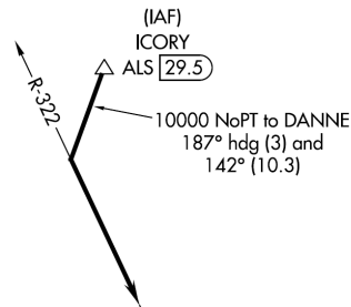
Figure 3.13 Dogleg Segment Based on Heading
