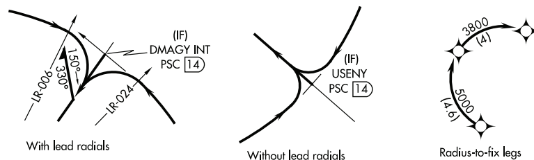
Figure 3.14 DME Arcs and RF Legs
