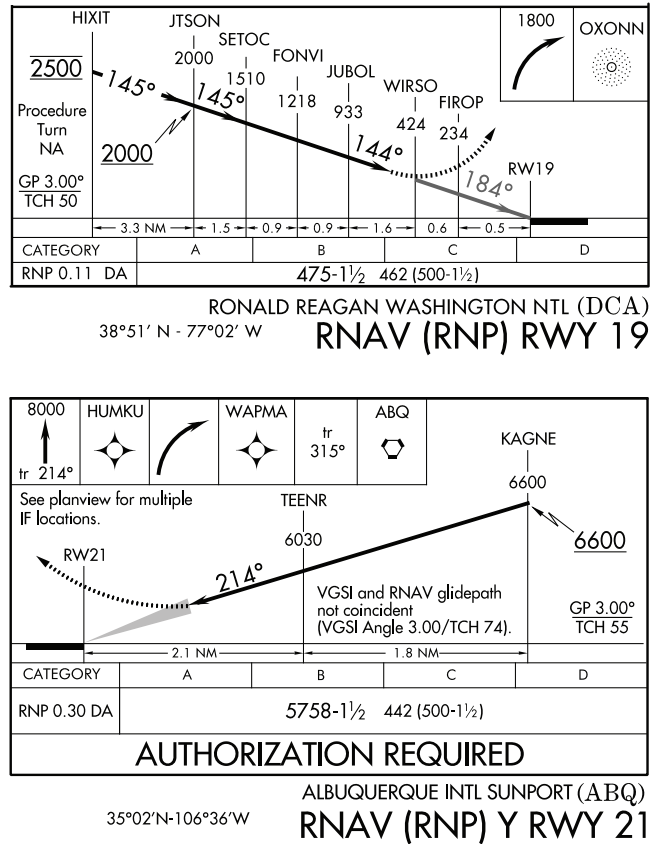
Figure 3.53 RNP Profile - Track to Fix (TF) and Radius to Fix (RF) Segments
