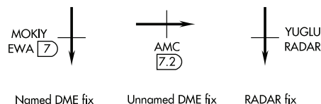
Figure 3.37 DME Fixes
