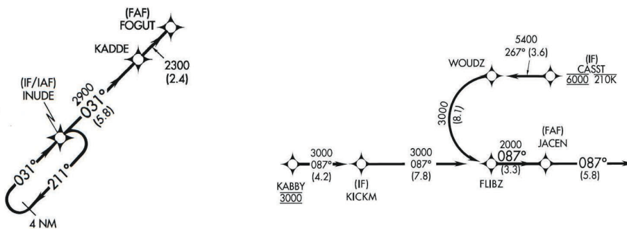
Figure 3.11 Procedure Track Type
