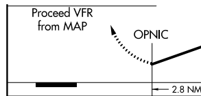
Figure 3.51 Copter VFR Segment
