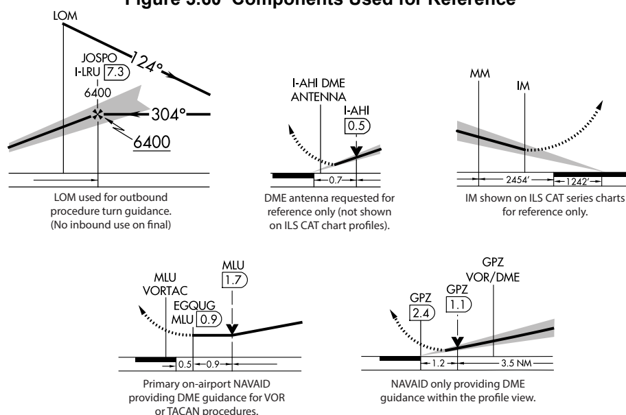
Figure 3.60 Components Used for Reference
