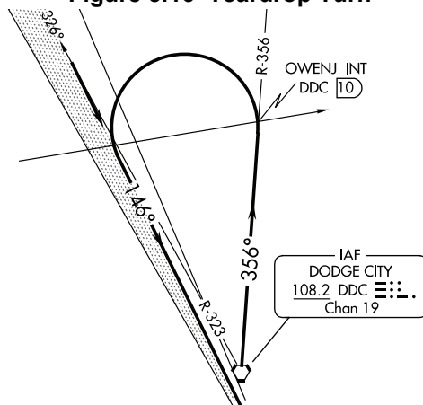
Figure 3.16 Teardrop Turn
