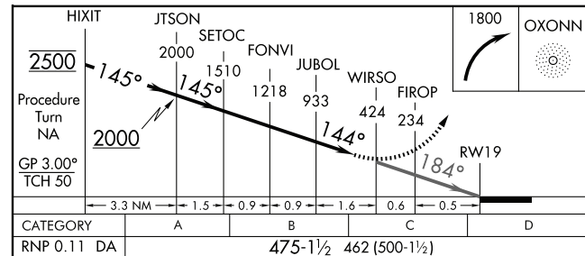
Figure 3.56 RNP Profile - Track to Fix (TF) and Radius to Fix (RF) Segments
