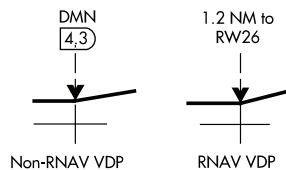
Figure 3.54 Visual Descent Point
