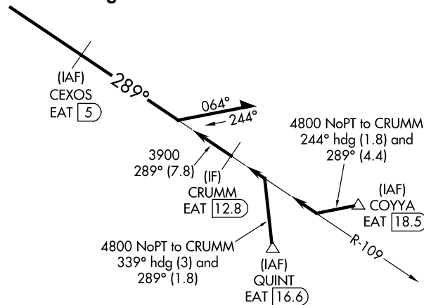
Figure 3.10 Procedure Track
