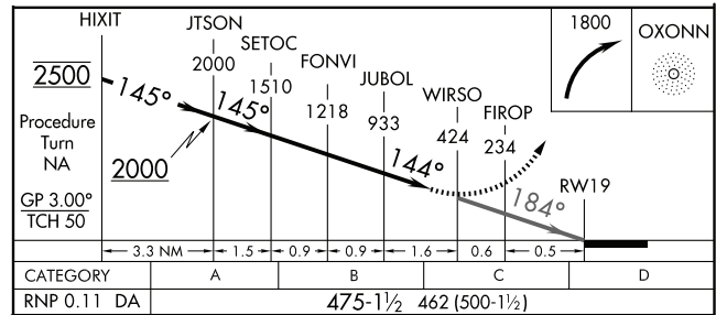
Figure 3.53 RNP Profile - Track to Fix (TF) and Radius to Fix (RF) Segments
