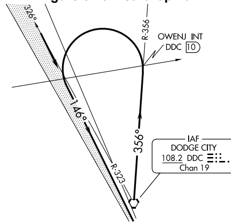
Figure 3.16 Teardrop Turn
