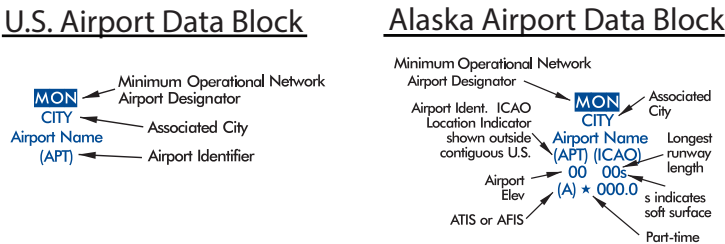
Figure 3.49 Airport Data Block
