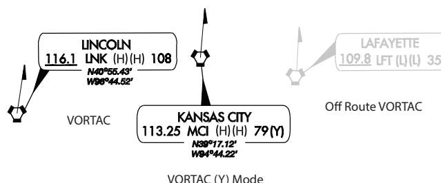
Figure 3.70 VORTAC
