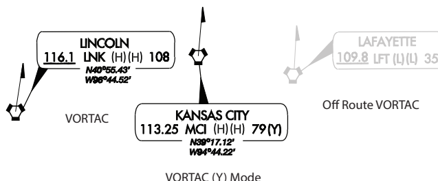
Figure 3.70 VORTAC
