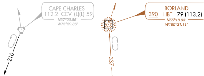
Figure 3.173 NAVAID Based-Off Route Holding Patterns - VHF/UHF & LF/MF
