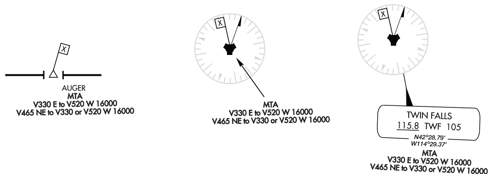
Figure 3.142 Minimum Crossing Altitudes (MCA) & Minimum Turning Altitude (MTA)
