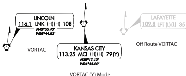
Figure 3.70 VORTAC
