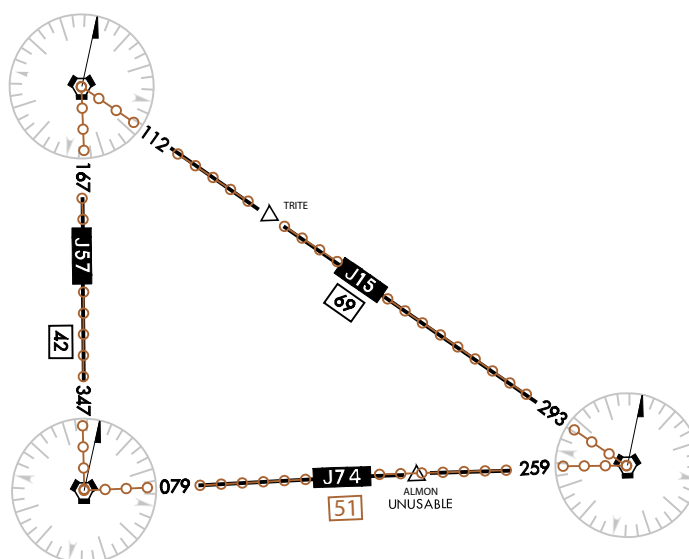
Figure 3.124 Substitute Routes Coincident
