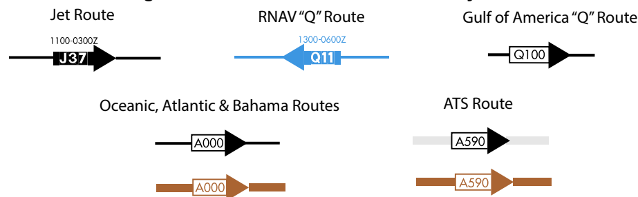
Figure 3.128 Preferred Direction Airways/Routes
