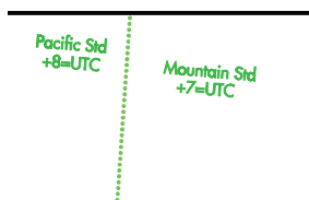
Figure 3.43 Time Zones
