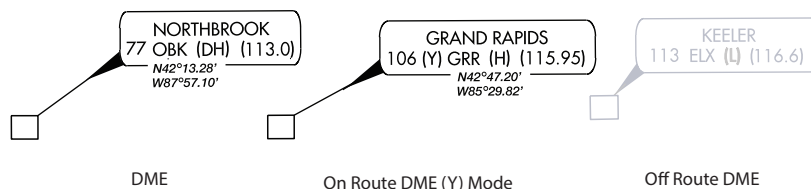
Figure 3.71 DME
