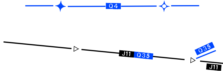
Figure 3.116 “Q” RNAV Routes
