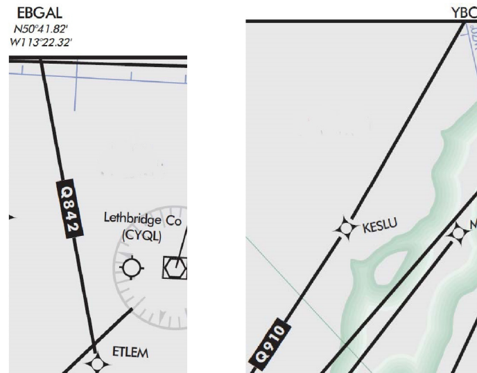
Figure 3.31 Airways/Routes Past Chart Boundary - External - Foreign RNAV Routes
