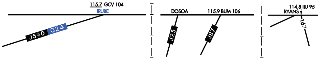
Figure 3.32 Placement of Next Point Information - Internal
