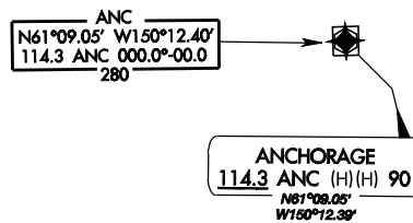
Figure 3.168 (AK) VOR/DME RNAV Collocated with NAVAID
