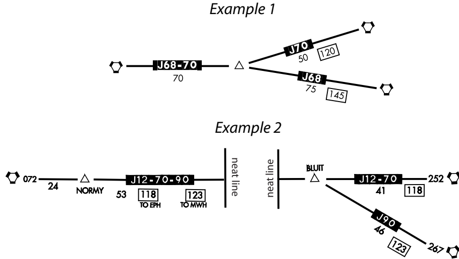
Figure 3.145 Box Mileages - Coincidental Routes & “TO” Notes
