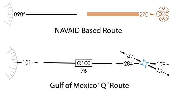
Figure 3.129 Radials and Bearings
