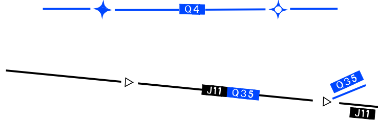
Figure 3.116 “Q” RNAV Routes
