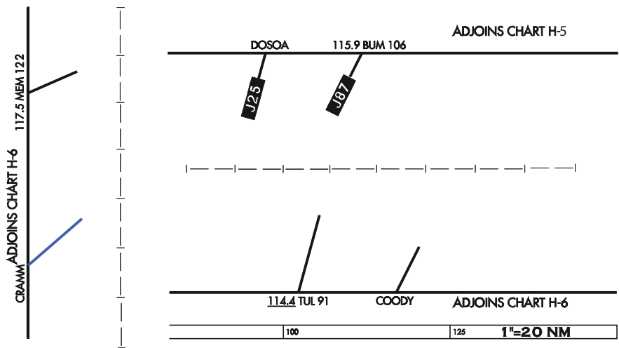
Figure 3.32 Margin Notes for Adjoining/Overlapping Charts
