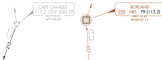
Figure 3.171 NAVAID Based-Off Route Holding Patterns - VHF/UHF & LF/MF
