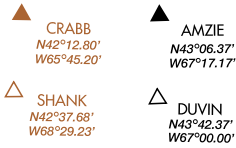
Figure 3.152 Radio Fix Geographic Coordinates
