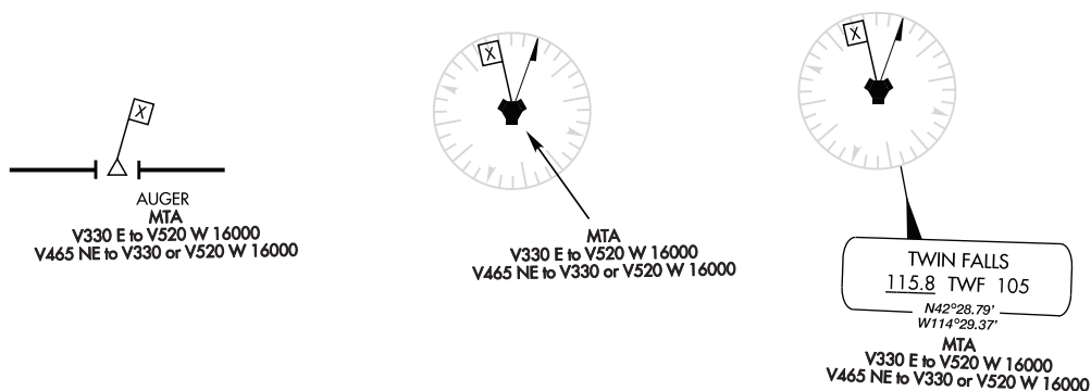
Figure 3.140 Minimum Crossing Altitudes (MCA) & Minimum Turning Altitude (MTA)
