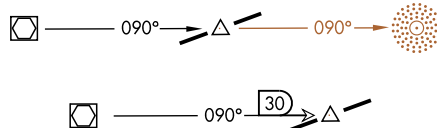
Figure 3.156 NAVAIDs Used for Fix Makeup
