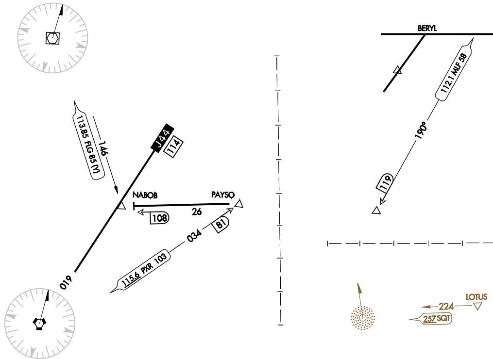
Figure 3.159 Facility Locator Boats
