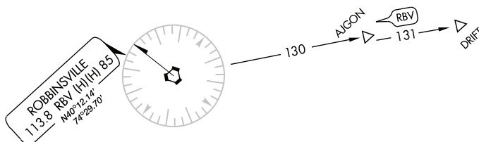
Figure 3.161 Facility Locator Boats in Congested Areas
