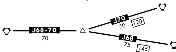
Figure 3.143 Box Mileages - Coincidental Routes & “TO” Notes
