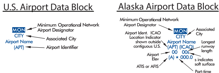
Figure 3.47 Airport Data Block
