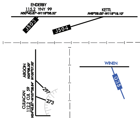
Figure 3.31 Placement of Next Point Information - External
