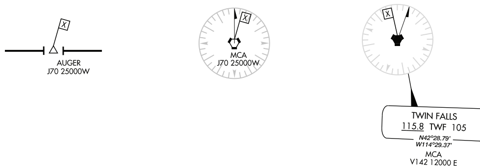
Figure 3.138 Minimum Crossing Altitudes (MCA)
