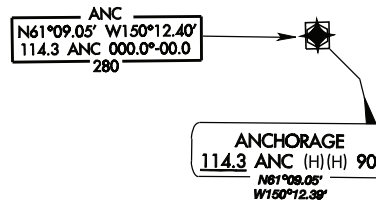
Figure 3.166 (AK) VOR/DME RNAV Collocated with NAVAID
