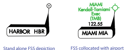
Figure 3.74 FSS Not Associated with a NAVAID
