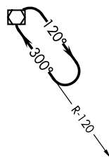
Figure 3.32 Non-RNAV Holding Patterns
