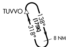
Figure 3.31 RNAV Holding Patterns
