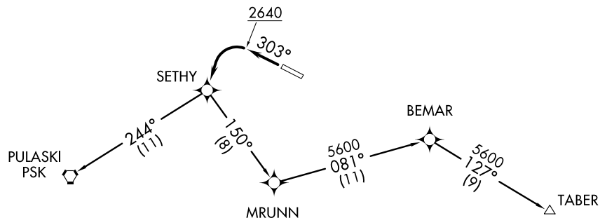
Figure 3.13 Waypoint Depiction
