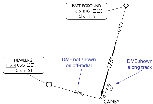
Figure 3.22 Off-Radial DME
