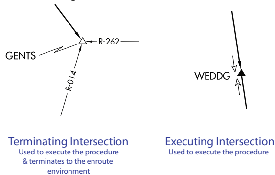
Figure 3.21 Intersections
