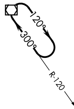
Figure 3.33 Non-RNAV Holding Patterns
