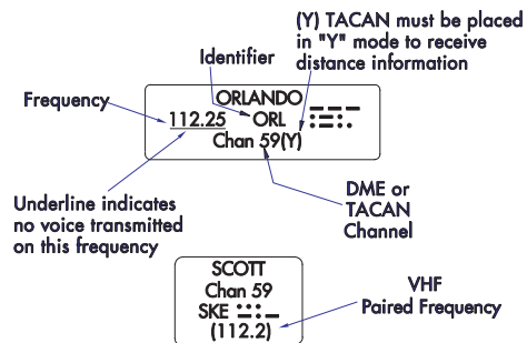
Figure 3.10 NAVAID Symbolization
