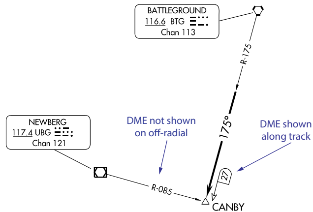
Figure 3.22 Off-Radial DME
